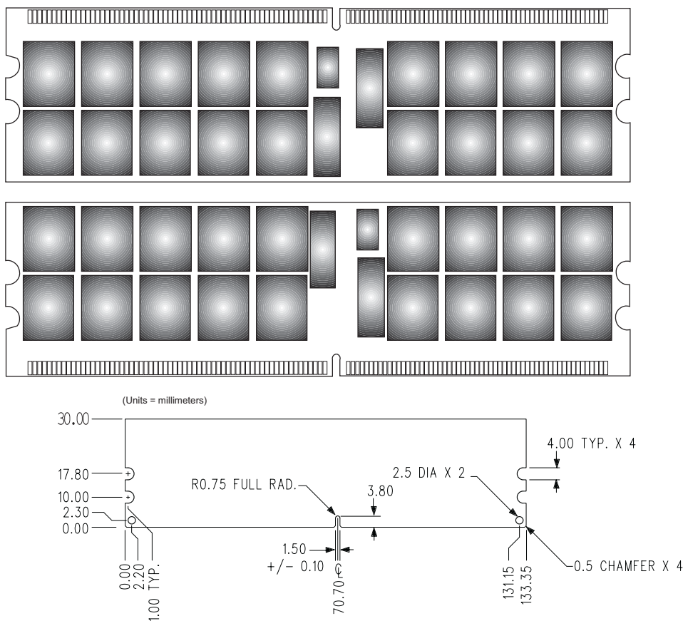
Figure 1: KVR533D2Q8R4K2/8G 240-Pin DIMM
