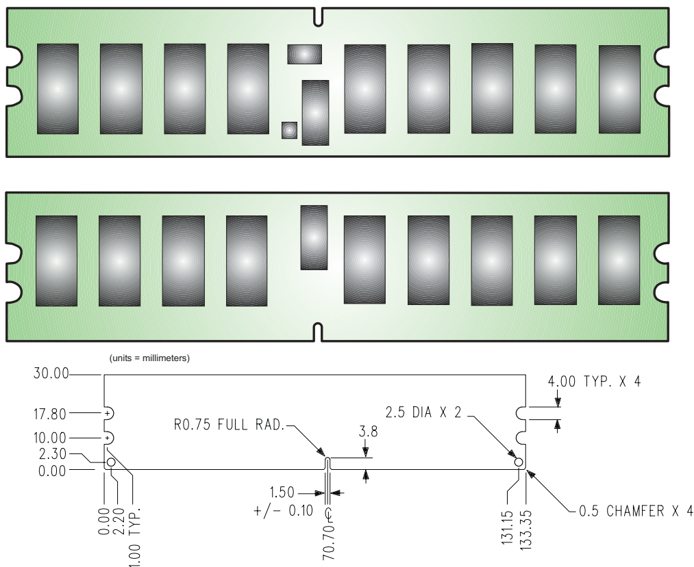
Figure 1: KVR667D2S4P5/1GI 240-Pin DIMM
