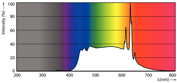
Spectral Power Distribution Colour - 5BA11/PER/UD50/CL/G/E26/D 6/3PF T20
