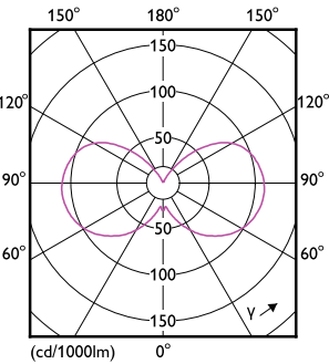
Light Distribution Diagram - 5BA11/PER/UD50/CL/G/E26/D 6/3PF T20
