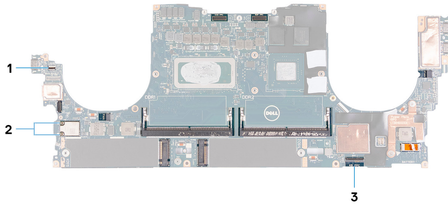
Figure 2. System-board connectors
