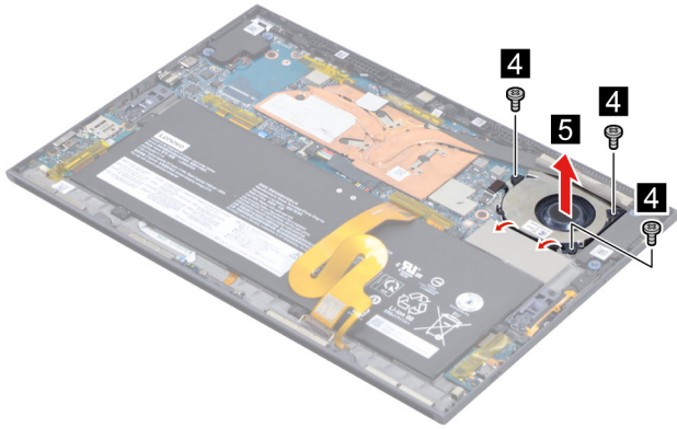
Figure 16. Remove the fan.
