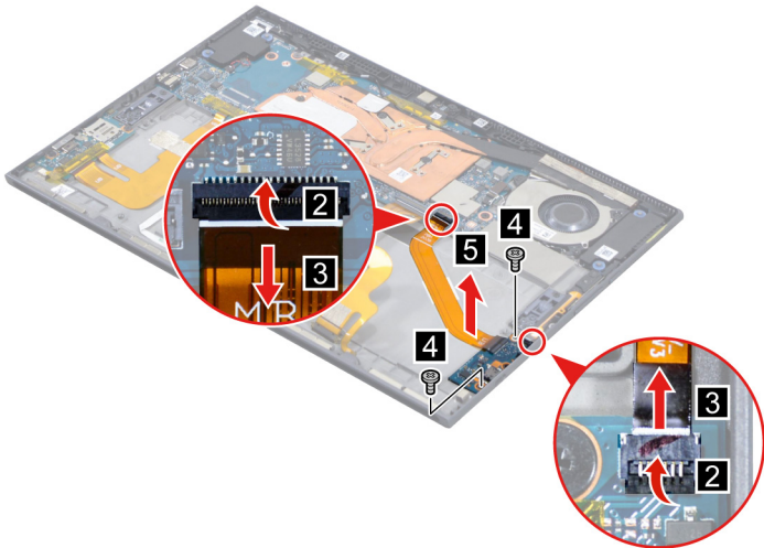
Figure 28. Detach two cable connectors and remove the function board module.
