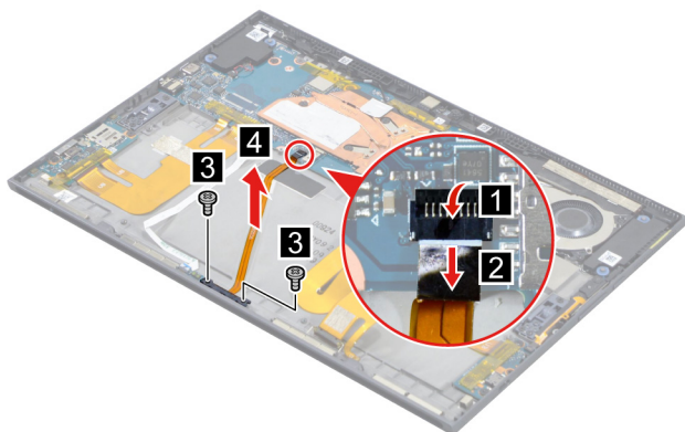
Figure 32. Disconnect the pogo pin cable from the system board and remove the pogo pin with cable.
