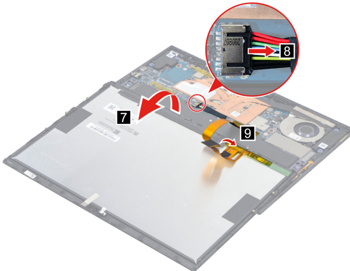
Figure 6. Rotate the LCD module and disconnect the battery pack cable from the system board. Peel off the tape.
