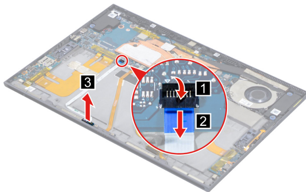
Figure 30. Disconnect the ToF cable from the system board and then remove the ToF board module.
