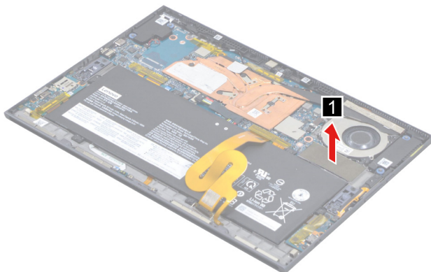
Figure 10. Peel off the tape.
