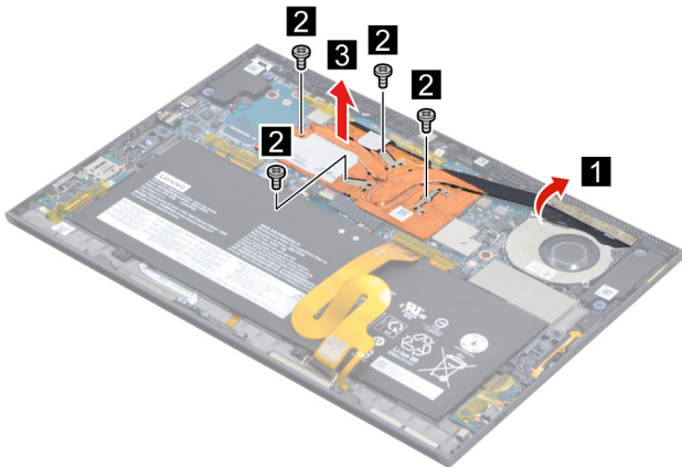
Figure 17. Remove four screws and then remove the heat sink
