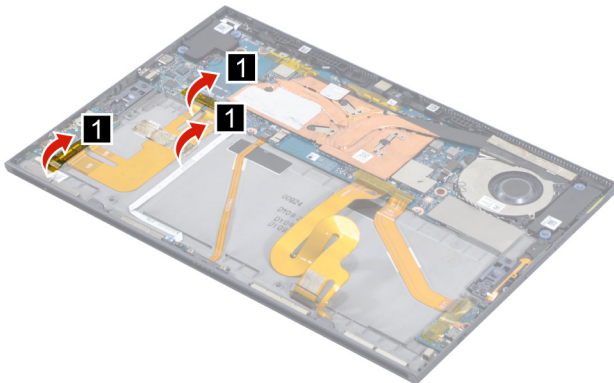
Figure 24. Peel off the three pieces of tape.
