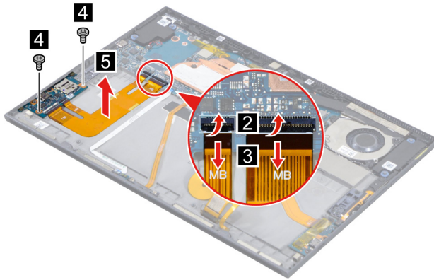
Figure 25. Remove the USB board module.
