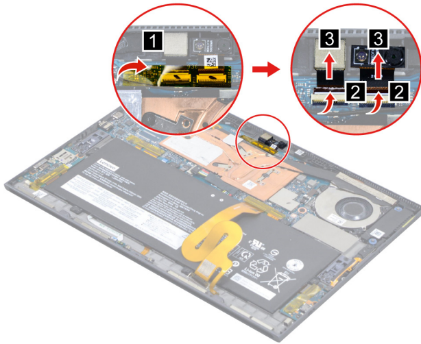
Figure 18. Remove the front camera and rear camera.
