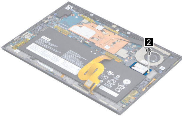
Figure 11. Remove one screw.
