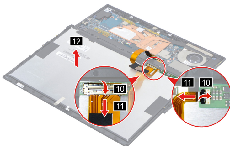
Figure 7. Disconnect the EDP cable from the LCD module and remove the LCD module.
