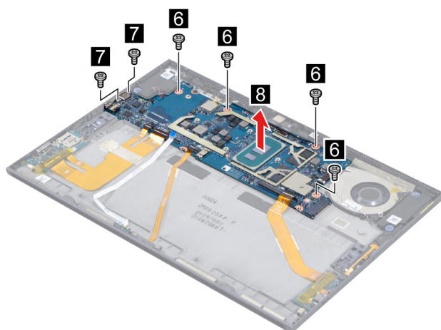
Figure 35. Remove the system board.
