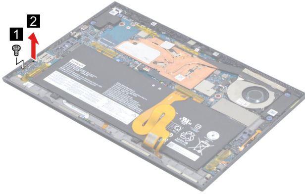
Figure 23. Remove the one screw and remove the I/O bracket.
