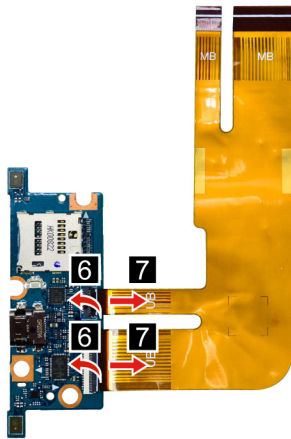
Figure 26. Separate the USB board cable from the USB board.
