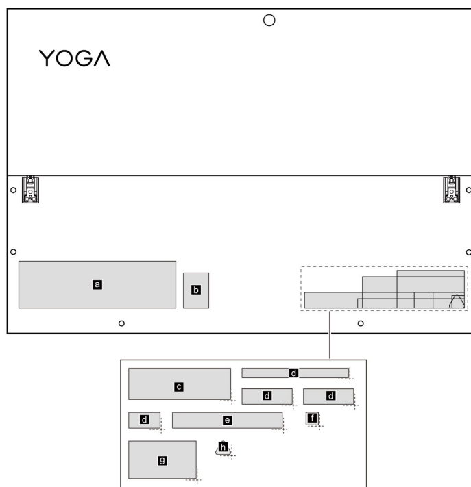
Figure 36. Label layout on the back side of the base cover
