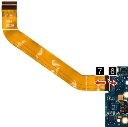
Figure 29. Separate the function board cable from the function board.
