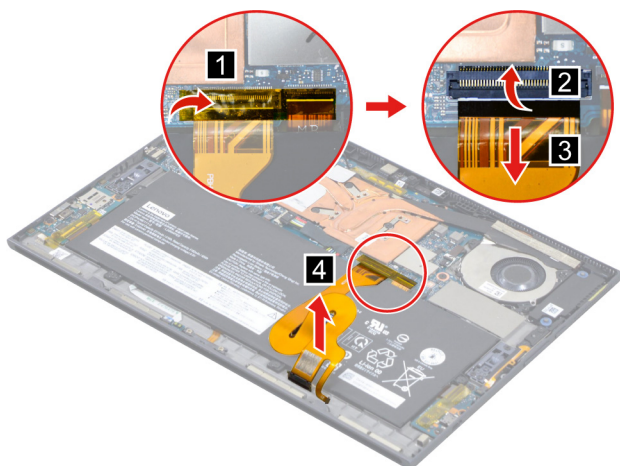
Figure 8. Remove the EDP cable.
