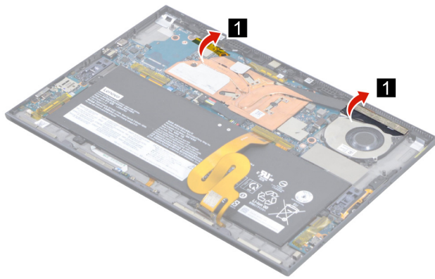
Figure 19. Peel off the two pieces of tape.
