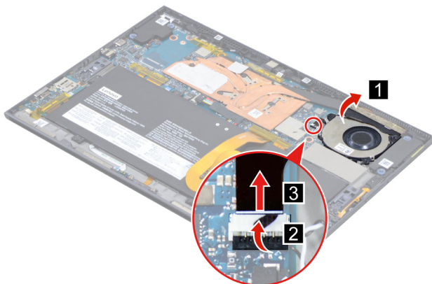
Figure 15. Peel off the tape and then disconnect the fan cable from the system board.
