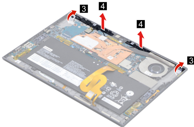
Figure 21. Peel off the tape on both sides. Remove the antenna module and LTE bracket.
