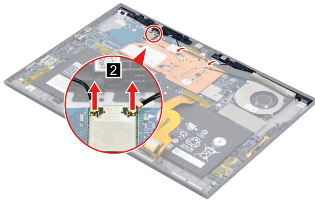
Figure 20. Detach the main and auxiliary antenna cable connectors and release the antenna cables.
