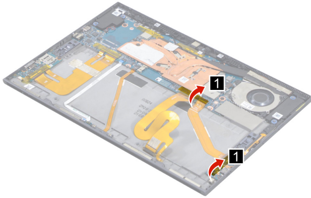
Figure 27. Peel off the two pieces of tape.
