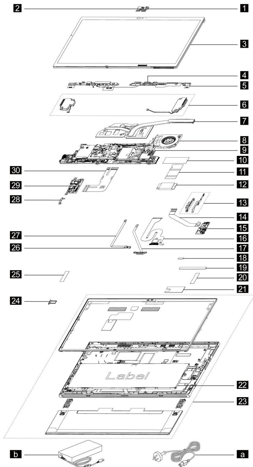
Figure 1. Yoga Duet 7 13ITL6 and Yoga Duet 7 13ITL6-LTE exploded view
