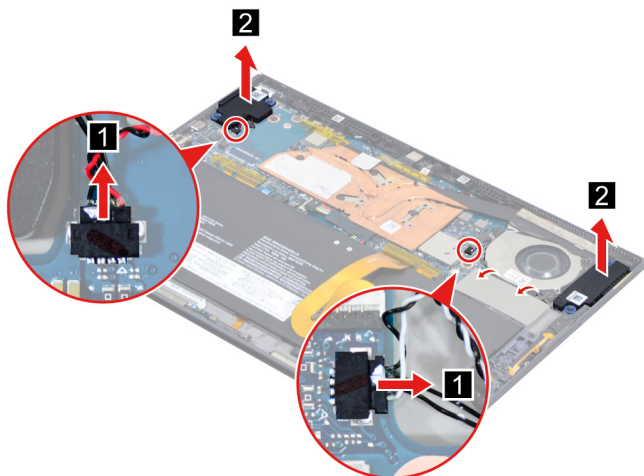
Figure 14. Remove the speakers.
