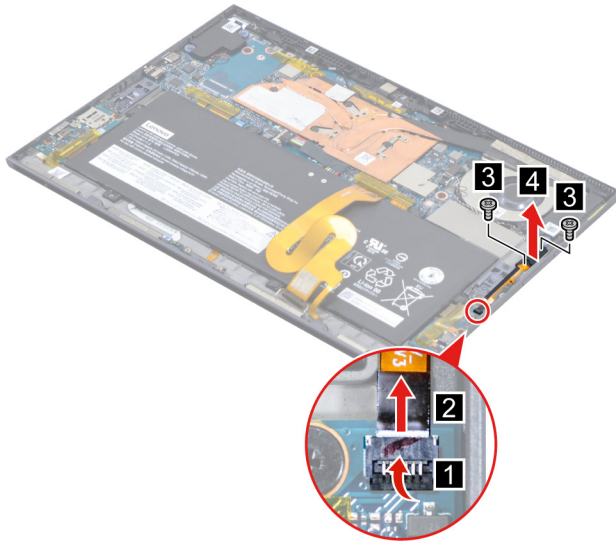
Figure 22. Remove the side switch module.
