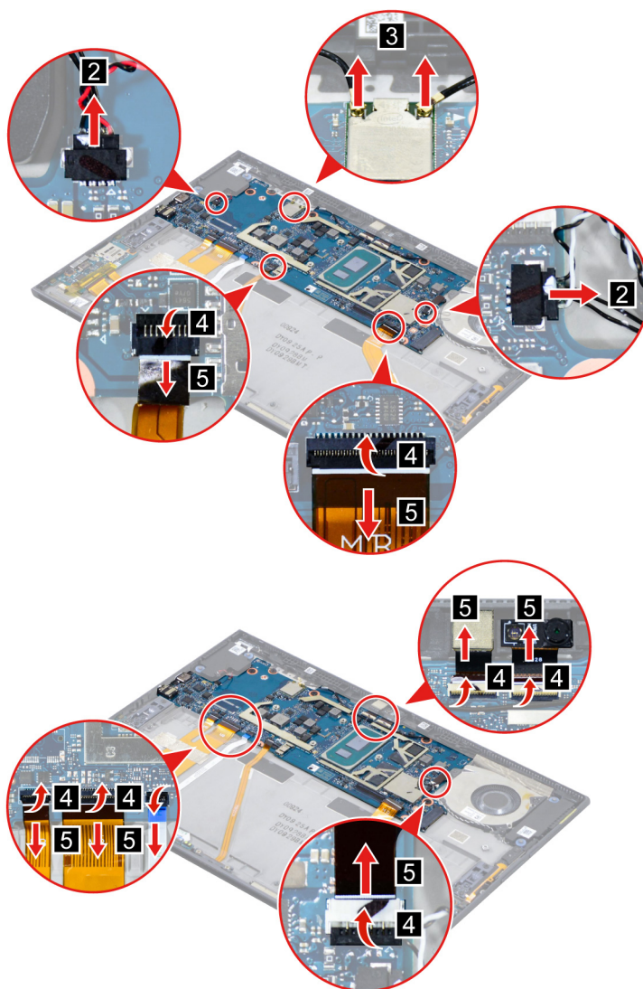
Figure 34. Disconnect cables connected to the system board.
