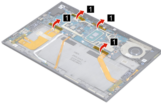
Figure 33. Peel off the four pieces of tape.
