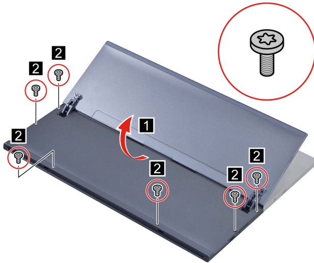
Figure 3. Open the kickstand and then remove six screws.
