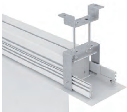
mounting kit for suspended ceilings
