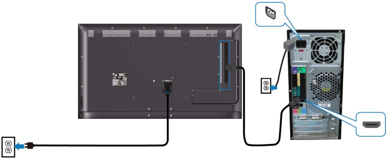
Connecting the DP cable
