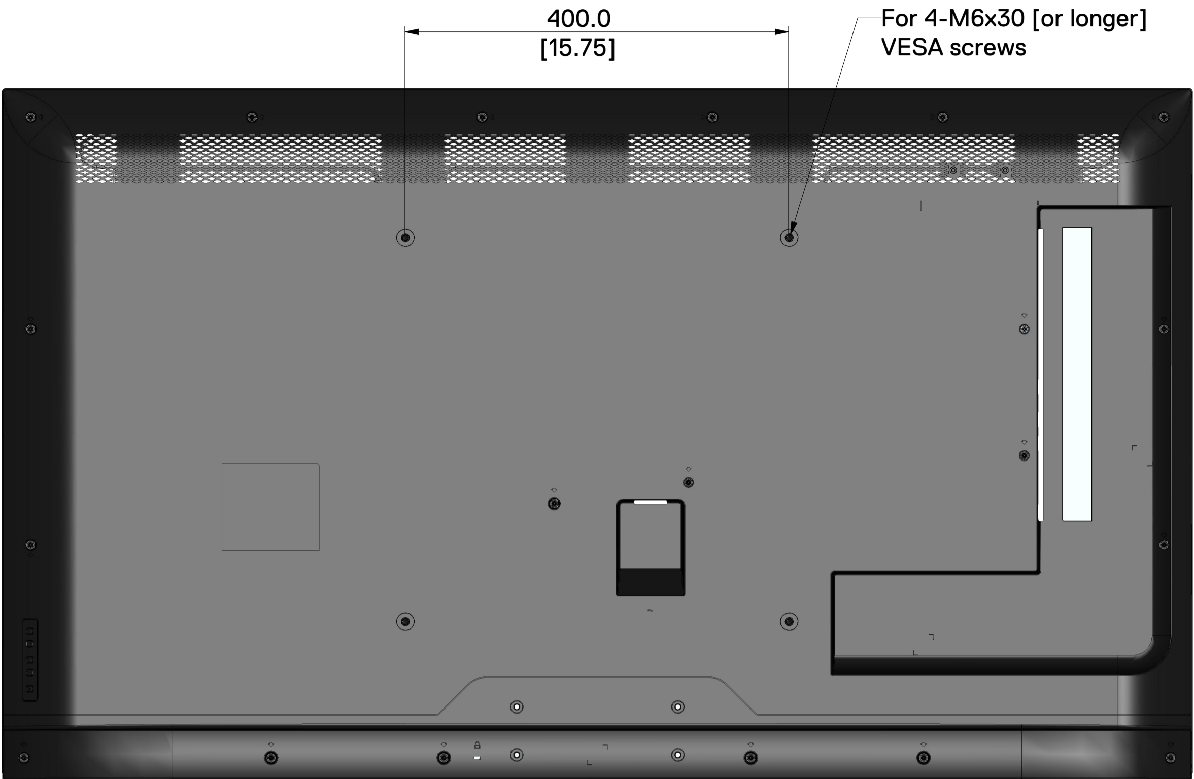
Back View of Monitor without Stand
