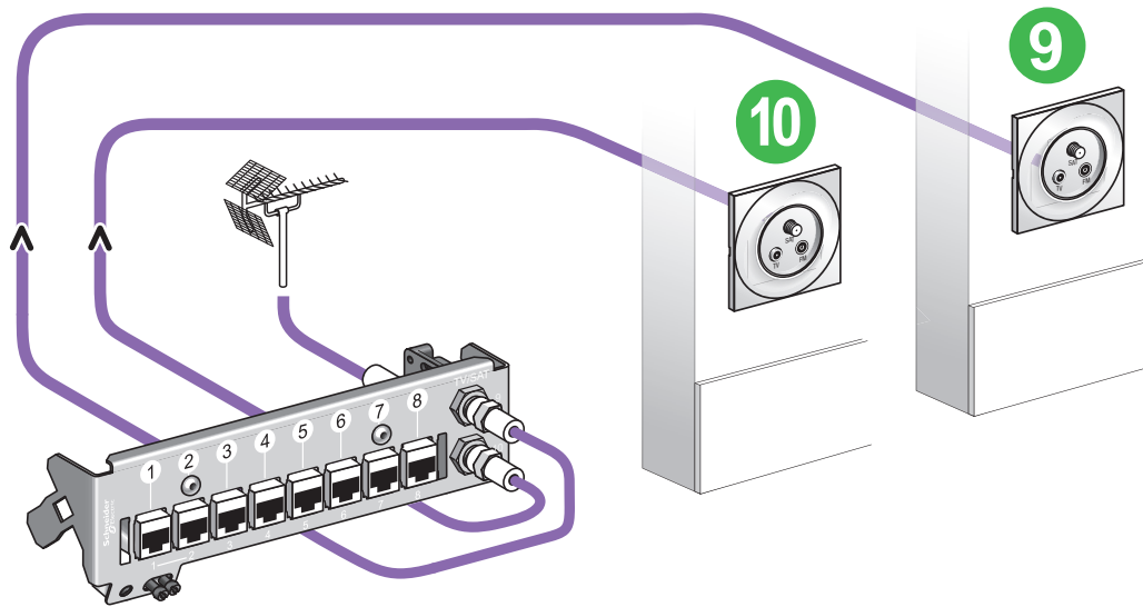
Câble coaxial
