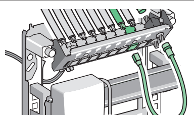
Raccordement TV
