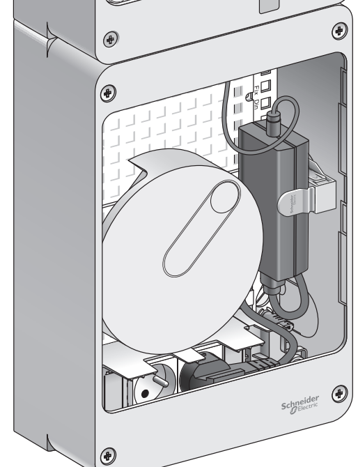
Coffret R9H13402VDIBOX
