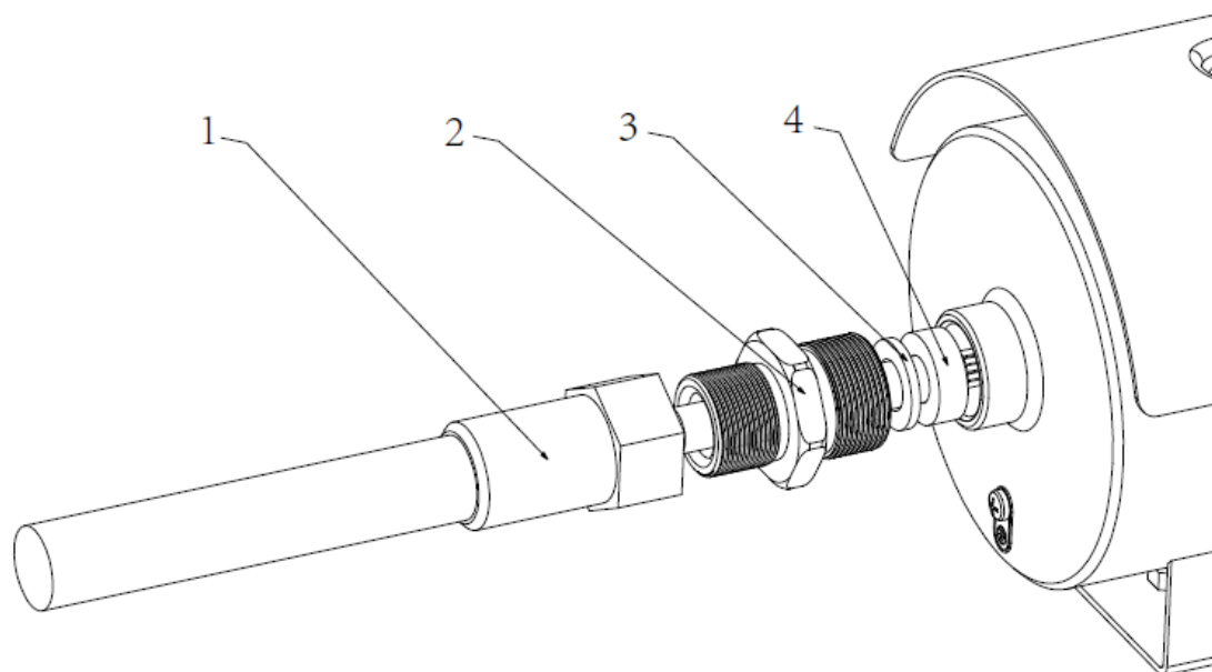
Figure 3-3 Connecting component (2)
