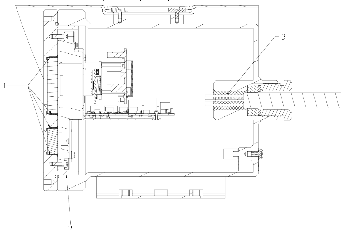
Figure 2-2 Explosion-proof structure
