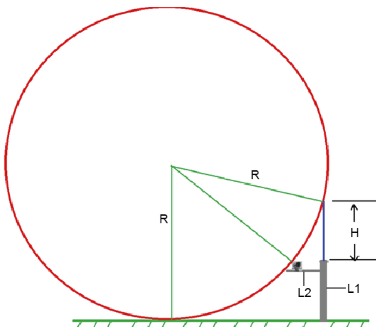
Appendix Figure 1-2 Install lightning protection devices (2)
