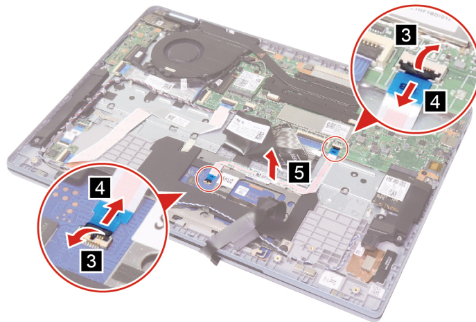
Figure 10. Disconnect and remove the touch pad cable
