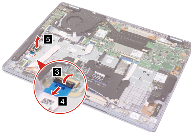
Figure 26. Disconnect the cable and remove the fingerprint reader board
