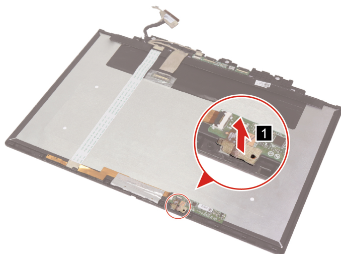
Figure 41. Peel off the acetate tape
