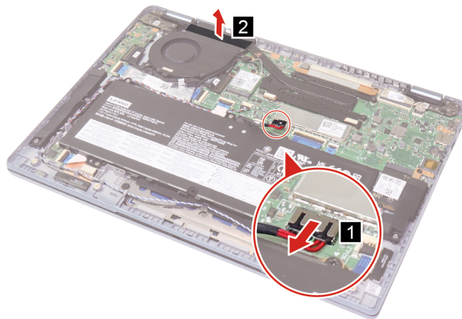
Figure 13. Disconnect the battery pack cable and peel off the tape
