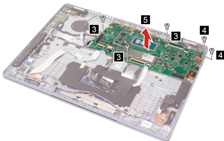
Figure 29. Remove five screws and the system board
