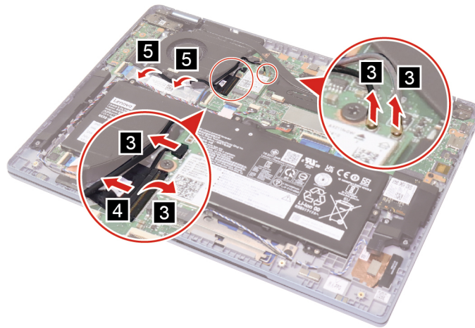
Figure 14. Disconnect cables
