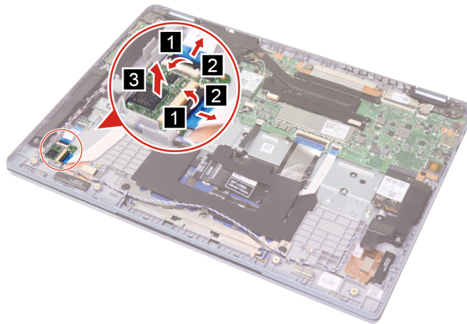
Figure 23. Disconnect cables and remove the MCU board
