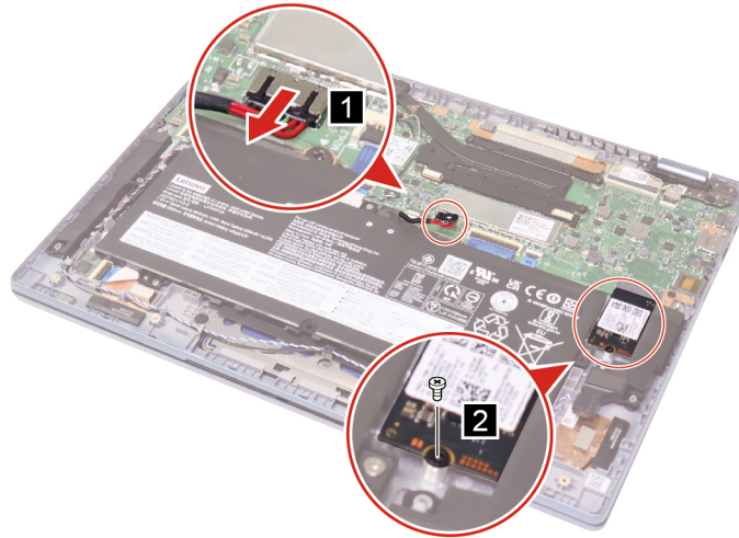
Figure 6. Disconnect the battery pack cable and remove one screw
