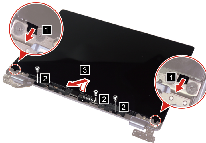
Figure 35. Remove three screws and the LCD module
