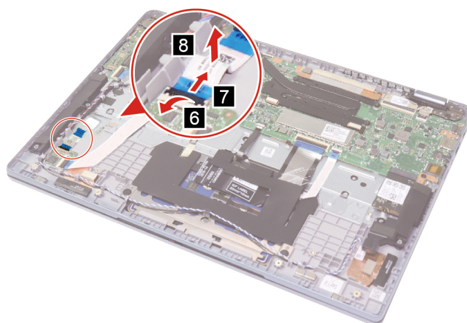
Figure 27. Disconnect and remove the fingerprint reader cable
