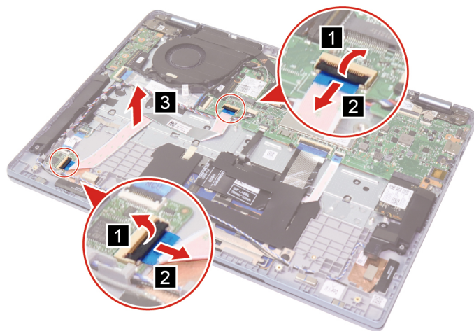
Figure 22. Disconnect and remove the MCU cable
