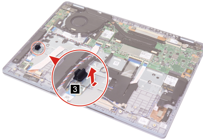
Figure 25. Remove the fingerprint reader bracket with rubber
