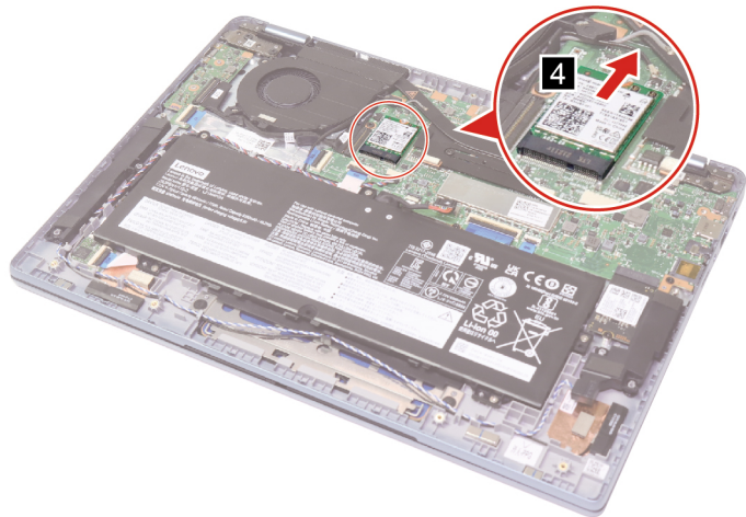
Figure 21. Remove the Wi-Fi card
