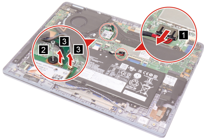
Figure 20. Disconnect cables and remove one screw
