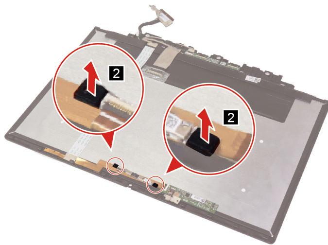
Figure 38. Remove the microphone rubbers
