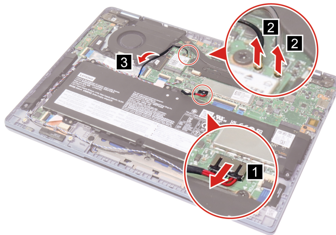
Figure 16. Disconnect the battery pack cable and the antenna cables
