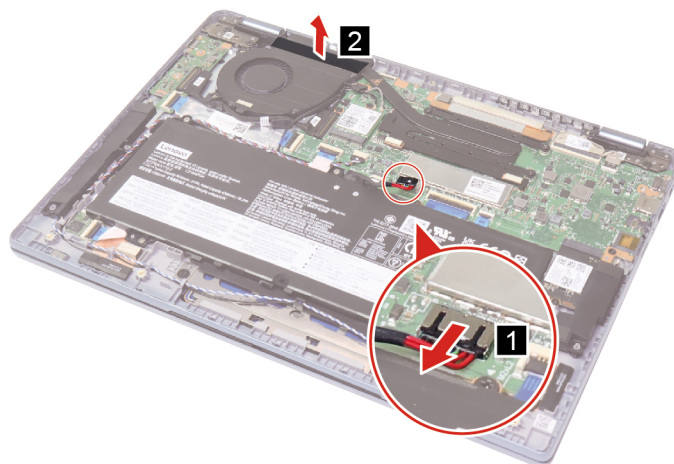
Figure 11. Disconnect the battery pack cable and peel off the tape
