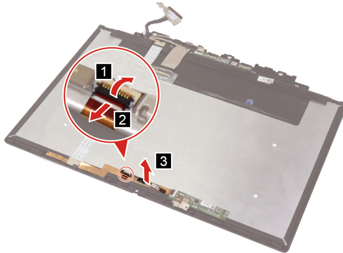
Figure 39. Remove the camera board
