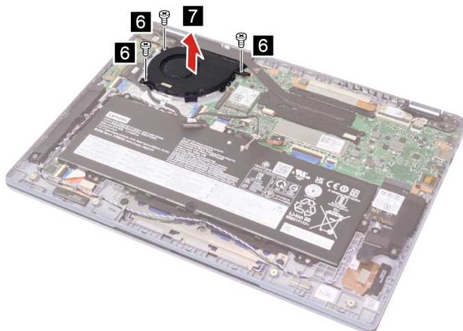
Figure 15. Remove three screws and the system fan
