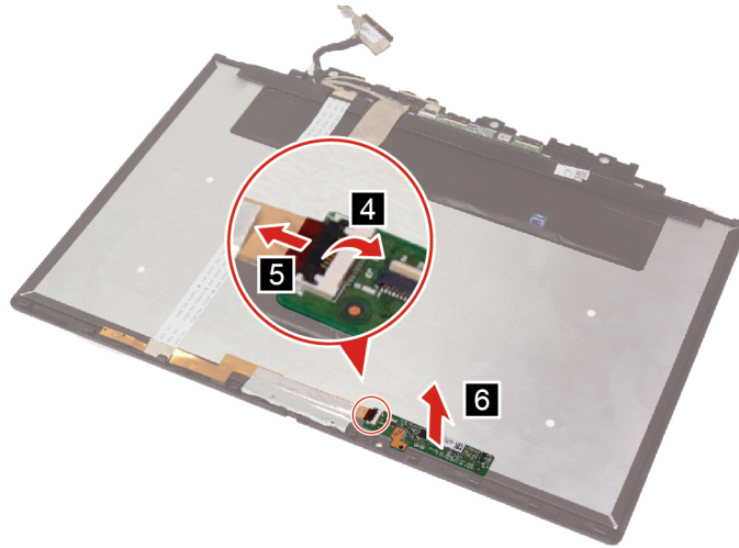
Figure 43. Disconnect the cable and remove the HPS board
