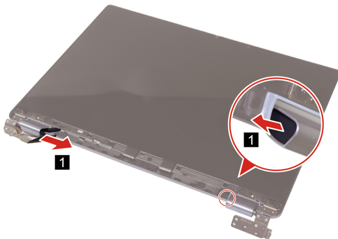
Figure 34. Remove hinge rubbers
