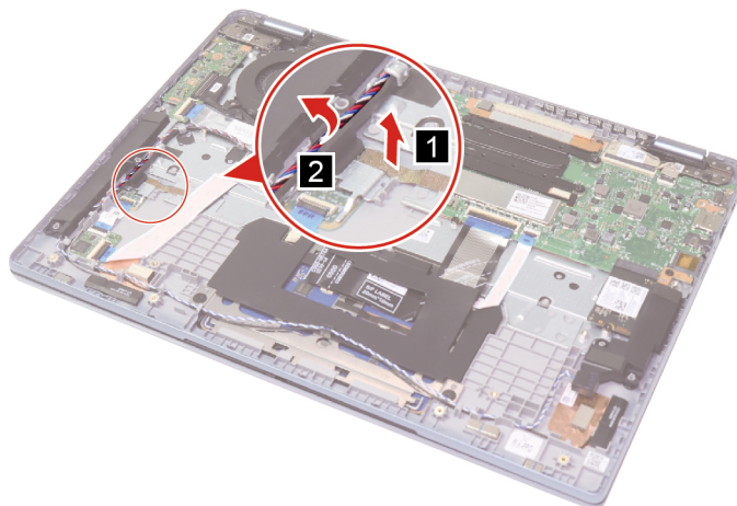
Figure 24. Peel off the tape and release the cable from the rubber
