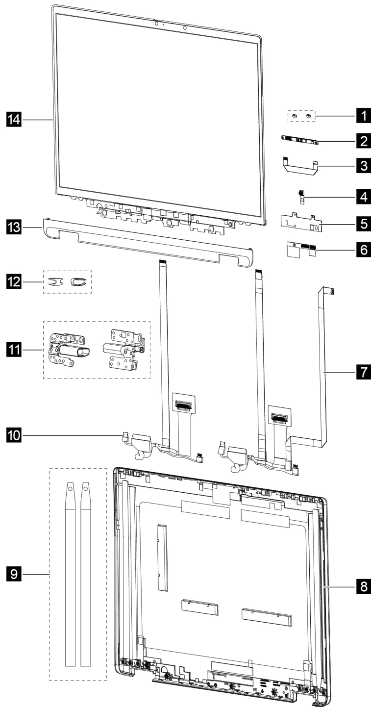
Figure 2. Exploded view of the LCD unit
