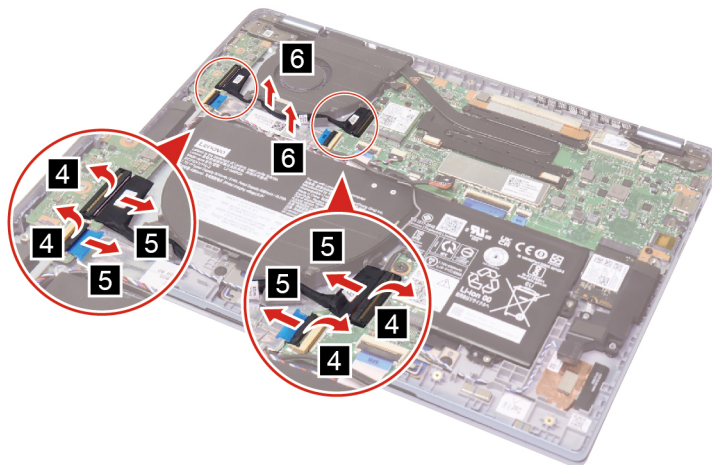
Figure 17. Disconnect and remove the I/O board cables
