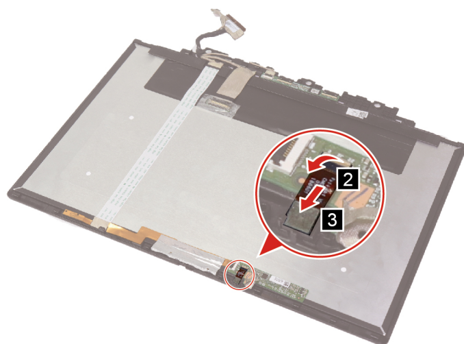
Figure 42. Disconnect the cable and remove the HPS camera
