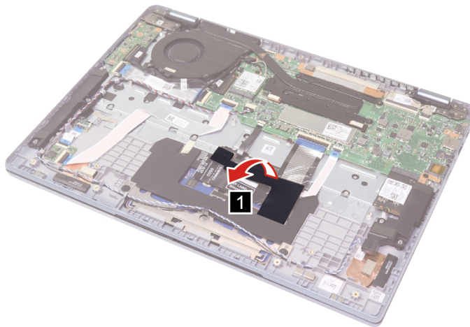
Figure 8. Peel back the rubber
