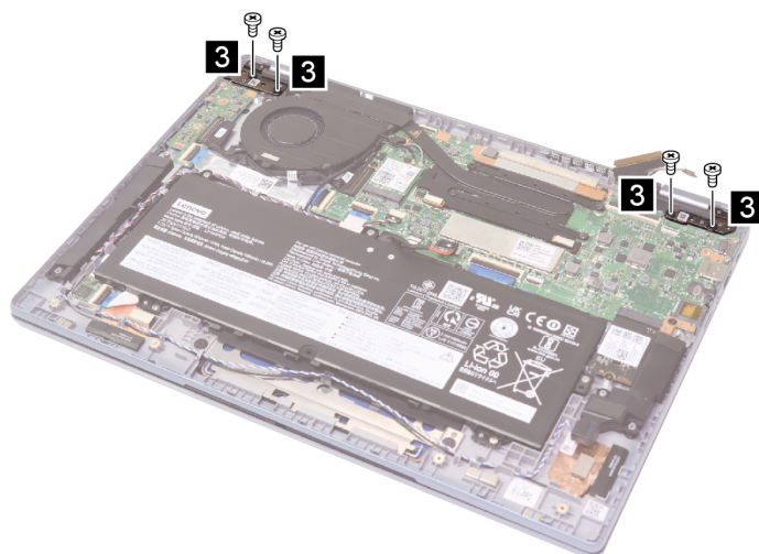
Figure 31. Remove four screws
