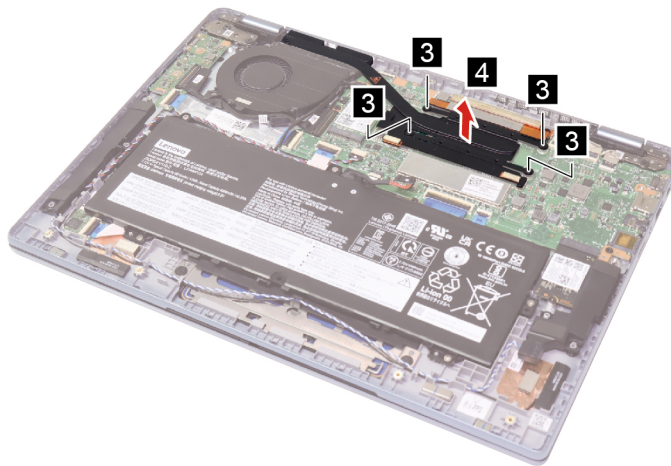
Figure 12. Loosen four screws and remove the heat sink
