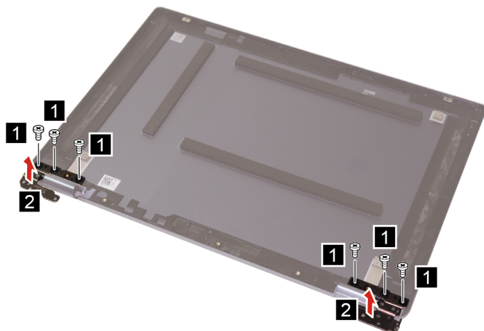
Figure 36. Remove six screws and the hinges
