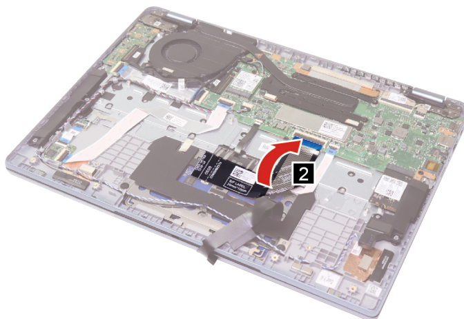
Figure 9. Peel back the keyboard cable
