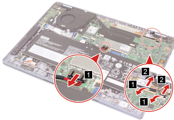
Figure 30. Disconnect the battery pack cable and EDP cable connectors
