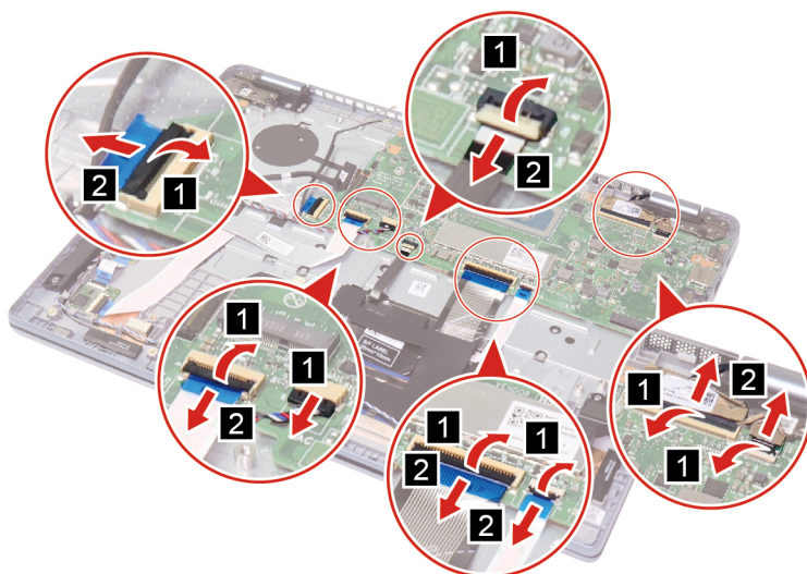
Figure 28. Disconnect all cables
