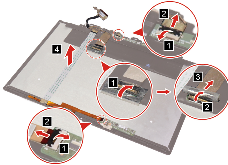
Figure 40. Disconnect all connectors and remove the EDP cable.
