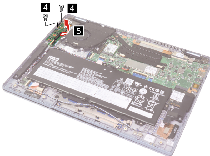
Figure 19. Remove three screws and the I/O board
