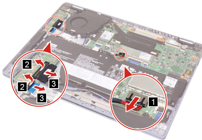
Figure 18. Disconnect the battery pack cable and the I/O board cables
