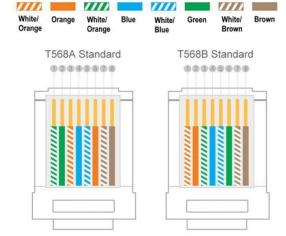
WIRING STRUCTURE
