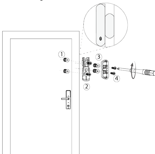
Figure 5-6 Drill holes
