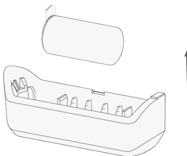
Figure 5-5 Take out the magnet
