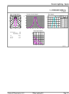
Accent Lighting Spots - MAS LEDspot VLE D 6-50W 940 PAR20 25D
