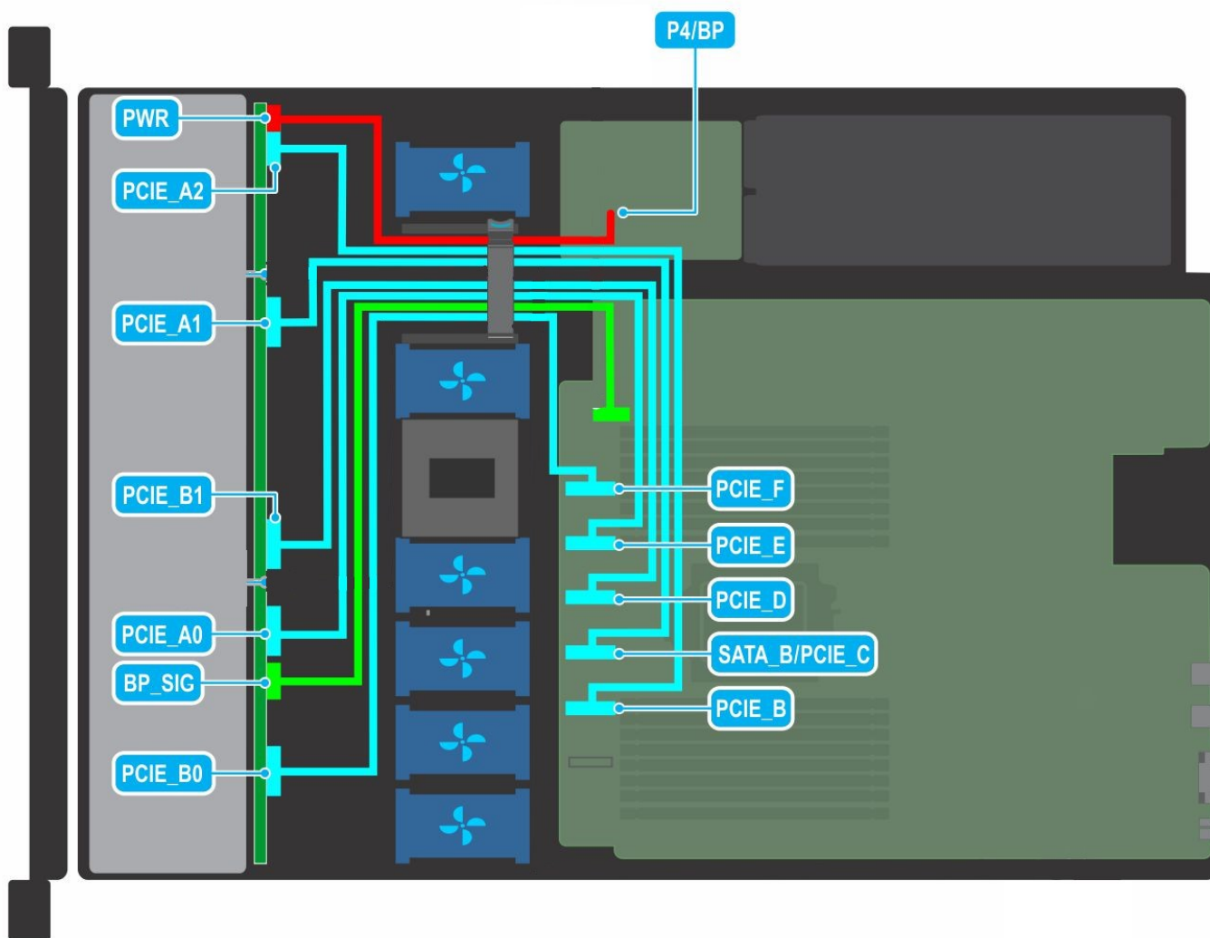
Figure 2. Cable routing - 10 x 2.5 inch NVMe drive backplane
