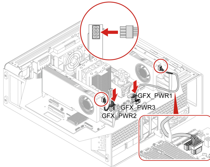
Figure 2. Cable connection for GTX RTX A4500/RTX A5500/RTX A6000
