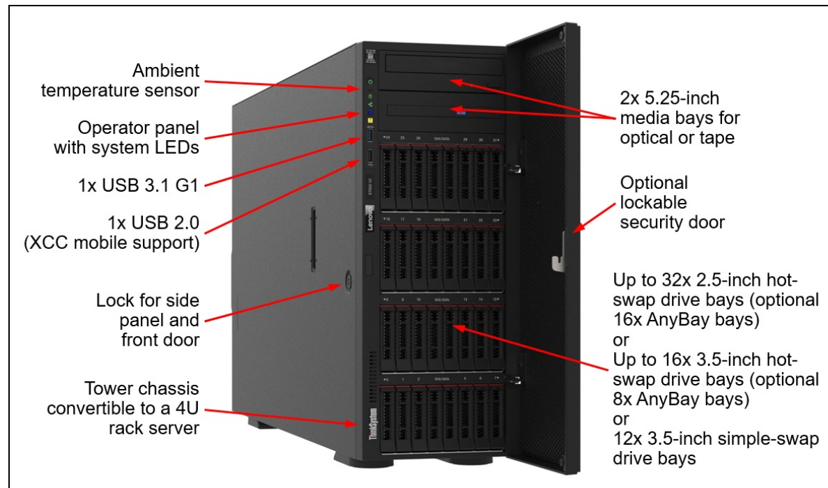
Figure 2. Front view of the ThinkSystem ST650 V2
