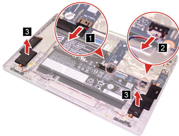
Figure 6. Remove the speakers
