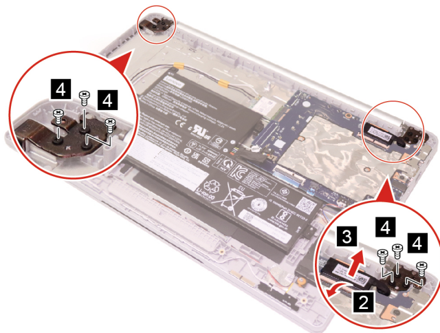
Figure 19. Disconnect the EDP cable, remove six screws and open the hinges
