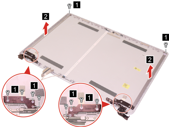
Figure 25. Remove the hinges
