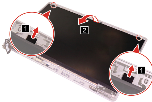
Figure 23. Pull out the removable tapes and lift the LCD panel
