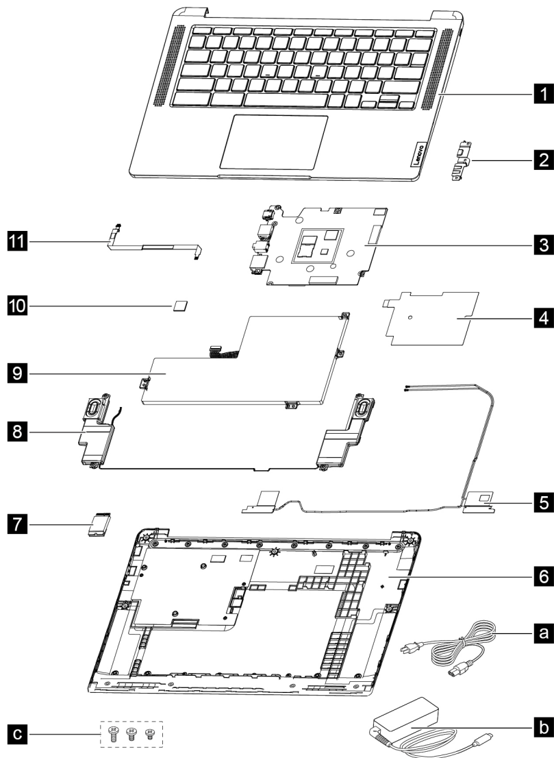
Figure 1. Exploded view - system
