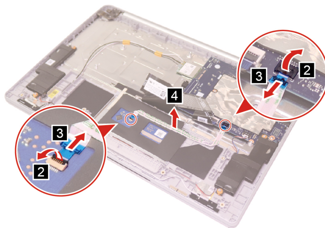
Figure 14. Remove touchpad cable
