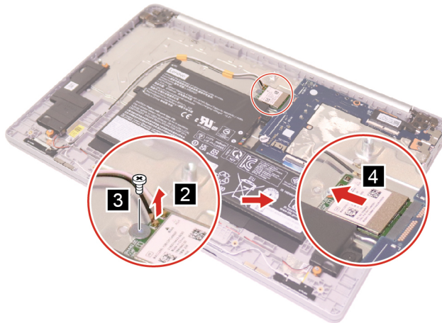
Figure 10. Remove the Wi-Fi card
