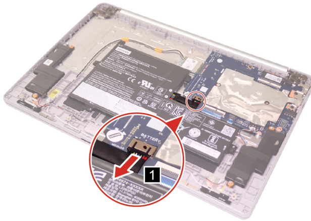
Figure 9. Disconnect the battery pack cable
