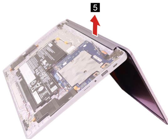
Figure 20. Remove the LCD unit
