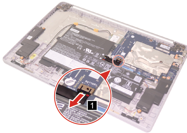
Figure 18. Disconnect the battery pack cable
