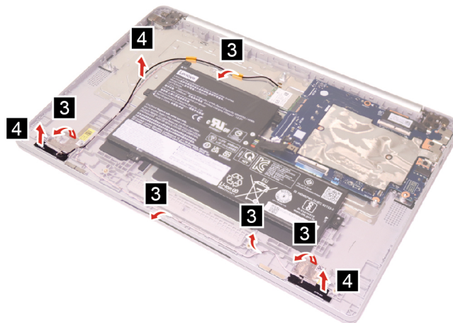
Figure 12. Peel off the foil and remove the Wi-Fi antennas
