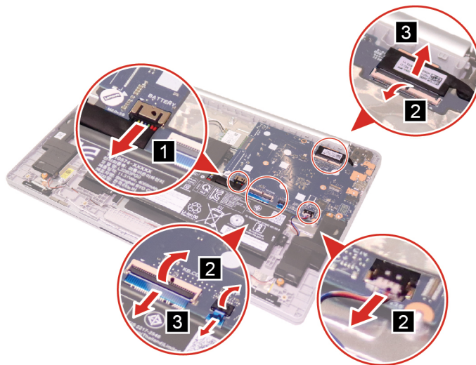
Figure 15. Disconnect cables
