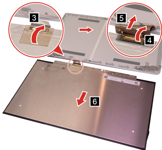
Figure 24. Disconnect the EDP cable and remove the LCD panel
