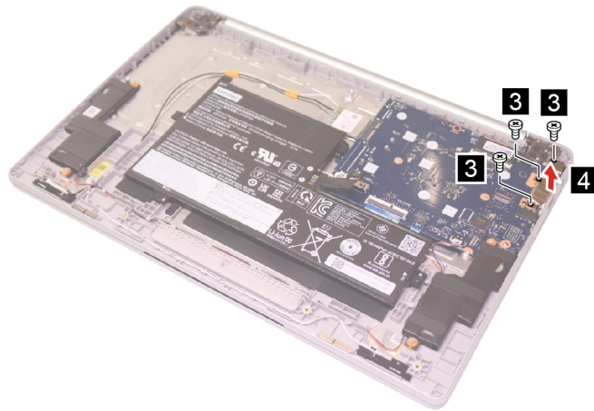
Figure 8. Remove the I/O bracket
