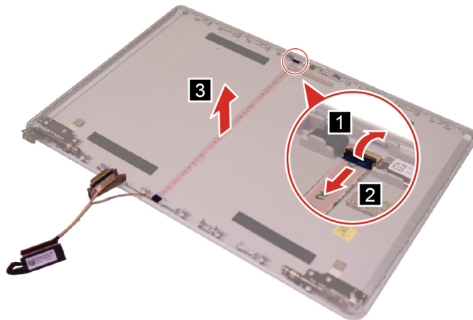
Figure 26. Remove the EDP cable
