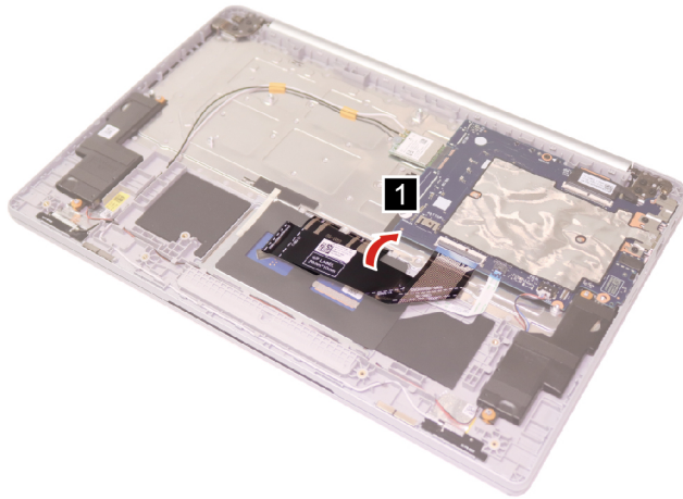
Figure 13. Turn over the keyboard cable
