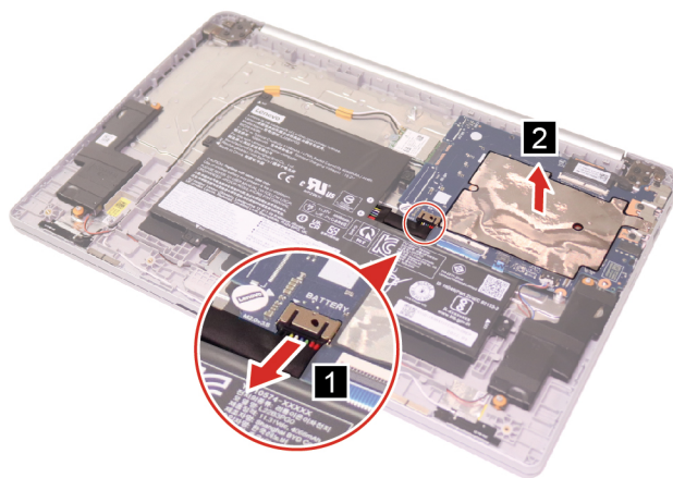
Figure 7. Disconnect the battery pack cable and remove the system board foil
