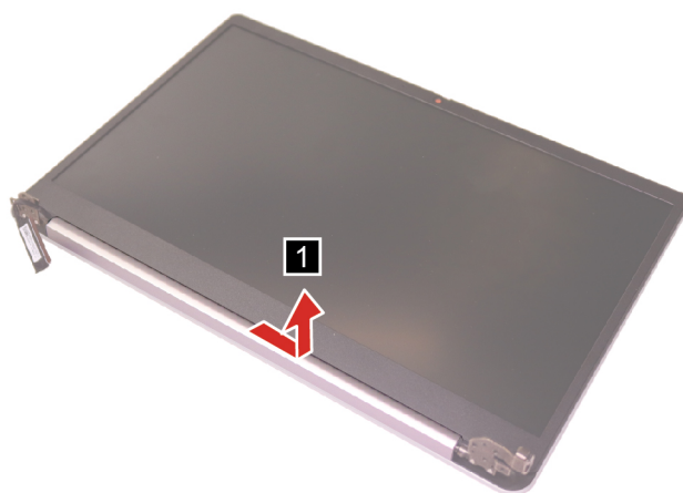
Figure 21. Remove the hinge cover
