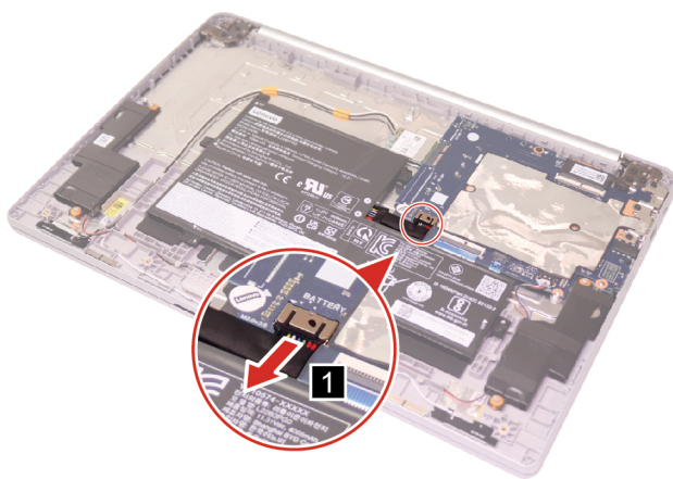
Figure 4. Disconnect the battery pack cable
