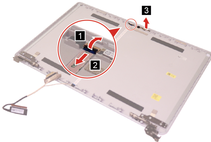
Figure 28. Disconnect the EDP cable and remove the camera board
