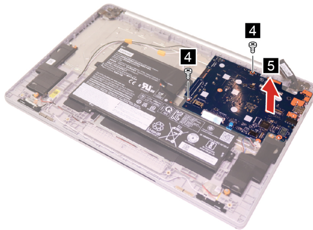
Figure 16. Remove two screws and then remove the system board
