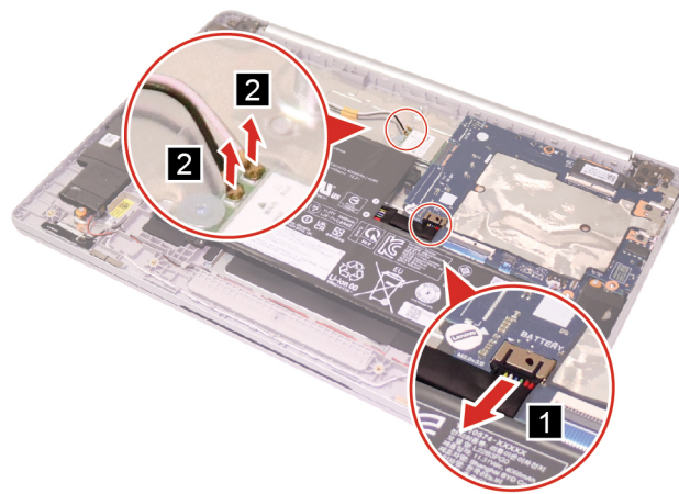
Figure 11. Disconnect the battery pack cable and the Wi-Fi antennas
