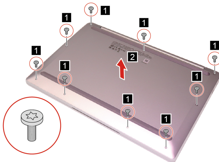
Figure 3. Remove the lower case
