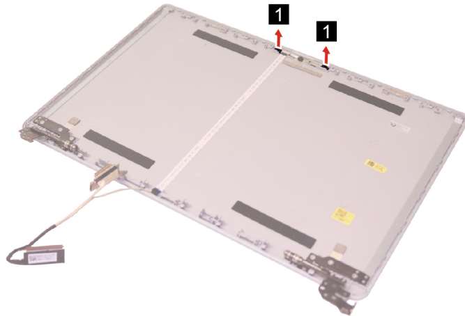
Figure 27. Remove the microphone rubbers
