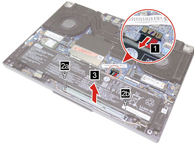
Figure 12. Remove the touchpad bracket
