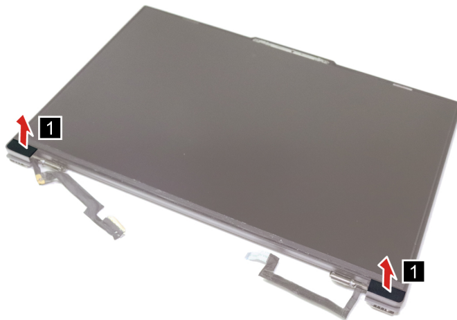
Figure 32. Remove the tapes
