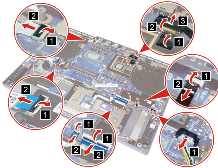
Figure 21. Disconnect cables
