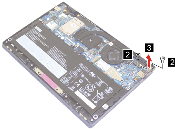
Figure 19. Remove the Type-C bracket
