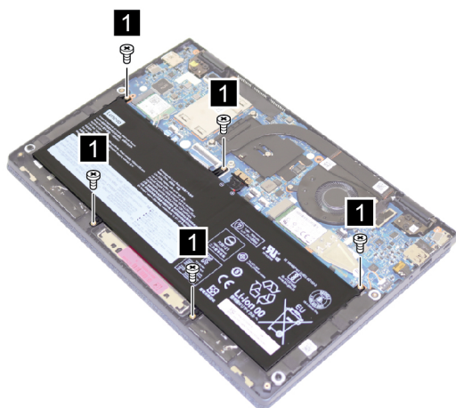
Figure 5. Remove five screws
