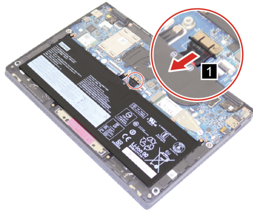
Figure 7. Disconnect the battery pack cable
