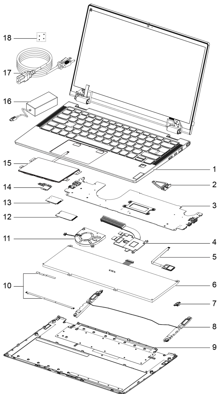
Figure 1. Yoga 6 13ALC6 exploded view
