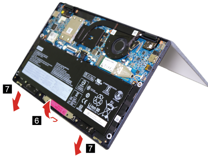
Figure 33. Remove the upper case assembly
