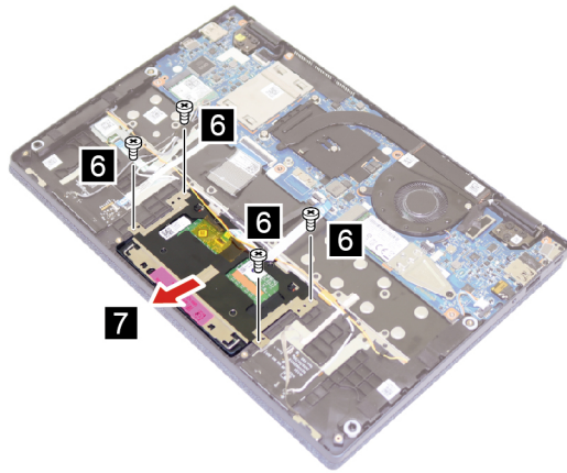
Figure 22. Remove the touchpad
