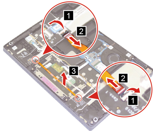
Figure 25. Remove the antenna cable
