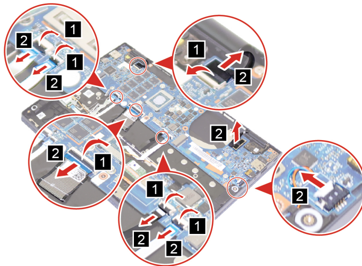
Figure 28. Disconnect cables
