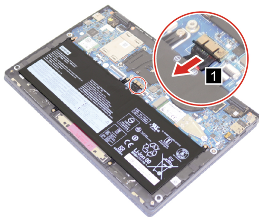
Figure 13. Disconnect the battery pack cable
