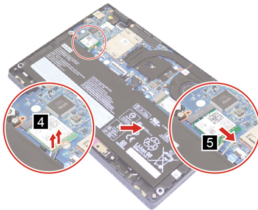
Figure 12. Remove the Wi-Fi card
