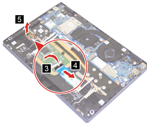
Figure 24. Remove the fingerprint sensor
