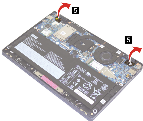
Figure 32. Open the hinges
