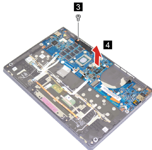
Figure 29. Remove the system board
