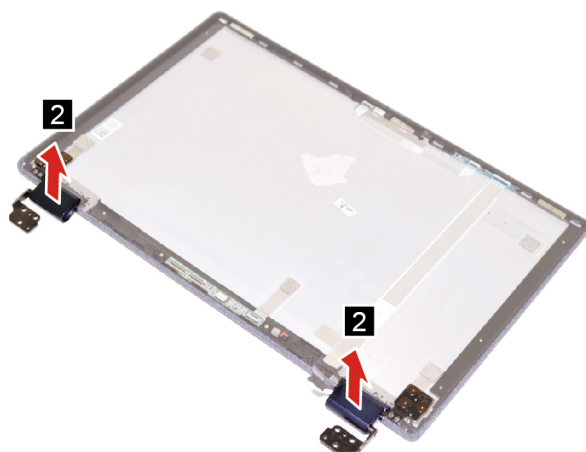
Figure 45. Remove the hinges
