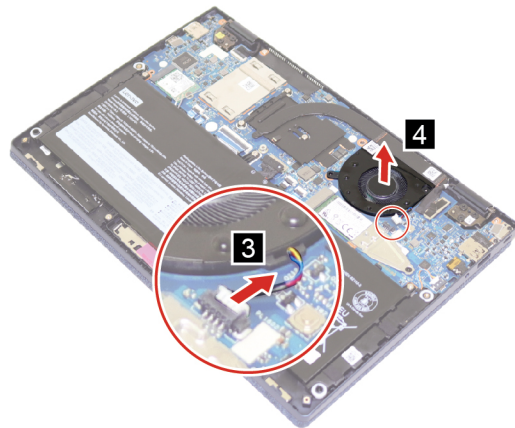
Figure 15. Remove the system fan
