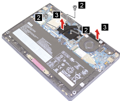
Figure 17. Remove the heatsink
