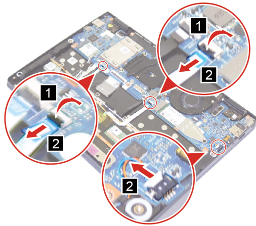
Figure 26. Disconnect the speakers cable
