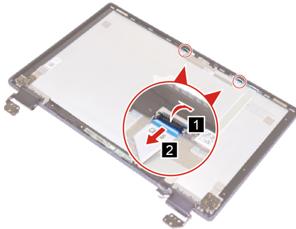
Figure 42. Disconnect the camera cable
