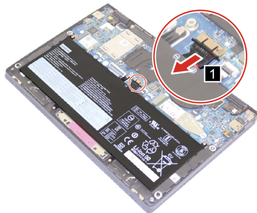
Figure 18. Disconnect the battery cable
