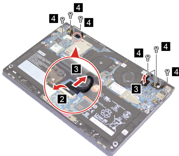
Figure 31. Disconnect cables and remove six screws
