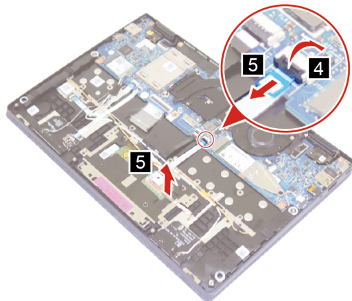
Figure 21. Remove the touchpad cable
