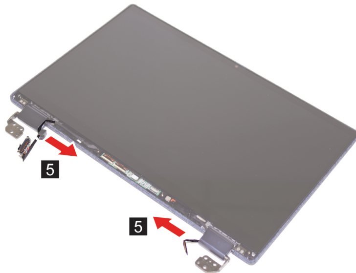
Figure 39. Pull out two LCD panel cables
