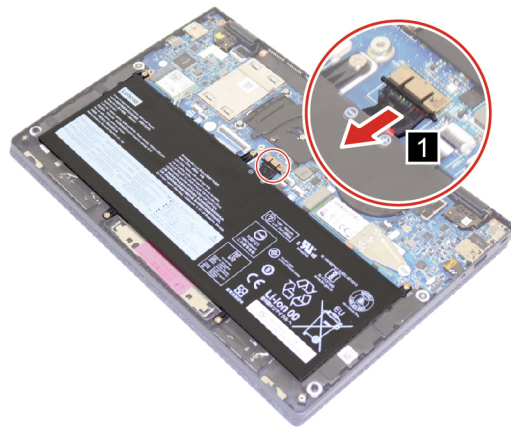
Figure 10. Disconnect the battery pack cable
