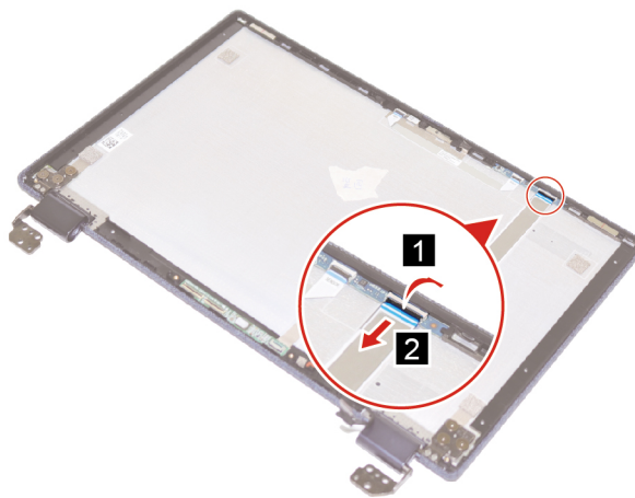
Figure 40. Disconnect the sensor board cable
