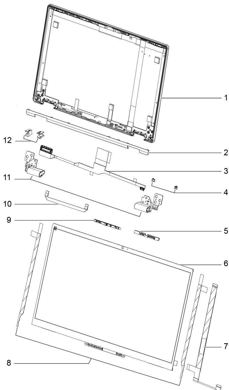
Figure 2. Yoga 6 13ALC6 LCD exploded view
