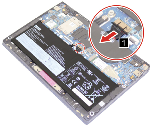
Figure 16. Disconnect the battery pack cable
