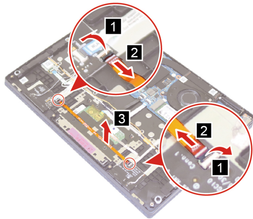
Figure 20. Remove the antenna cable
