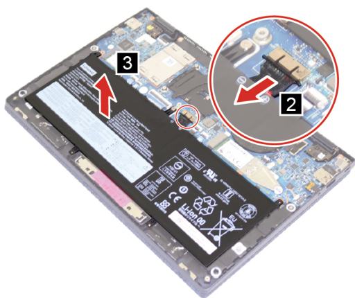
Figure 6. Remove the battery pack
