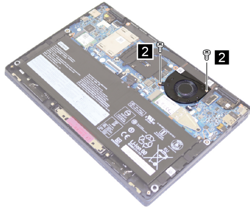
Figure 14. Remove two screws
