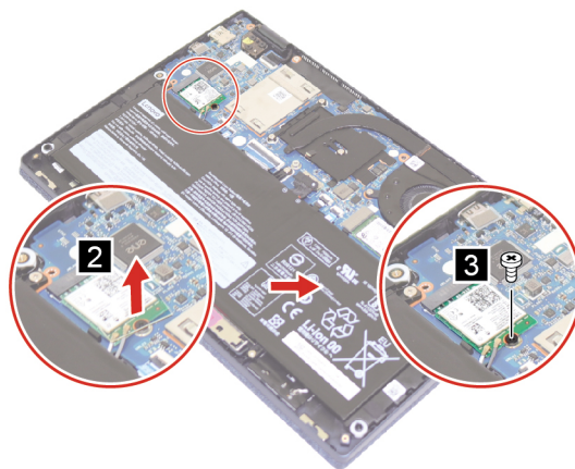
Figure 11. Remove the Wi-Fi card mylar and one screw
