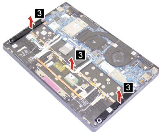
Figure 27. Remove the speakers
