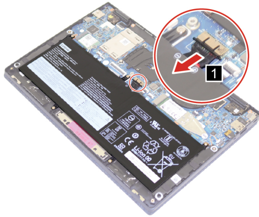
Figure 30. Disconnect the battery pack cable
