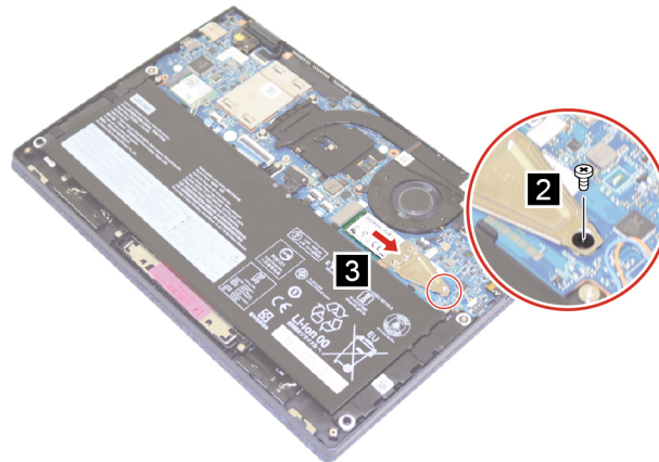
Figure 8. Remove the M.2 solid-state drive
