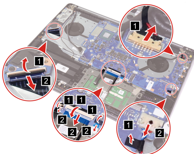
Figure 33. Disconnect cables
