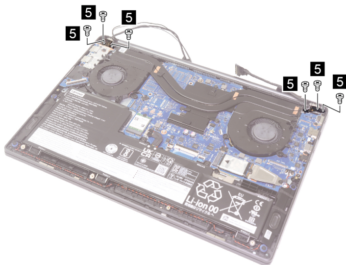
Figure 39. Remove six screws (for AMD UMA models)
