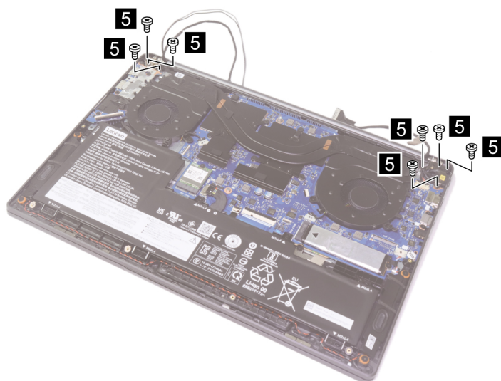
Figure 40. Remove seven screws (for Intel DIS models)
