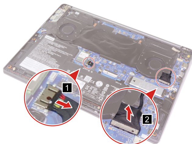
Figure 23. Disconnect battery pack cable and EDP cable
