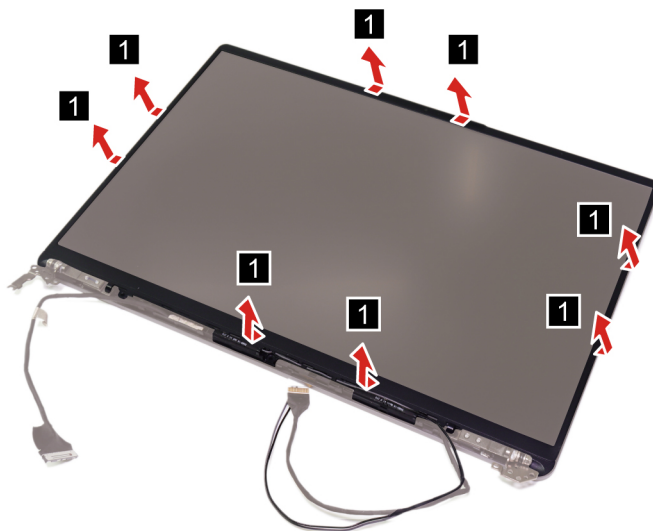
Figure 44. Remove the LCD bezel
