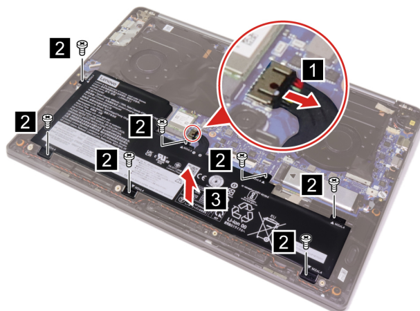
Figure 5. Disconnect the battery pack cable and remove seven screws and the battery pack
