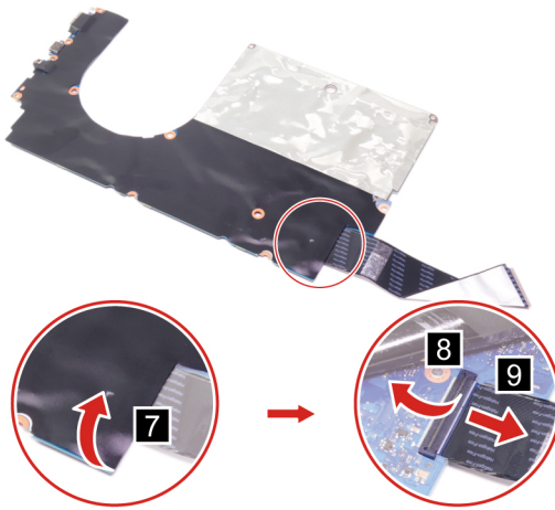
Figure 36. Peel back the system board mylar, disconnect the USB board cable and remove the USB board cable
