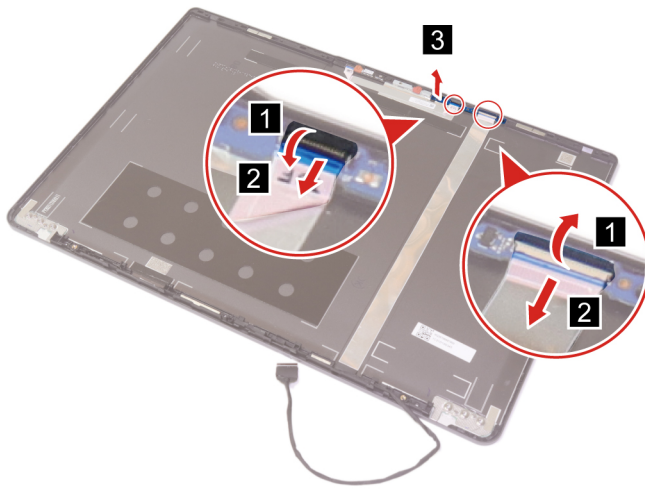
Figure 51. Disconnect the D-Mic cable and camera cable and remove the sensor board
