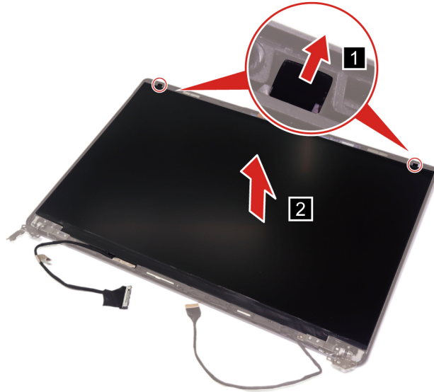
Figure 46. Pull out the removable tapes and lift the LCD panel.
