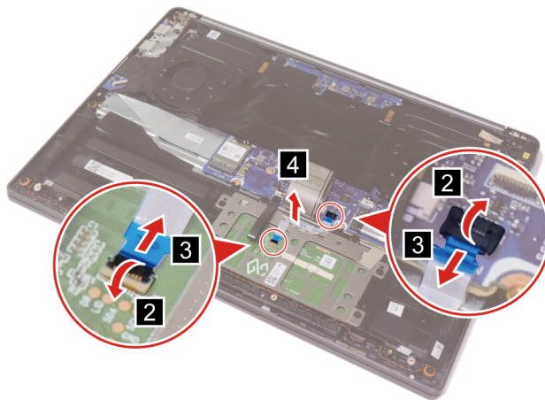
Figure 29. Disconnect the touch pad cable connectors and remove the touch pad cable
