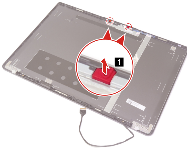
Figure 49. Remove the microphone rubbers
