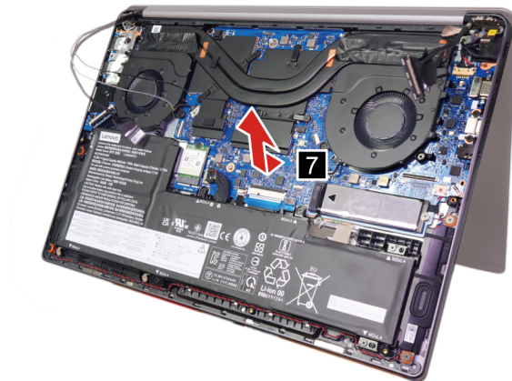
Figure 42. Remove the upper case assembly
