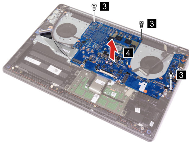
Figure 31. Remove three screws and the system board.
