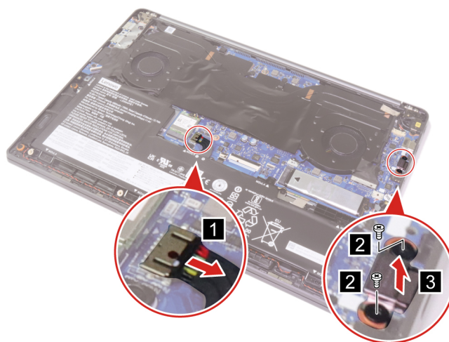
Figure 26. Disconnect the battery pack cable and then remove two screws and the lower I/O bracket
