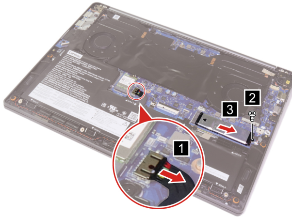
Figure 6. Disconnect the battery pack cable and remove one screw and the solid-state drive
