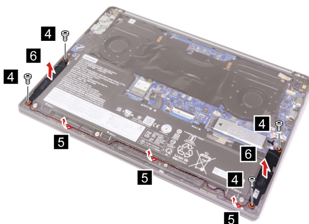
Figure 21. Remove four screws, pull out the speakers cable carefully and remove speakers
