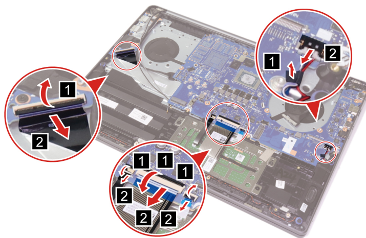
Figure 30. Disconnect cables
