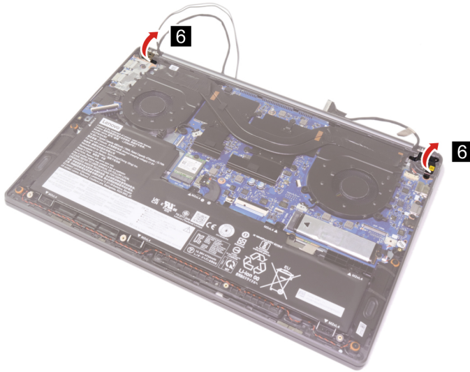
Figure 41. Open the hinge for about 90 degree
