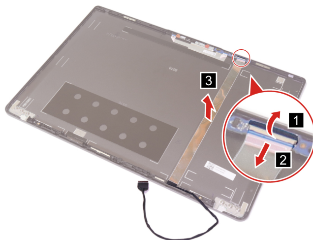
Figure 52. Disconnect the camera cable from the sensor board and remove the camera cable
