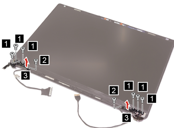
Figure 45. Remove eight screws and hinges
