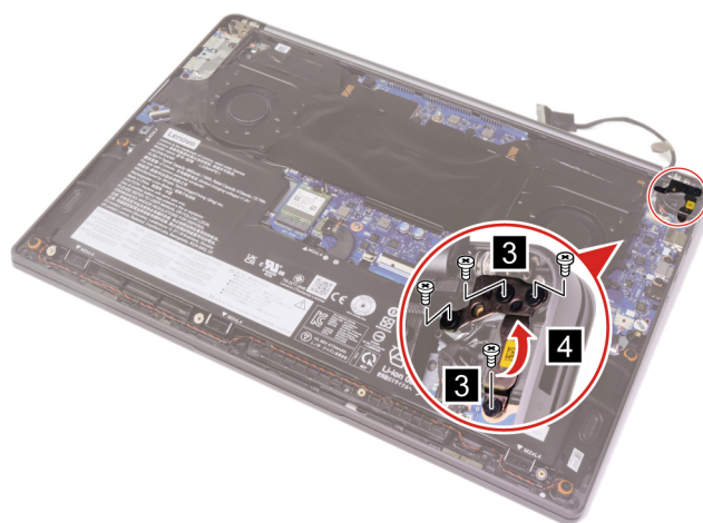
Figure 24. Remove four screws and then lift up the hinge
