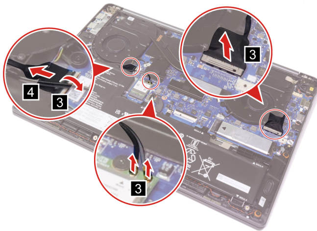
Figure 38. Disconnect antennas, EDP cable and camera cable
