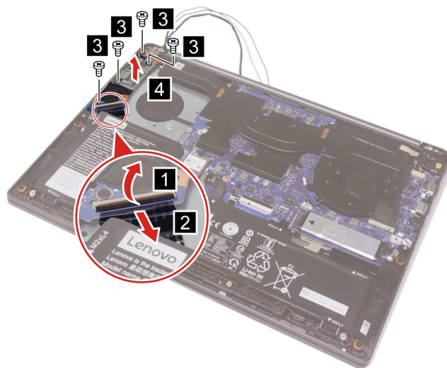
Figure 22. Disconnect the USB board cable and remove four screws and the USB board
