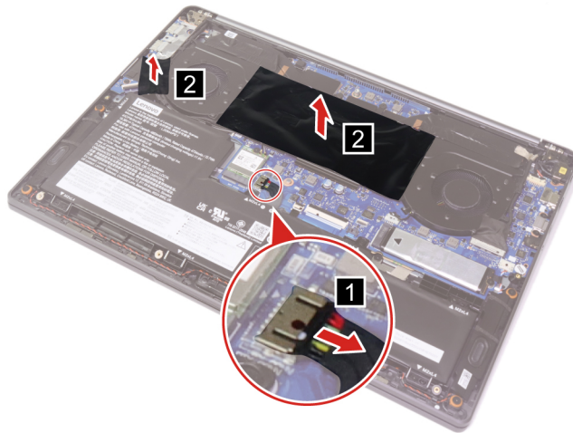
Figure 37. Disconnect the battery pack cable and peel off the thermal mylar
