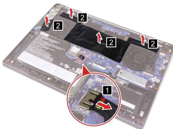
Figure 13. Disconnect battery pack cable and peel off thermal mylars
