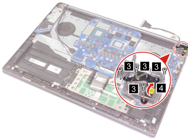
Figure 34. Remove four screws from the hinge and lift the hinge up.
