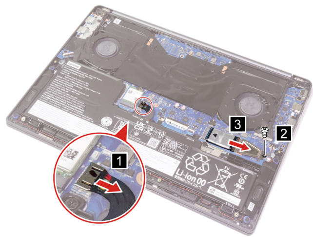
Figure 8. Disconnect the battery pack cable and remove one screw and the solid-state drive
