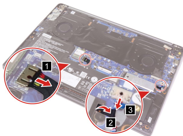
Figure 20. Disconnect the battery pack cable and speaker cable connectors
