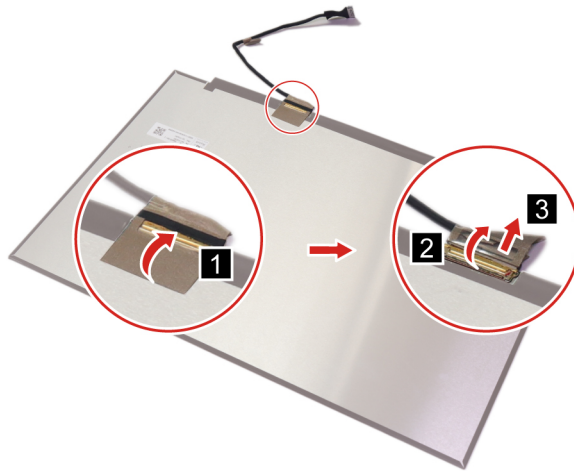
Figure 47. Remove the EDP cable
