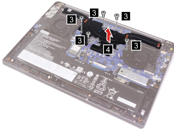
Figure 19. Remove five screws and then remove the heat sink
