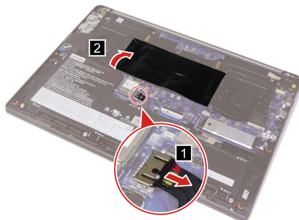
Figure 11. Disconnect the battery pack cable and lift up the thermal mylar
