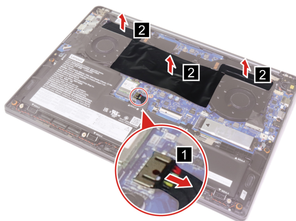
Figure 18. Disconnect the battery pack cable and peel off the thermal mylars
