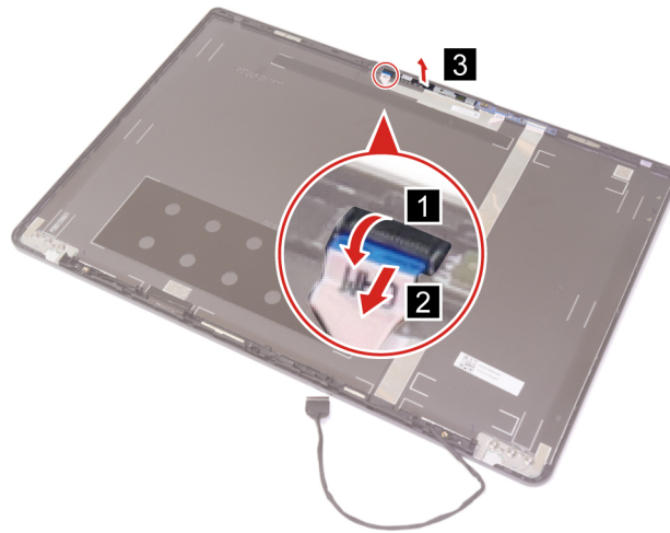
Figure 50. Disconnect the D-Mic cable and remove the camera board
