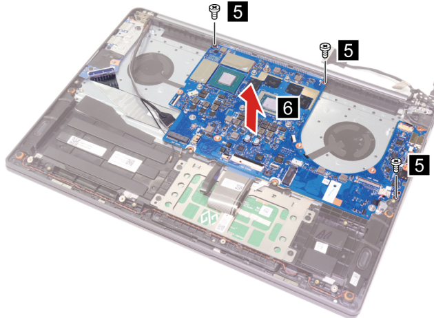
Figure 35. Remove three screws and the system board.
