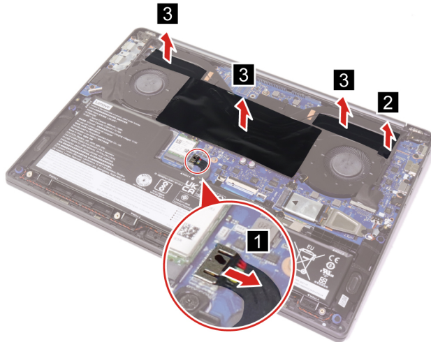
Figure 16. Disconnect the battery pack cable and peel off the thermal mylars
