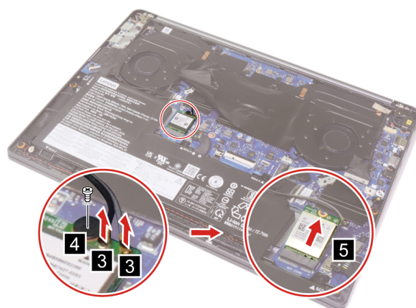
Figure 12. Disconnect the wireless antennas and remove one screw and the Wi-Fi card
