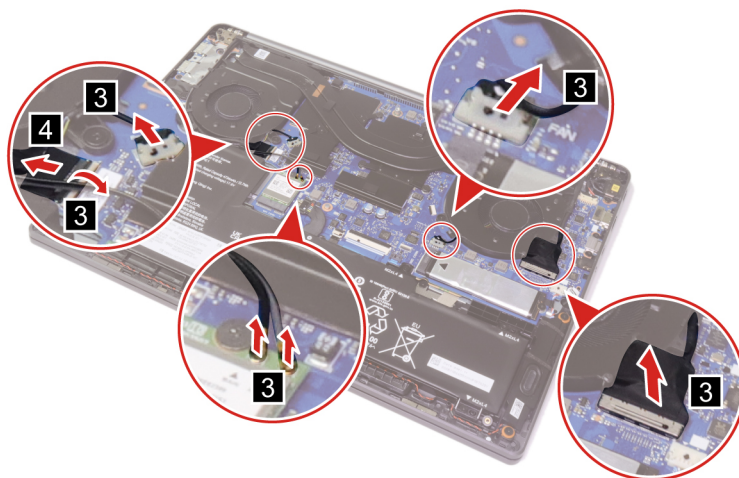
Figure 14. Disconnect the camera cable connector, EDP cable connector, fan cable connectors and antennas and then remove all the cables
