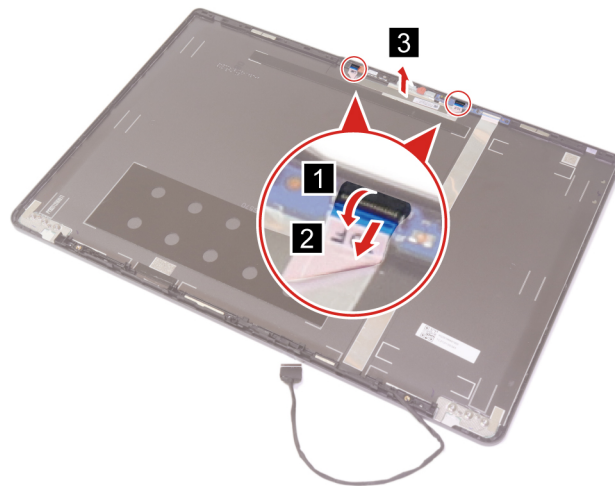
Figure 48. Remove the D-Mic cable
