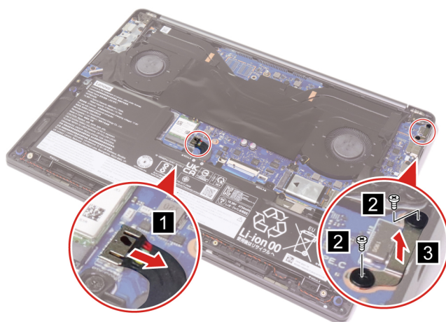
Figure 27. Disconnect the battery pack cable and then remove two screws and the upper I/O bracket
