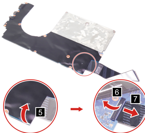
Figure 32. Peel back the system board mylar, disconnect the USB board cable and remove the USB board cable
