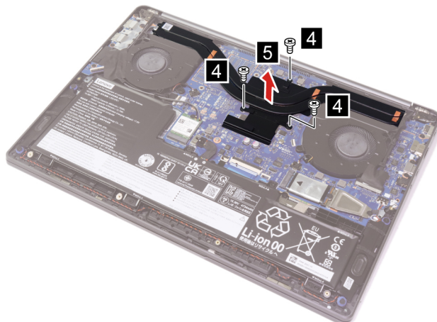
Figure 17. Remove three screws and then remove the heat sink
