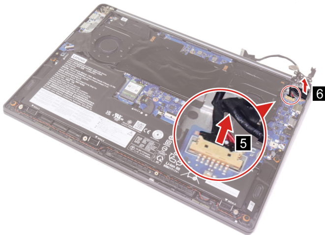
Figure 25. Disconnect the DC-in cable from the system board and remove the DC-in cable
