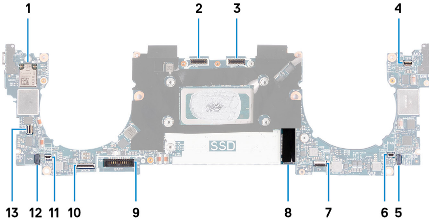
Figure 2. System-board connectors
