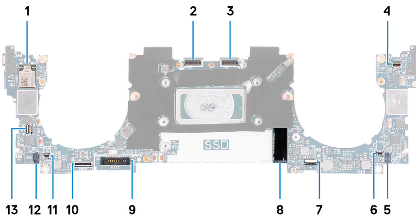
Figure 1. System-board connectors
