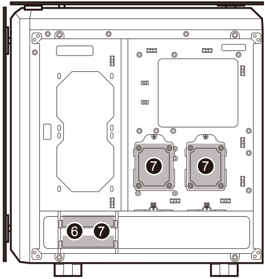
RIGHT SIDE
