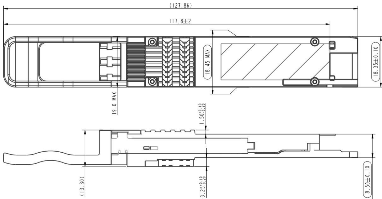
Figure 3. QDD4-400GB-ER8-AR Mechanical Dimensions
