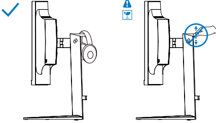
Headphone hook
