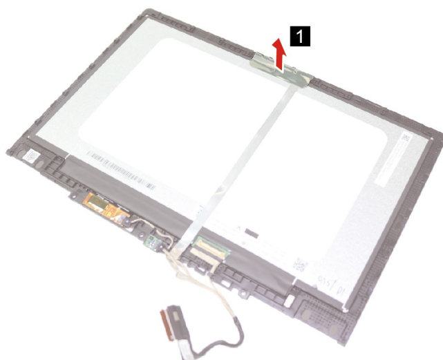
Figure 26. Remove the camera AL foil
