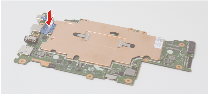
Figure 34. Install the mylar (a)
