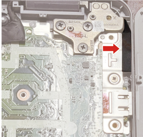
Figure 33. Install the sponge
