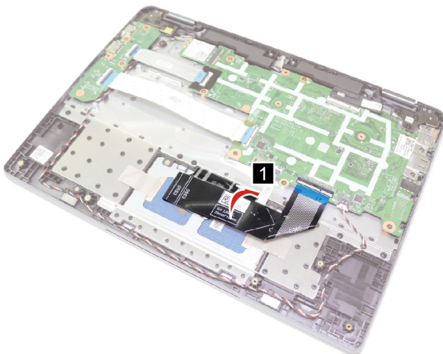
Figure 14. Lift the keyboard cable from the touch pad
