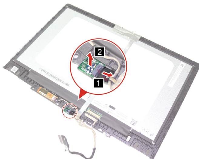
Figure 25. Disconnect the G-Sensor cable and then remove the G-Sensor board
