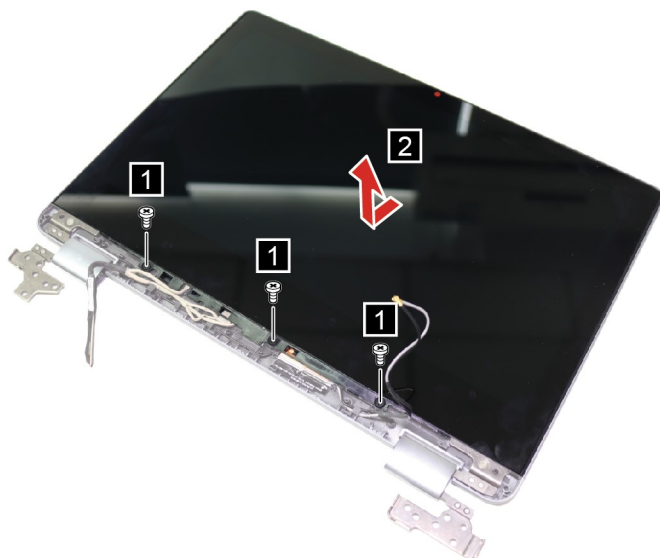
Figure 24. Remove the LCD module
