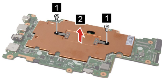
Figure 18. Remove two screws and then remove the thermal module
