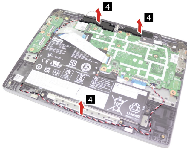
Figure 9. Remove the speakers
