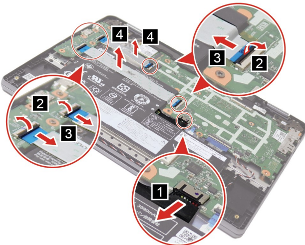
Figure 10. Remove the I/O board cables
