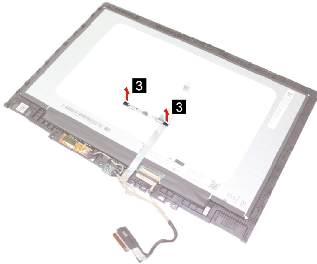
Figure 31. Remove the microphone rubbers
