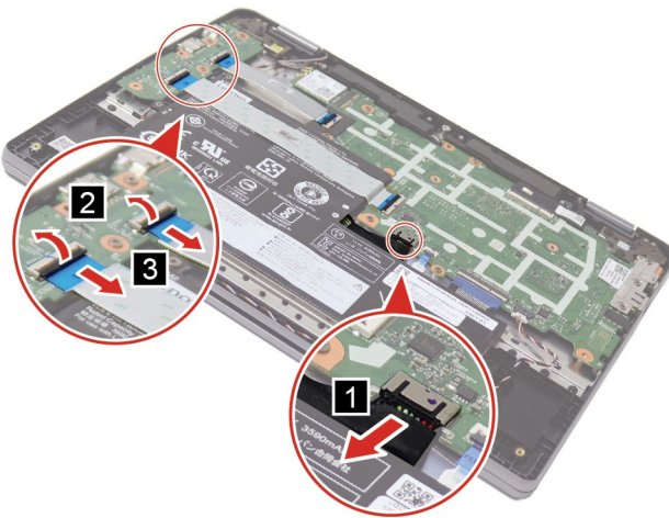
Figure 11. Disconnect the battery pack cable and I/O board cables from the I/O board
