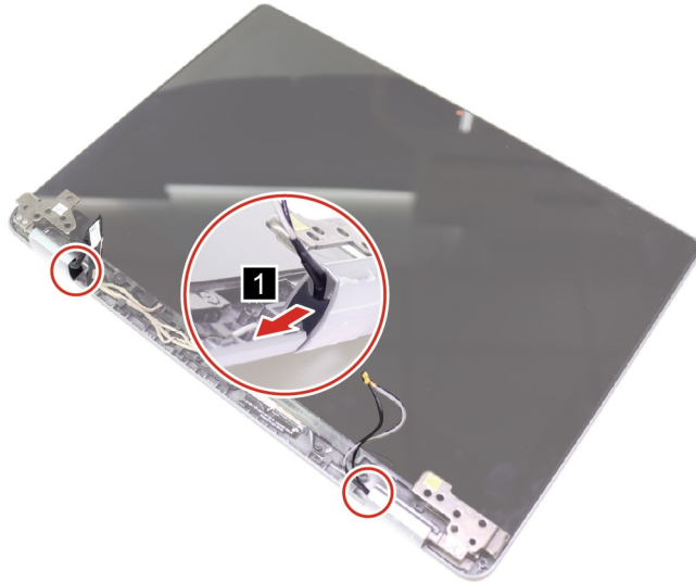
Figure 22. Remove the hinge rubbers
