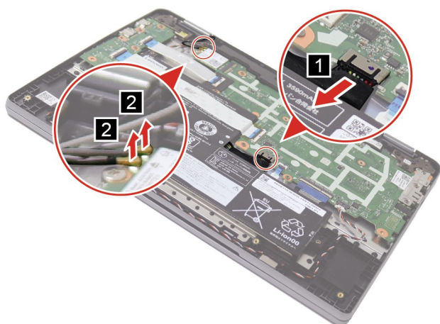
Figure 6. Disconnect the battery pack and Wi-Fi antenna cables
