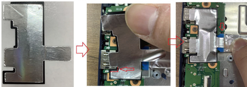
Figure 35. Install the mylar (b)
