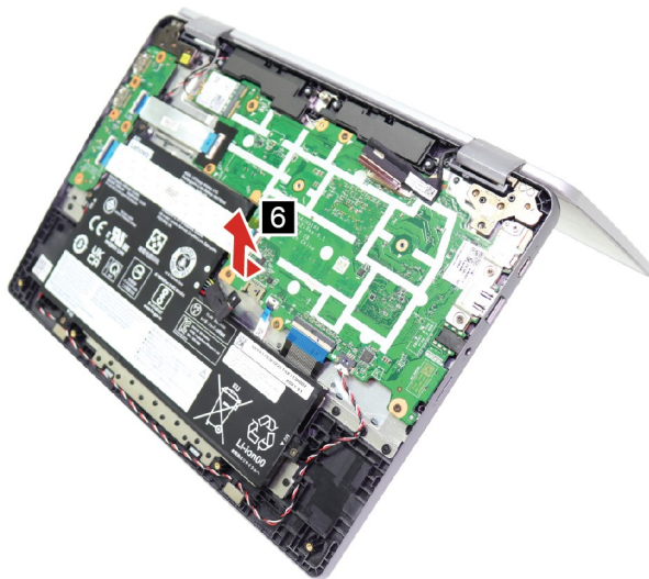
Figure 20. Remove the upper case assembly
