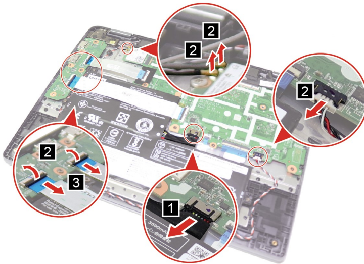
Figure 8. Disconnect the cables from the system board and Wi-Fi card
