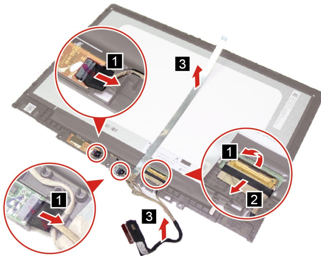
Figure 32. Disconnect and remove the EDP cable
