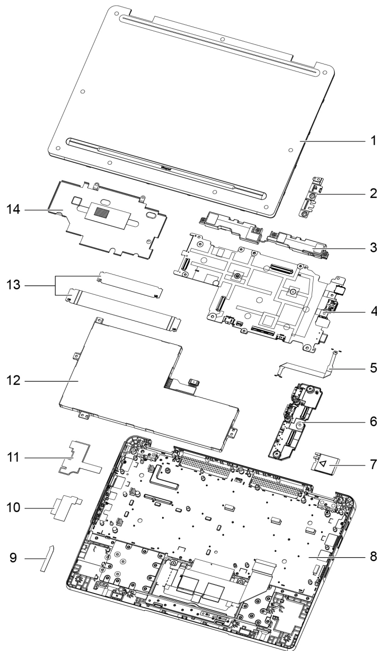
Figure 1. IP Flex 3 Chrome 11JL6 exploded view
