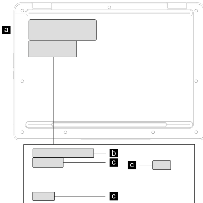
Figure 36. Label layout on the back side of the base cover
