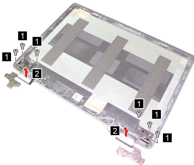
Figure 23. Remove six screws
