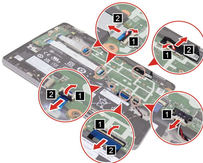
Figure 16. Disconnect the cables connected to the system board
