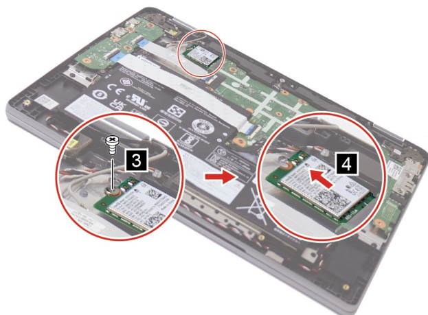
Figure 7. Remove the Wi-Fi card
