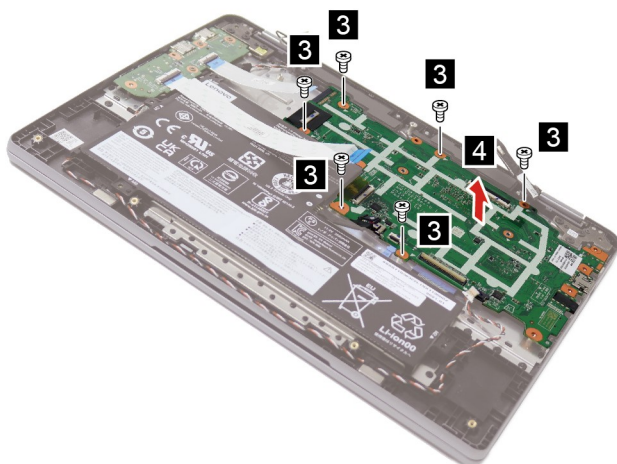
Figure 17. Remove six screws and then remove the system board
