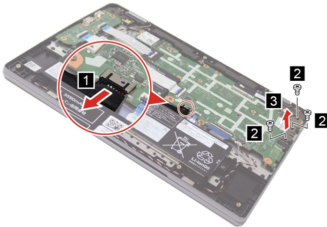
Figure 13. Disconnect the battery pack cable and remove three screws
