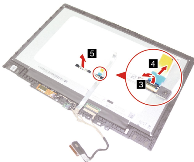
Figure 28. Remove the camera board
