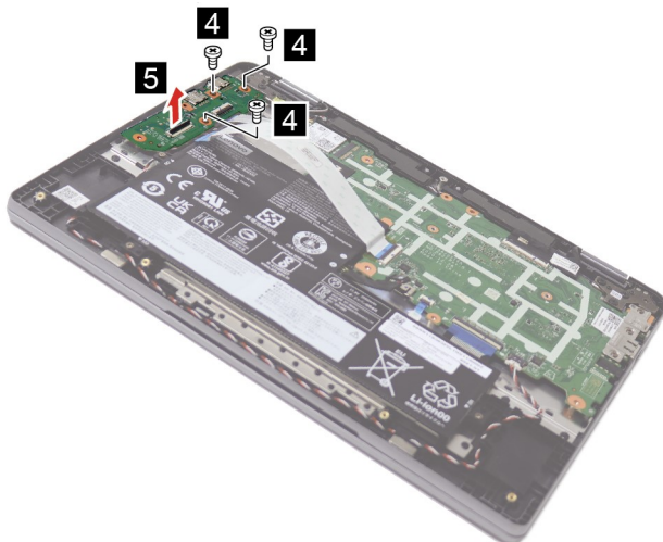
Figure 12. Remove the I/O board
