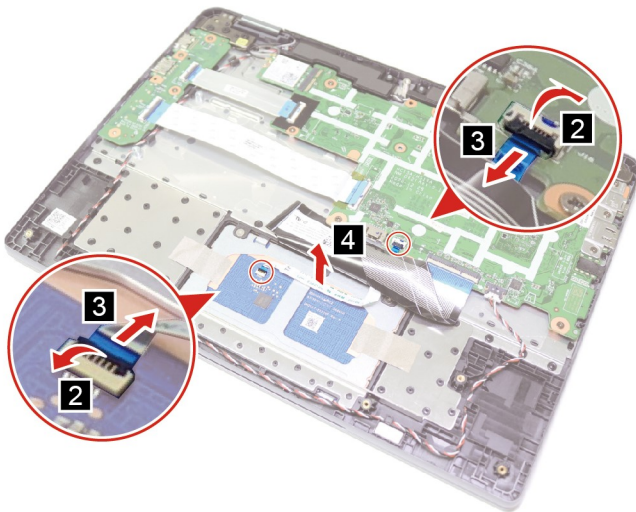
Figure 15. Disconnect and remove the touch pad cable
