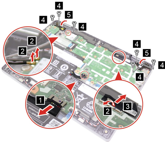
Figure 19. Disconnect the cables and remove six screws
