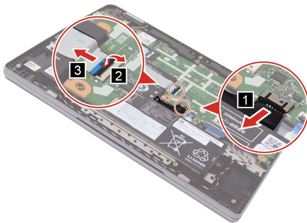
Figure 4. Disconnect the battery pack cable and I/O board cable from the system board
