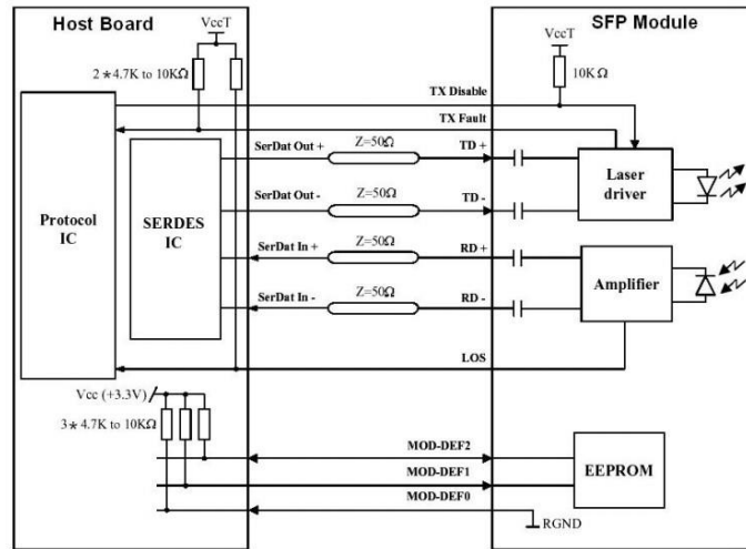
SFP Host Recommended Circuit
