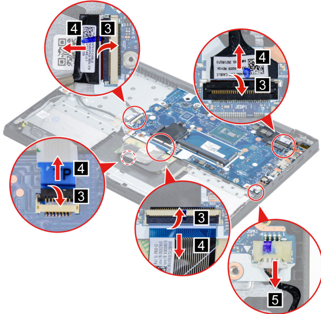
Figure 26. Disconnect the touchpad board cable and disconnect cables connected to the system board
