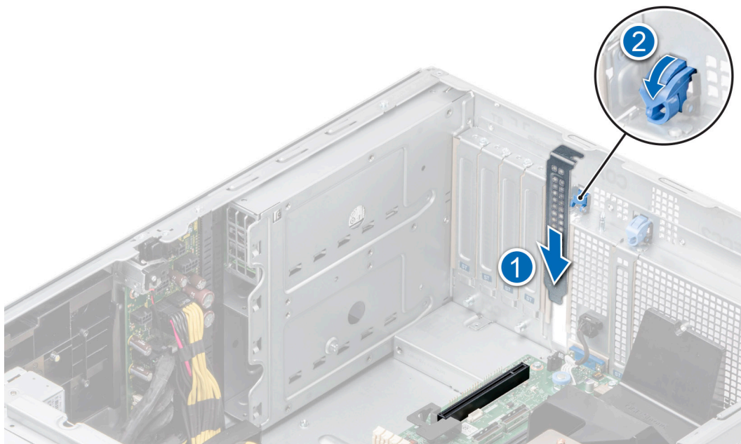
Figure 131. Installation de la plaque de recouvrement
