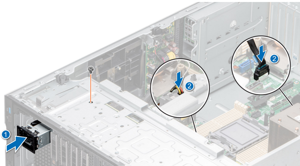
Figure 114. Installation du module BOSS S2
