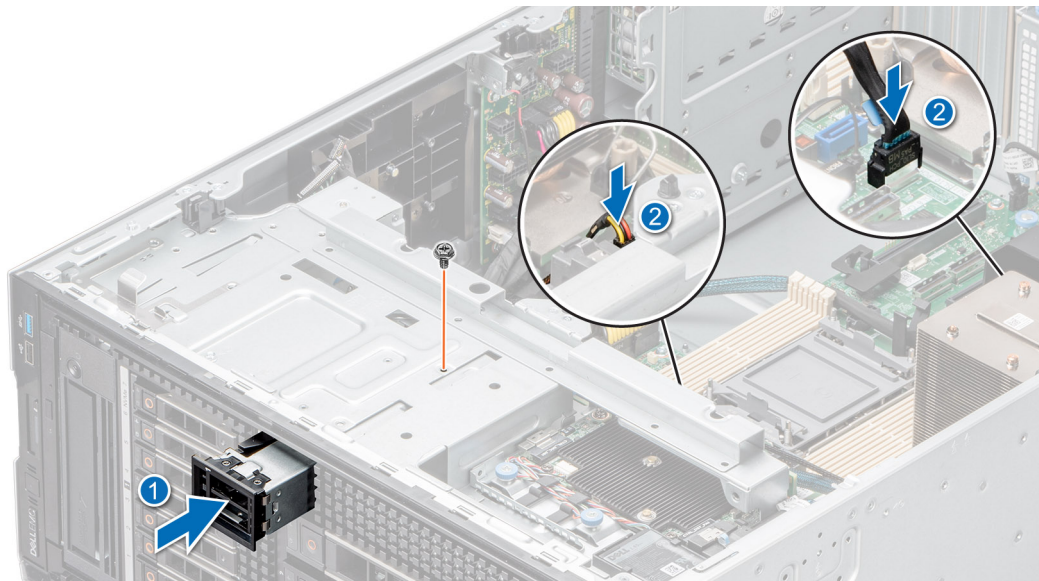
Figure 115. Installation du module BOSS S2
