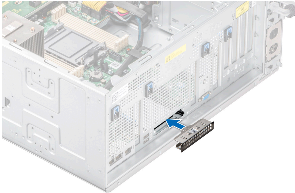
Figure 155. Installation de la plaque de recouvrement
