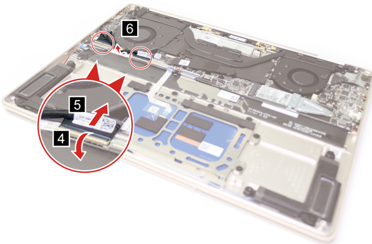
Figure 14. Disconnect the I/O board cable
