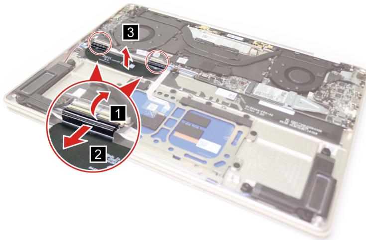
Figure 13. Disconnect the I/O board FPC
