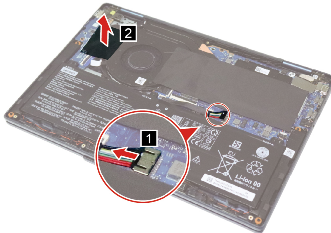
Figure 21. Disconnect the battery pack cable and peel off the mylar
