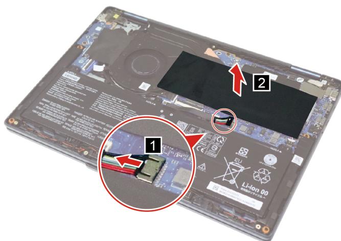
Figure 5. Disconnect the battery pack cable and peel off the mylar
