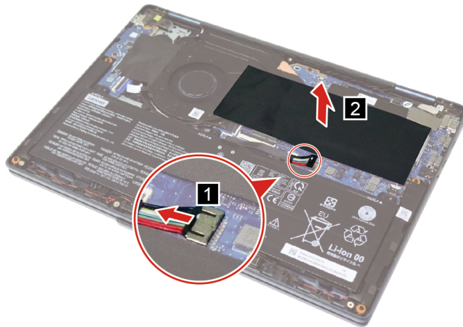
Figure 16. Disconnect the battery pack cable and peel off the mylar
