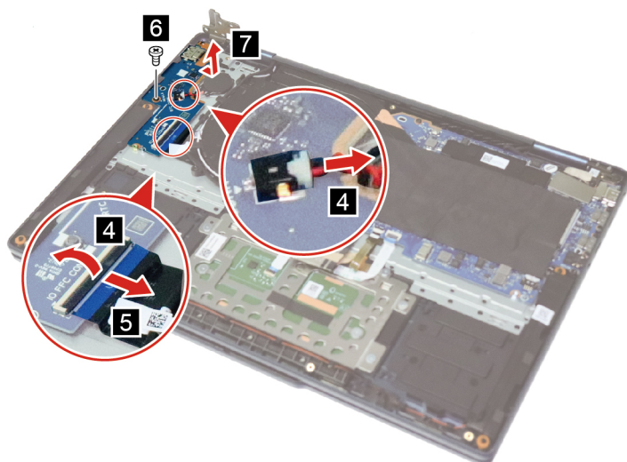
Figure 24. Disconnect the cables, remove one screw and the USB board
