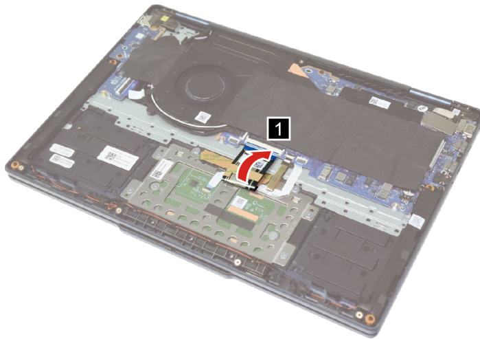
Figure 27. Peel back the keyboard cable
