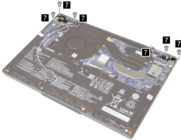
Figure 38. Remove six screws
