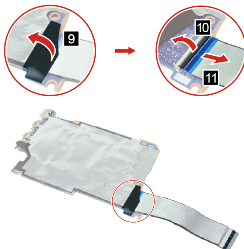
Figure 35. Peel off the mylar and remove the USB board cable
