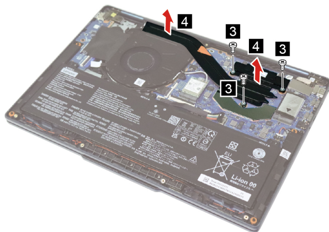
Figure 12. Remove three screws and remove the heat sink
