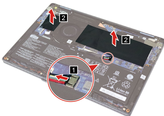
Figure 36. Disconnect the battery pack cable and peel off the mylars
