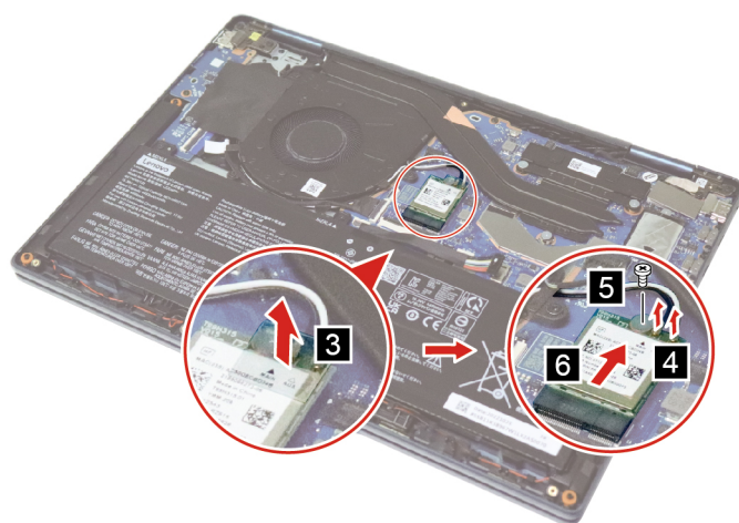
Figure 6. Peel off the mylar, disconnect the wireless antennas and remove the Wi-Fi card
