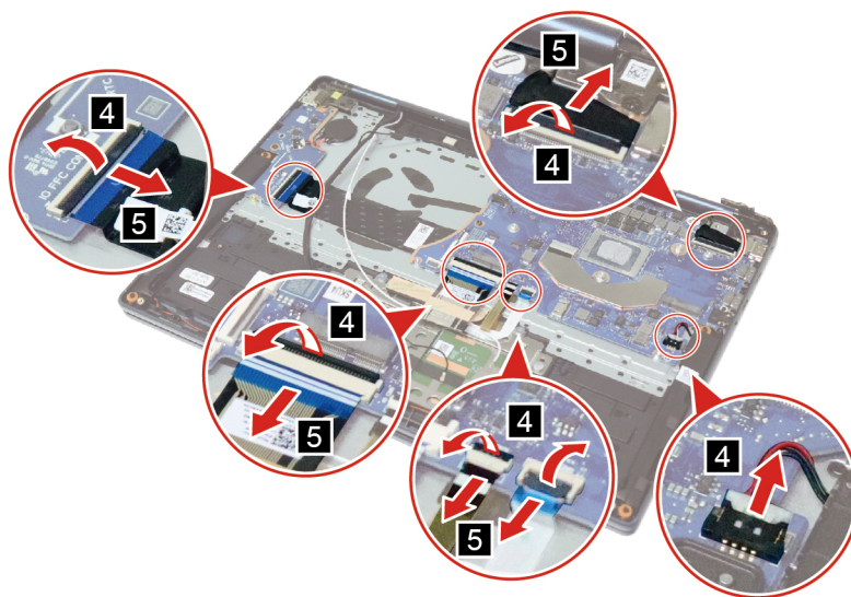
Figure 33. Disconnect the cables
