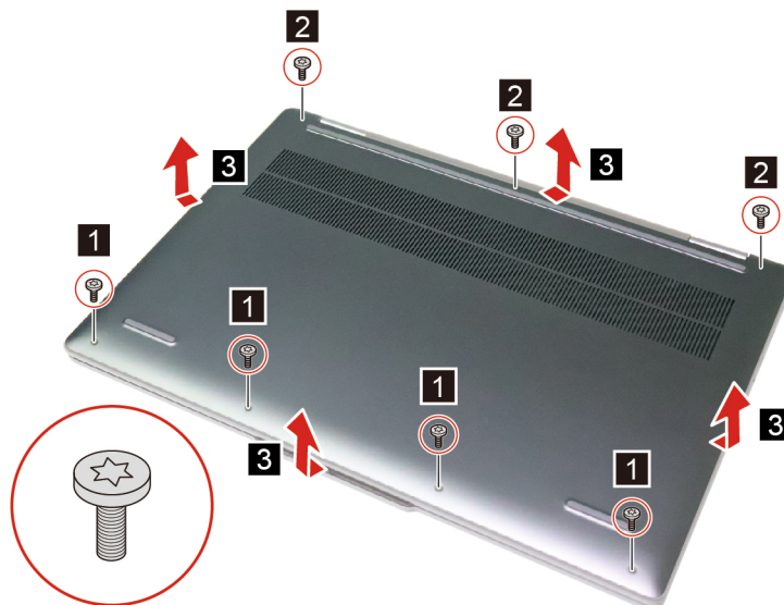
Figure 3. Remove the lower case
