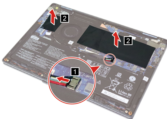
Figure 13. Disconnect the battery pack cable and peel off the mylars
