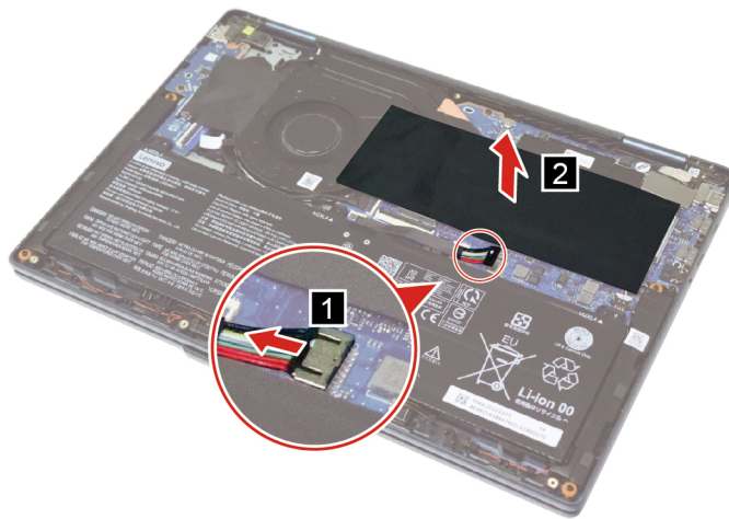
Figure 11. Disconnect the battery pack cable and peel off the mylar
