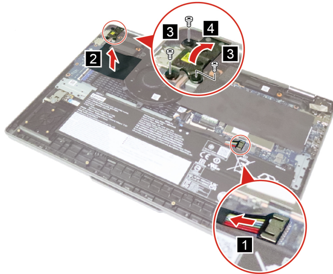
Figure 25. Disconnect the battery pack cable and peel off the mylar, remove three screws and lift the left hinge
