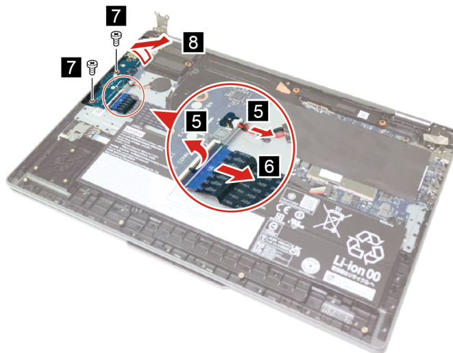
Figure 26. Disconnect the cables, remove two screws and the USB board
