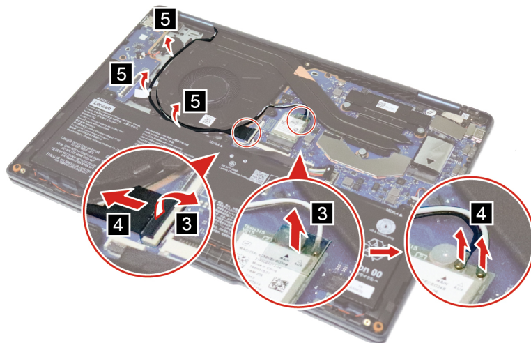
Figure 14. Disconnect the cables and remove them from the cable guide
