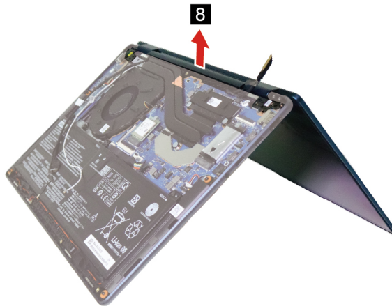
Figure 39. Rotate and remove the LCD module
