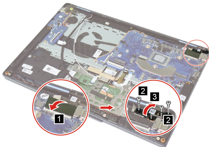
Figure 32. Peel off the absorber, remove three screws and lift the right hinge
