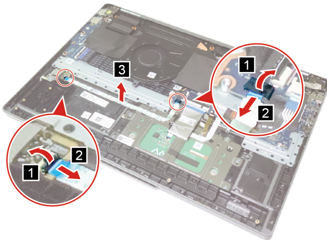
Figure 31. Disconnect and remove the fingerprint board cable
