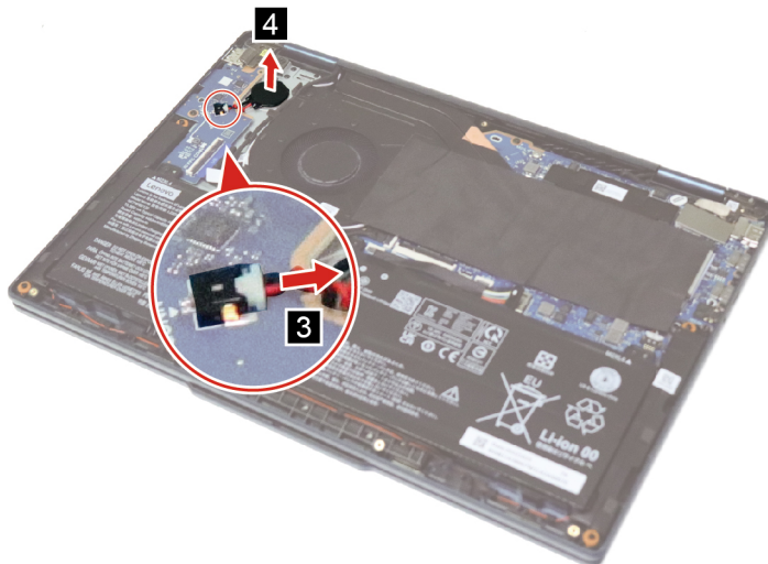
Figure 22. Disconnect and remove the coin-cell battery
