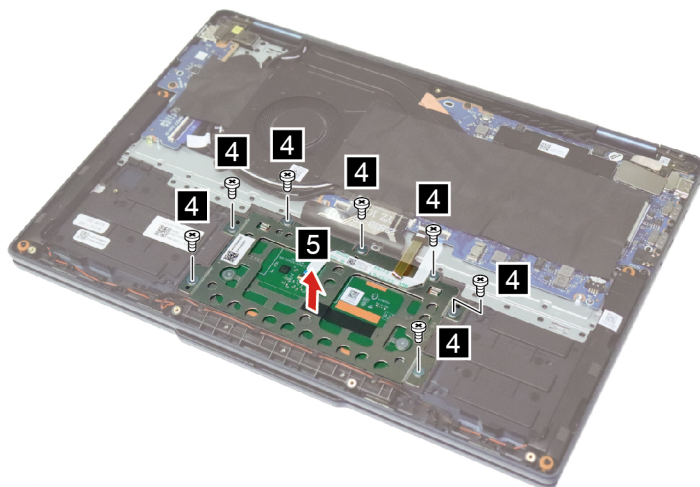
Figure 30. Remove seven screws and the touchpad
