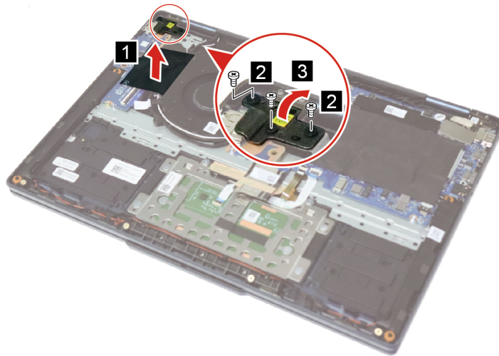
Figure 23. Peel off the mylar, remove three screws and lift the left hinge
