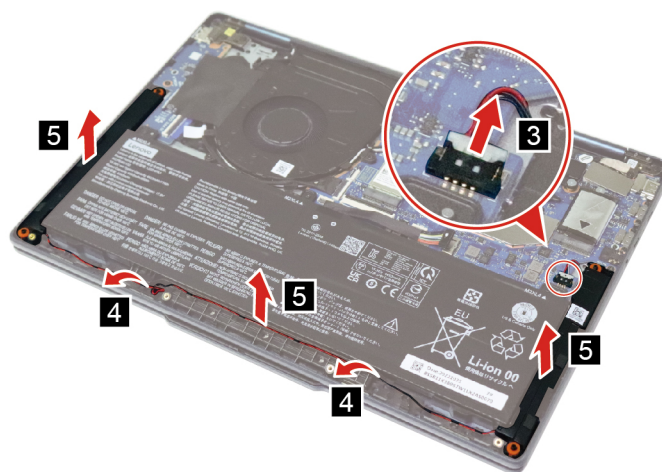
Figure 17. Disconnect and remove the speakers
