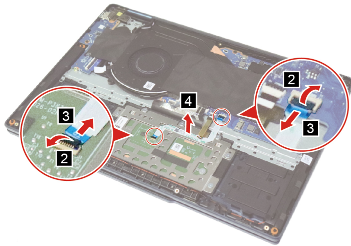
Figure 28. Disconnect and remove the touchpad cable
