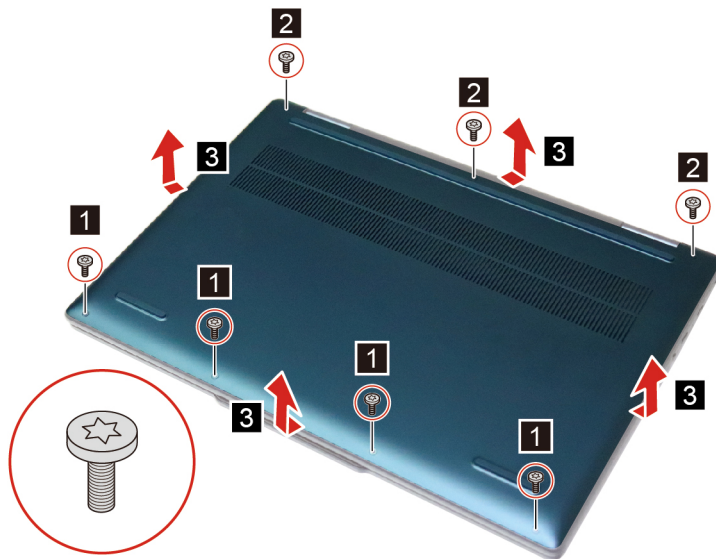
Figure 2. Remove the lower case
