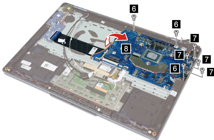
Figure 34. Remove seven screws and the system board with the USB board cable
