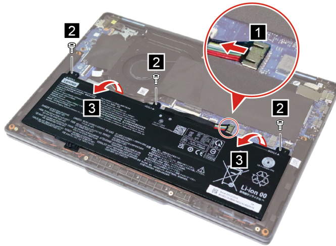
Figure 4. Disconnect the battery pack cable and remove the battery pack
