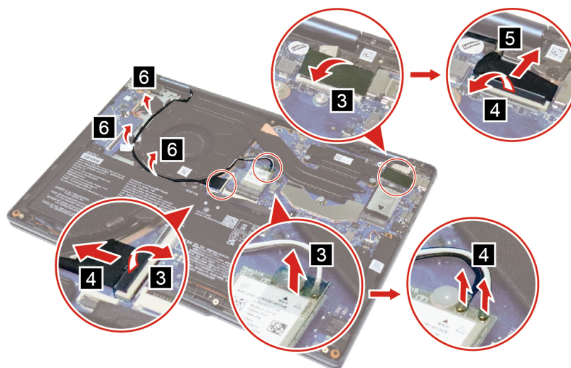
Figure 37. Disconnect and remove the cables from the cable guide
