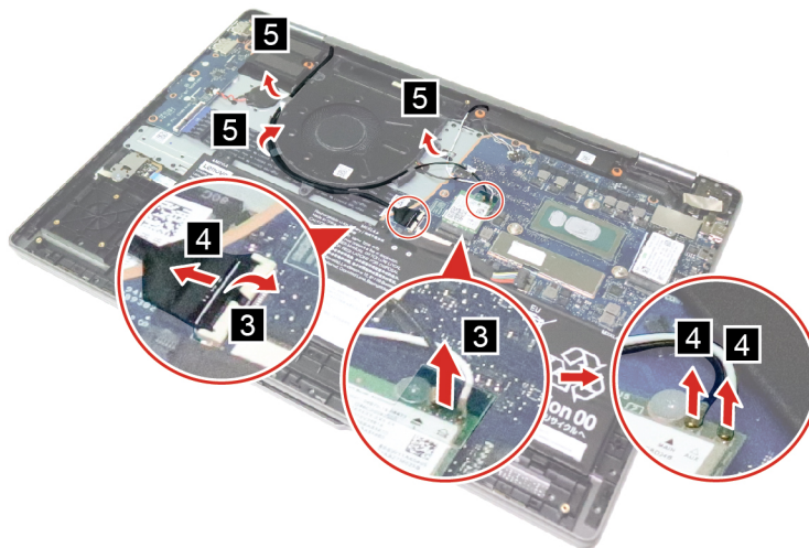
Figure 19. Disconnect the cables and remove them from the cable guide
