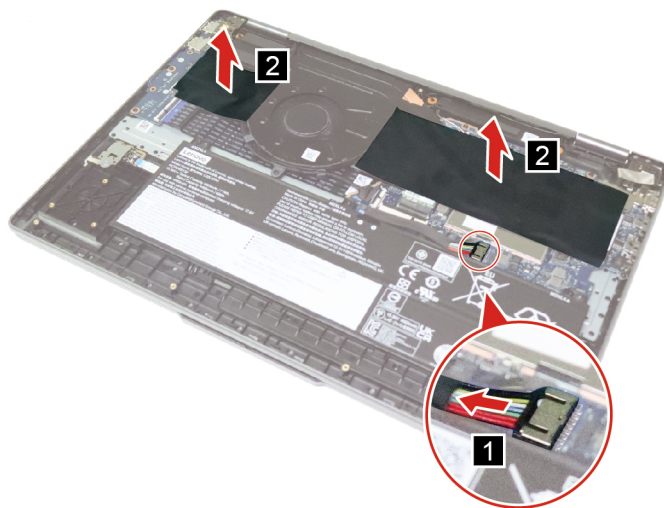
Figure 18. Disconnect the battery pack cable and peel off the mylars
