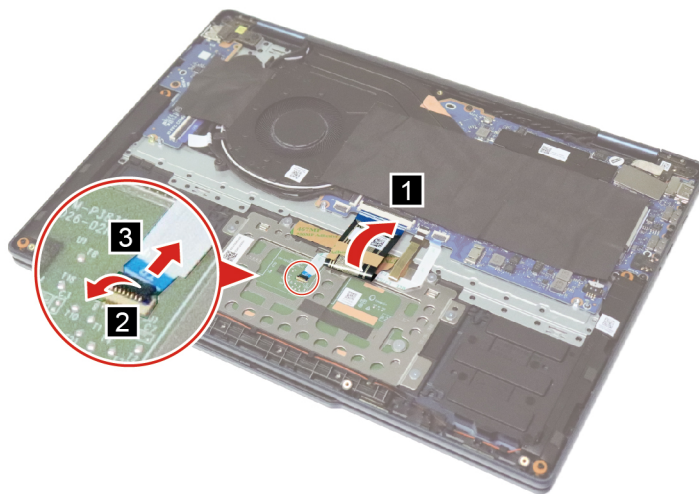
Figure 29. Peel back the keyboard cable and disconnect the touchpad cable
