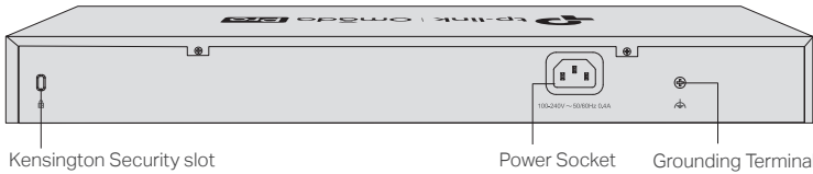
Figure 1-3 Rear Panel
