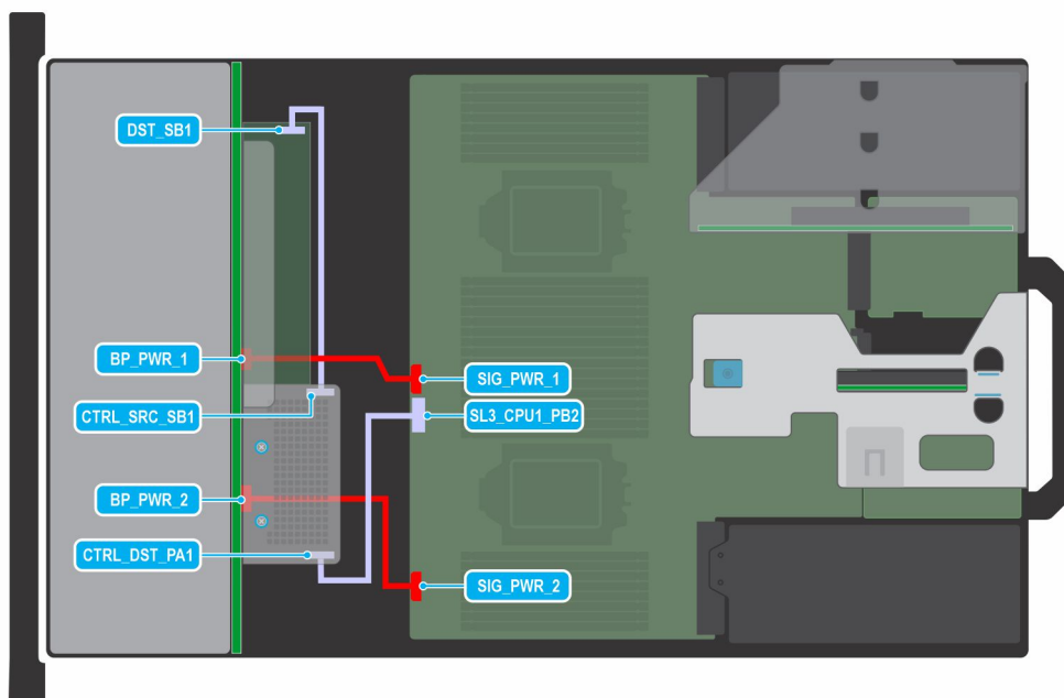
Figure 81. 24 x 2.5-inch SAS/SATA with expander and fPERC
