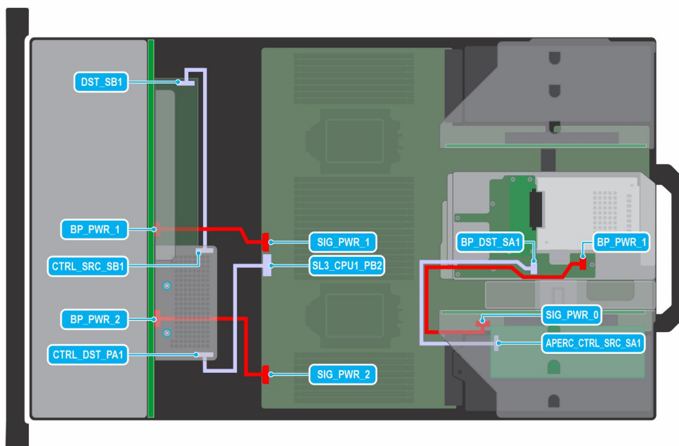
Figure 90. 24 x 2.5-inch SAS/SATA with separate controller, expander, APERC in R1, and fPERC
