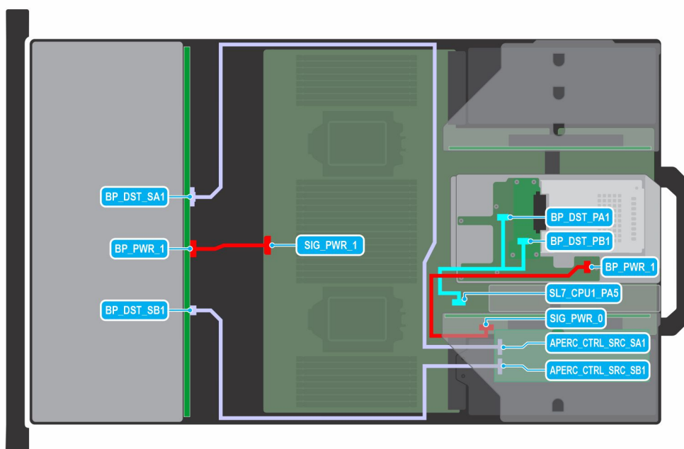
Figure 69. 12 x 3.5-inch SAS/SATA + 2 x 2.5-inch NVMe with APERC in Riser 1
