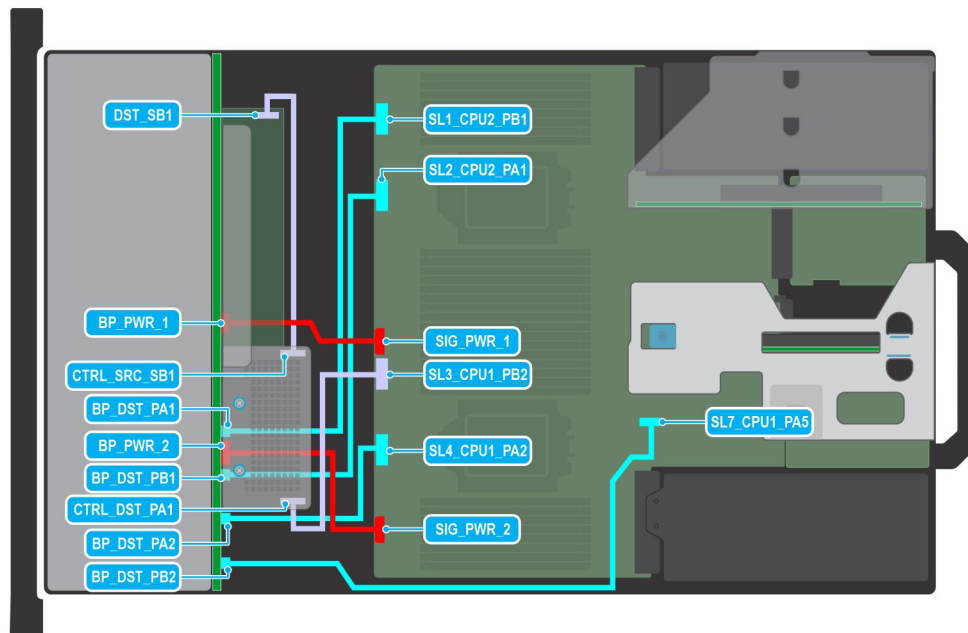
Figure 83. 24 x 2.5-inch SAS/SATA (8 universal + 16 SAS) with expander and fPERC
