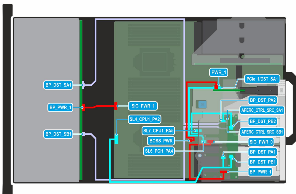
Figure 72. 12 x 3.5-inch SAS/SATA + 4 x 2.5-inch NVMe with APERC in Riser 2 and optional BOSS S2 module
