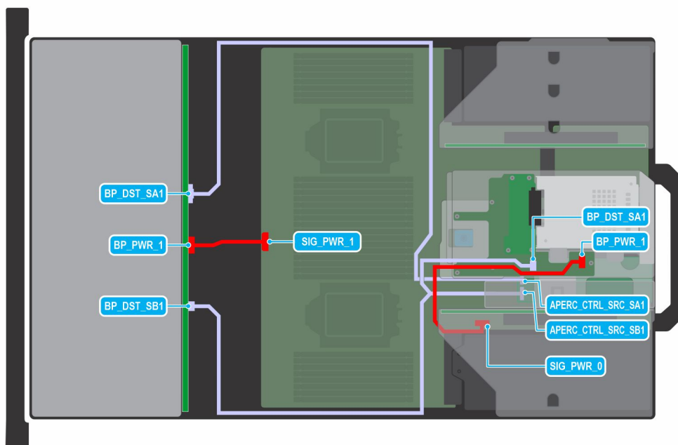
Figure 68. 12 x 3.5-inch SAS/SATA + 2 x 2.5-inch SAS/SATA with APERC in Riser 2
