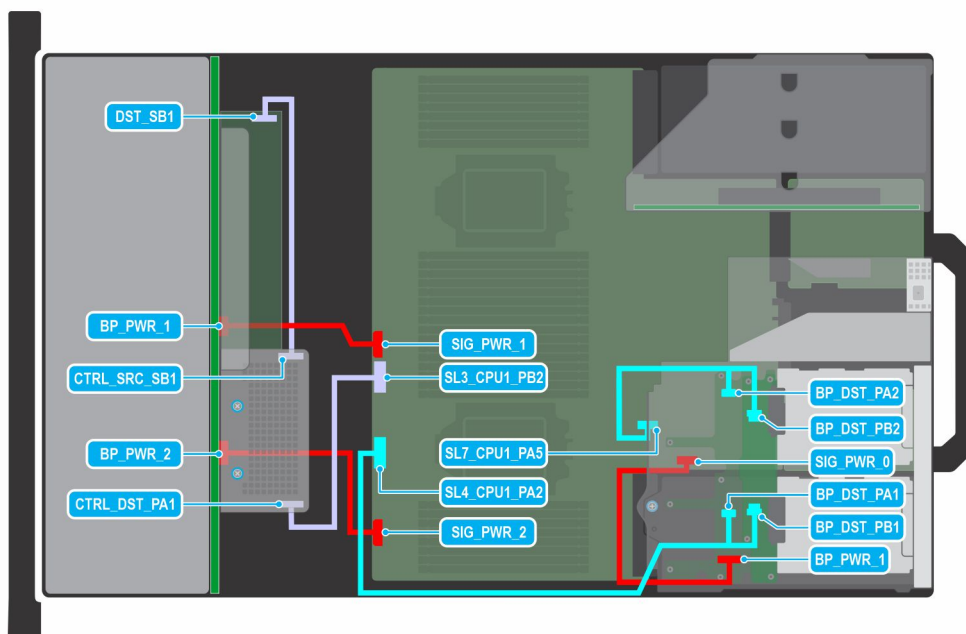
Figure 89. 24 x 2.5-inch SAS/SATA + 4 x 2.5-inch NVMe with expander and fPERC
