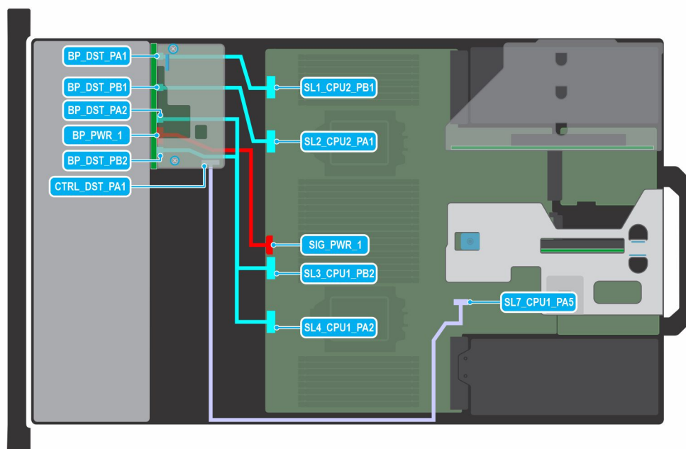
Figure 73. 8 x 2.5-inch SAS with NVMe and fPERC
