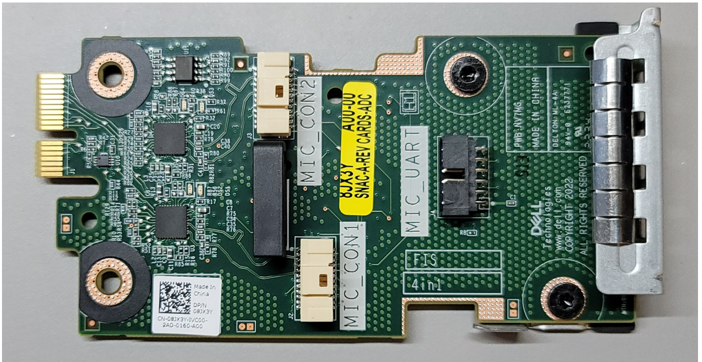
Figure 227. Management Interface Card (MIC)
