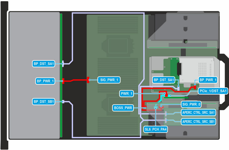
Figure 67. 12 x 3.5-inch SAS/SATA + 2 x 2.5-inch SAS/SATA with APERC in Riser 1 and optional BOSS S2 module
