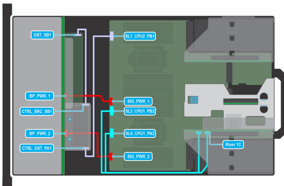
Figure 82. 24 x 2.5-inch SAS/SATA with expander, fPERC, and Riser 1C
