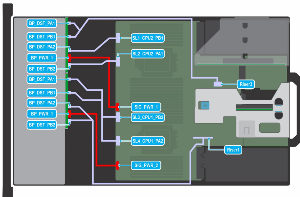
Figure 76. 16 x 2.5-inch NVMe direct
