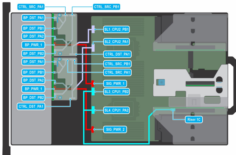
Figure 75. 16 x 2.5-inch NVMe with fPERC and Riser 1C
