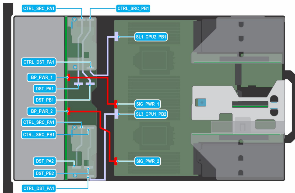
Figure 93. 24 x 2.5-inch NVMe switch with 2 front PERC
