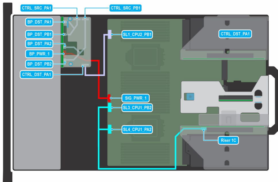
Figure 74. 8 x 2.5-inch SAS with fPERC and Riser 1C
