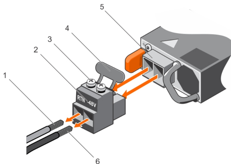
Figure 215. Removing the DC Input Power Wires
