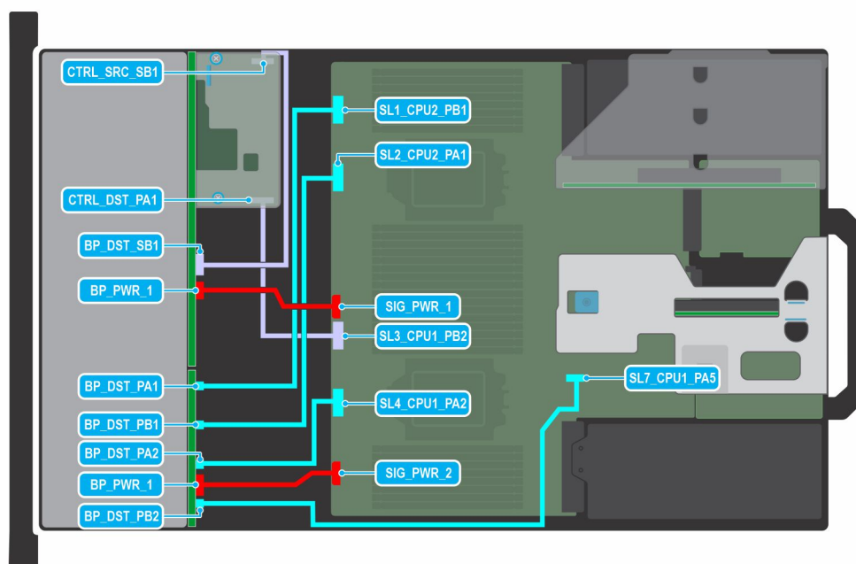
Figure 80. 16 x 2.5-inch SAS/SATA + 8 x 2.5-inch NVMe with fPERC
