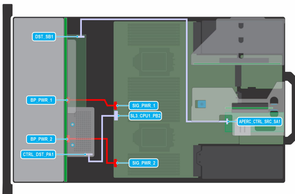
Figure 85. 24 x 2.5-inch SAS/SATA with dual controller, expander, fPERC, and APERC in Riser 2
