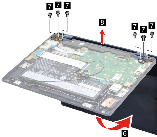
Figure 18. Remove the LCD module
