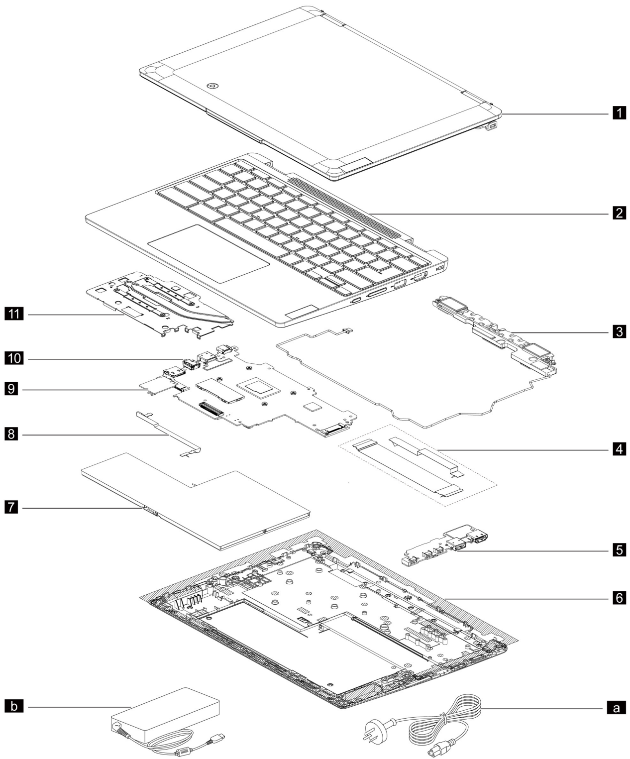
Figure 1. exploded view
