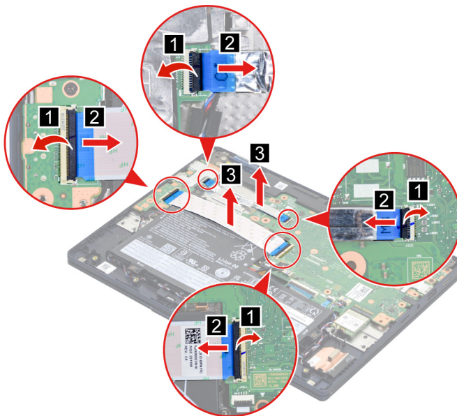
Figure 8. Remove the I/O board cable
