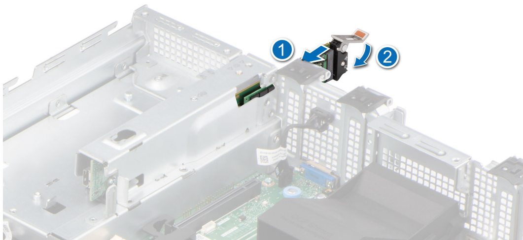
Figure 85. Installation du support de la carte BOSS S2
