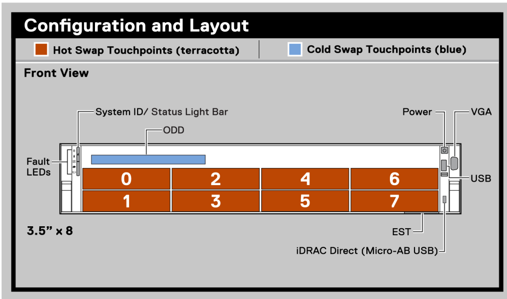
Figure 13. Configuration et disposition
