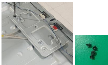
Remove the speaker units. (L/R)
