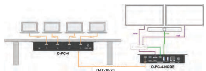
UC-room with BYOD support on Windows-based UC-systems.
