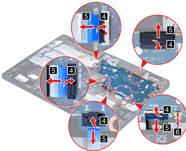
Figure 12. Disconnect cables connected to the system board
