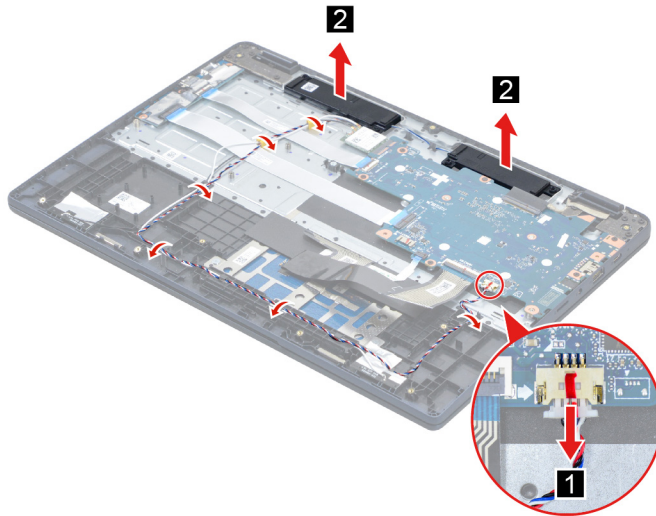
Figure 7. Remove the speakers
