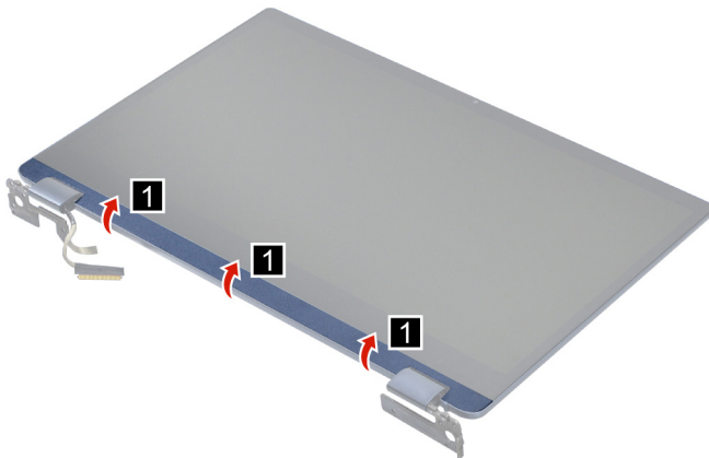
Figure 16. Remove the strip cover
