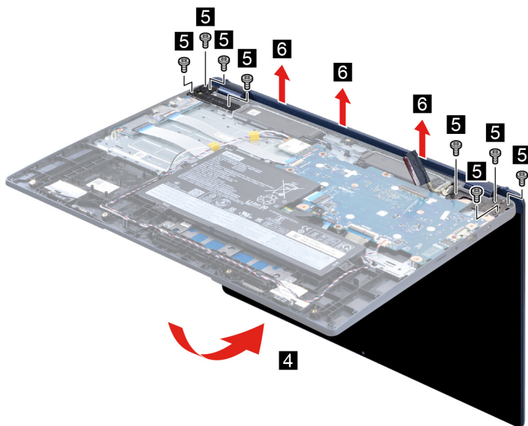
Figure 15. Remove the LCD module
