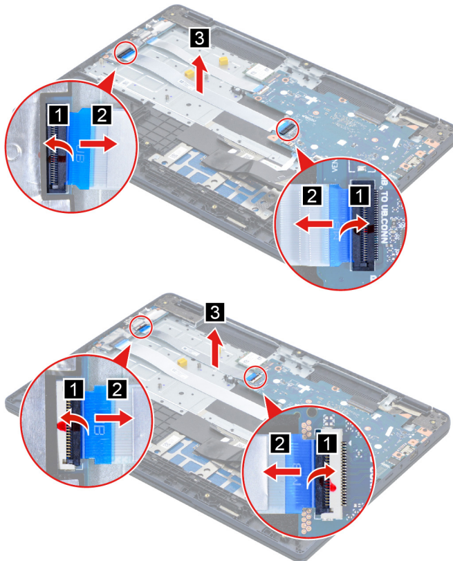
Figure 9. Remove the I/O board cable
