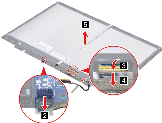
Figure 23. Remove the EDP cable
