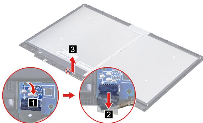
Figure 19. Remove the sensor board
