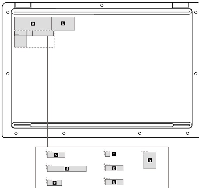
Figure 24. Label layout on the back side of the base cover
