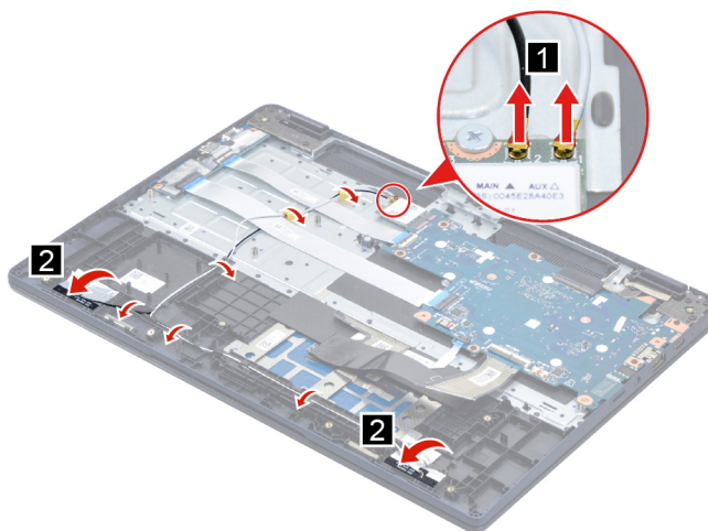
Figure 8. Remove the antennas
