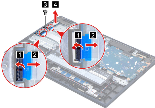
Figure 10. Remove the I/O board
