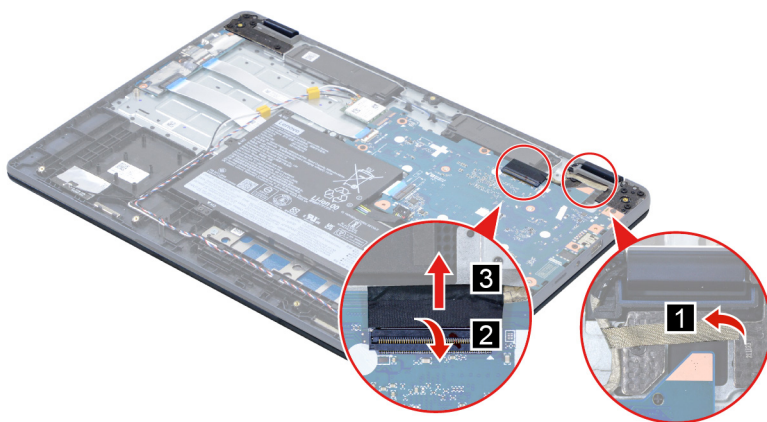
Figure 14. Peel off the tape and disconnect the LCD cable
