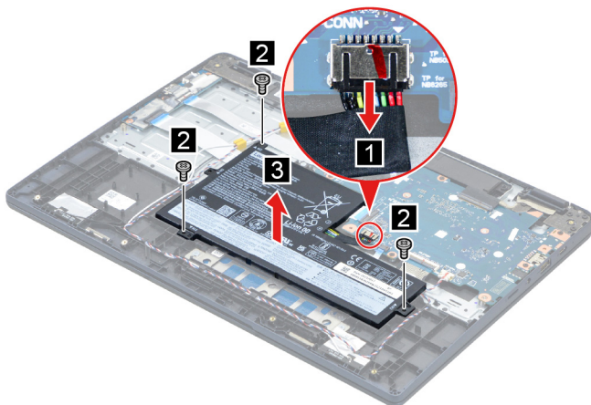
Figure 5. Remove three screws and remove the battery pack
