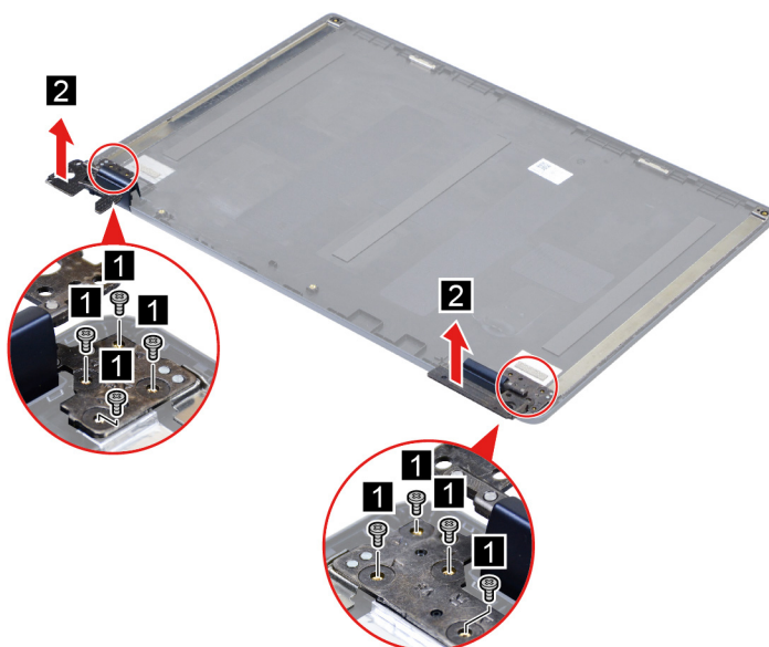
Figure 18. Remove the hinges
