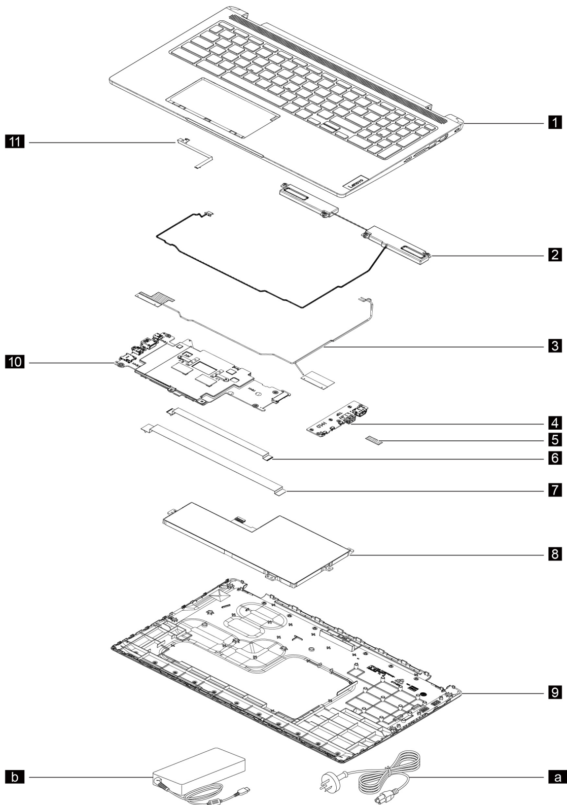
Figure 1. Exploded view
