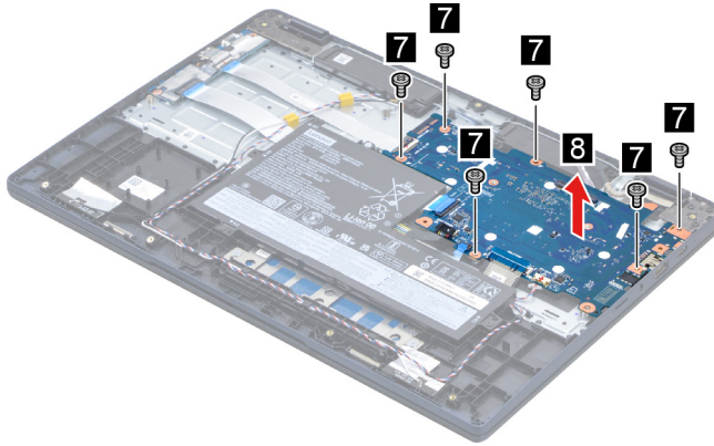
Figure 13. Remove six screws and remove the system board
