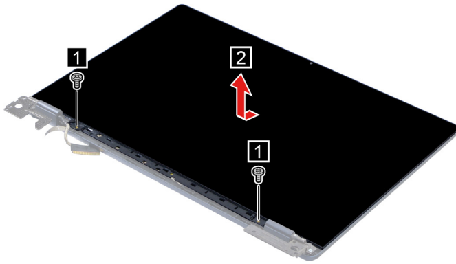
Figure 17. Remove two screws and remove the LCD panel
