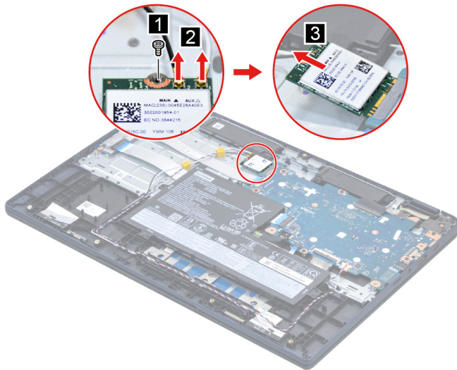
Figure 11. Remove the Wi-Fi card
