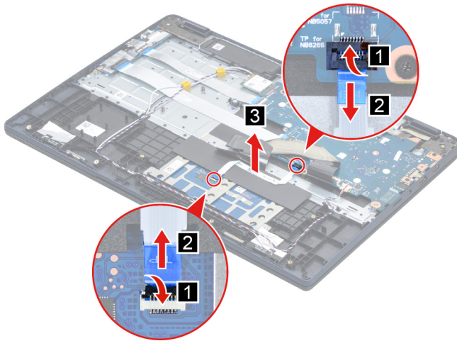
Figure 6. Remove the touchpad board cable
