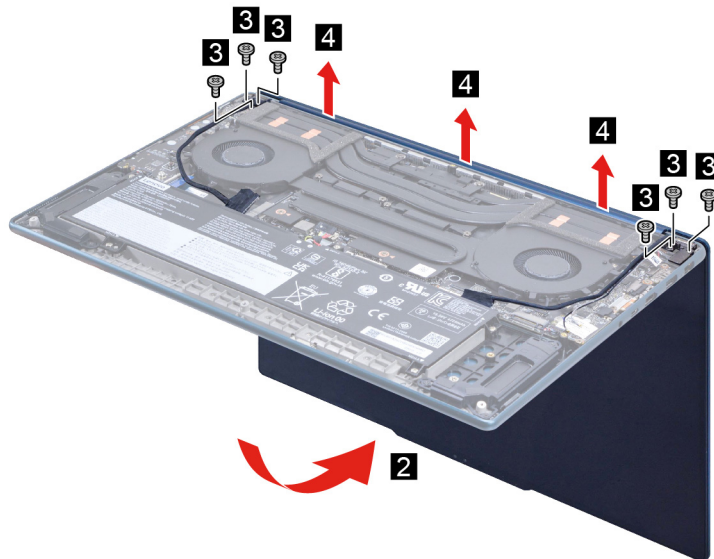
Figure 25. Remove the LCD module
