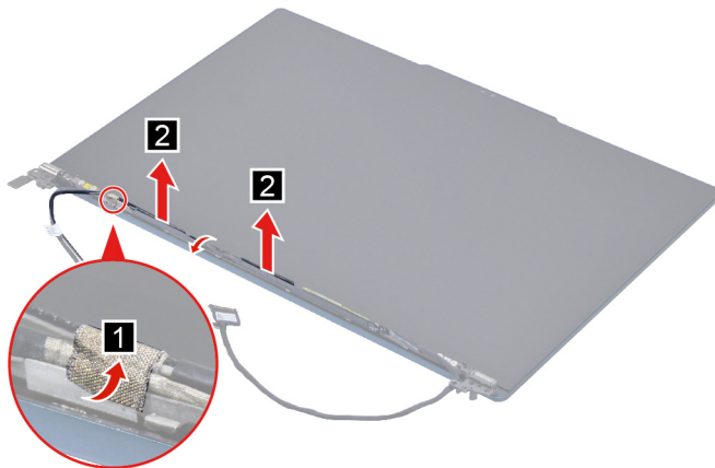
Figure 27. Remove the antenna
