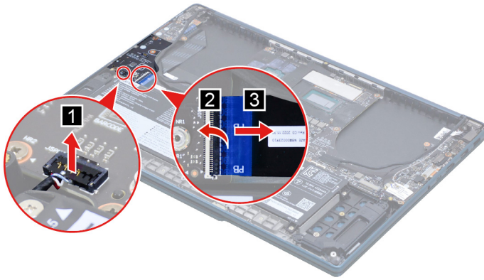
Figure 13. Disconnect cables connected to the power board
