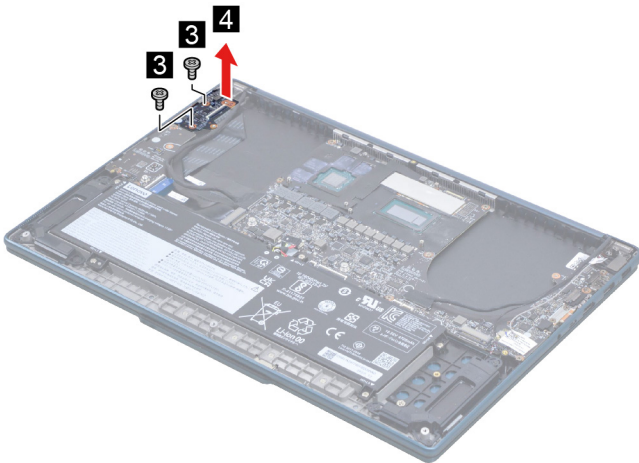
Figure 16. Remove two screws and remove the I/O board
