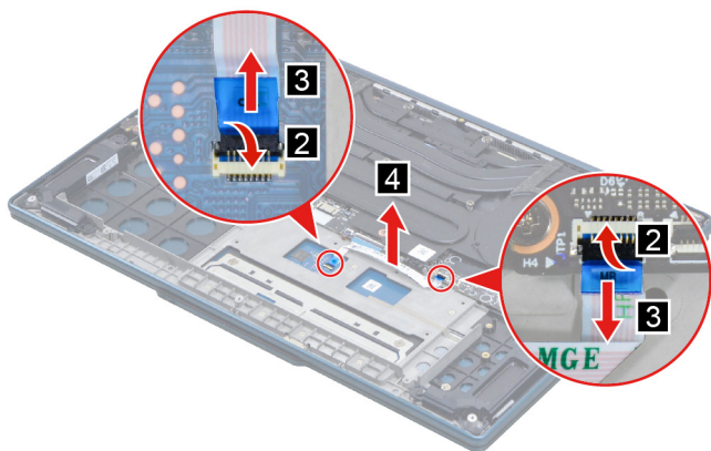
Figure 10. Remove the touchpad board cable
