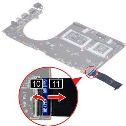
Figure 21. Remove the power board cable
