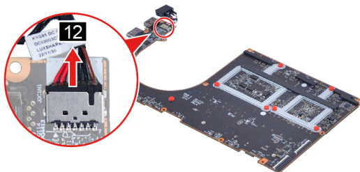
Figure 22. Remove the DC-in cable
