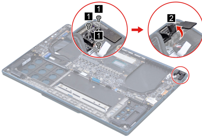
Figure 17. Remove three screws and open the hinge
