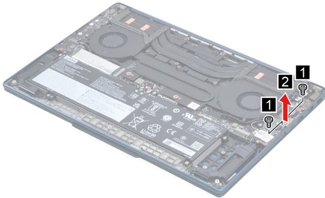
Figure 8. Remove the Type-C bracket
