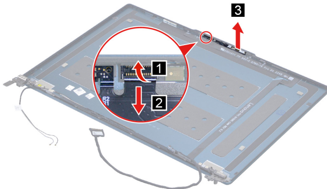
Figure 36. Remove the camera board
