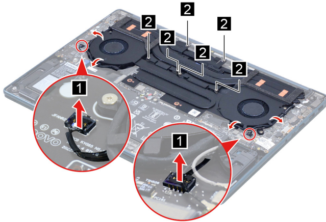
Figure 11. Disconnect the fan cable and loosen six screws
