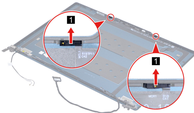
Figure 31. Remove the microphone rubber
