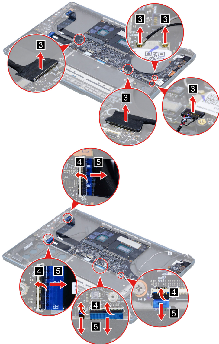
Figure 18. Disconnect cables connected to the system board
