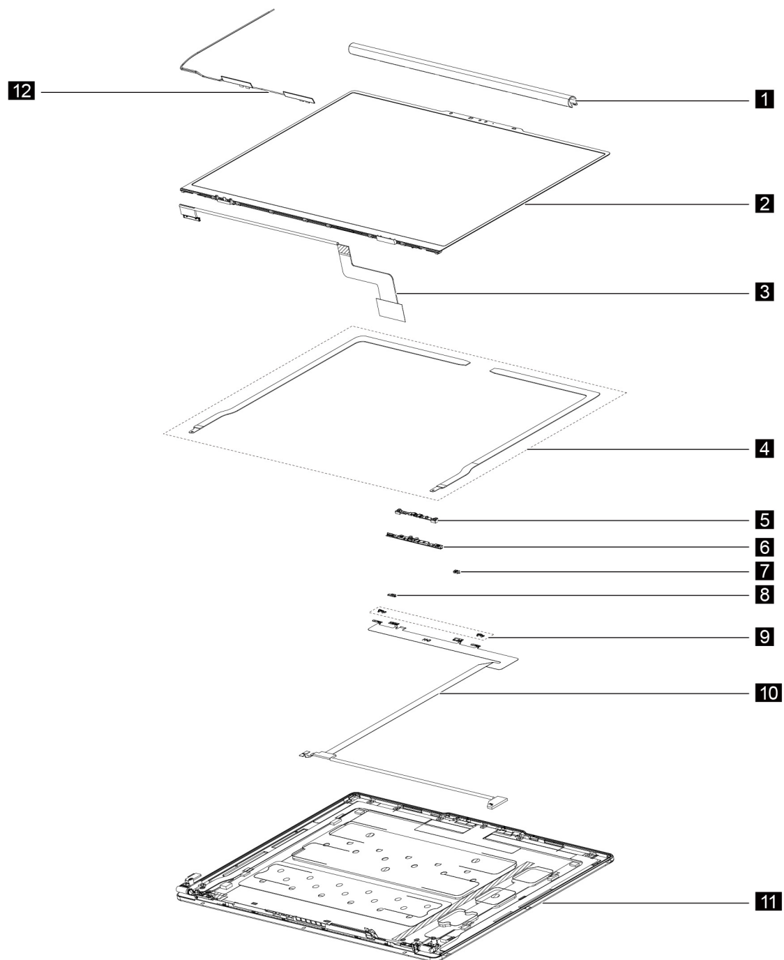
Figure 2. LCD module - exploded view
