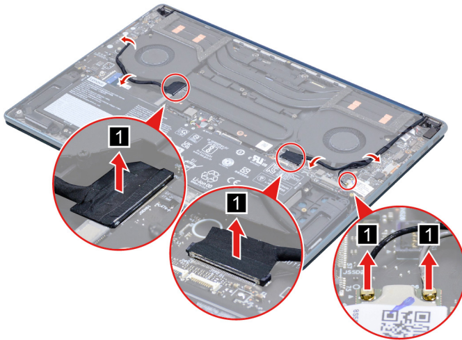
Figure 24. Disconnect cables and antenna cable
