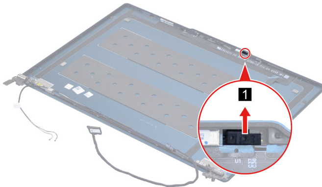
Figure 32. Remove the ToF rubber
