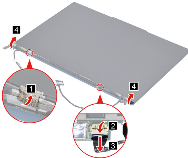
Figure 28. Disconnect the EDP cable from the LCD cover and remove the hinge deco
