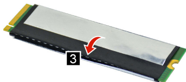
Figure 7. Remove the SSD mylar
