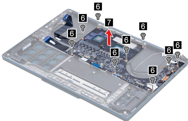
Figure 19. Remove nine screws and remove the system board
