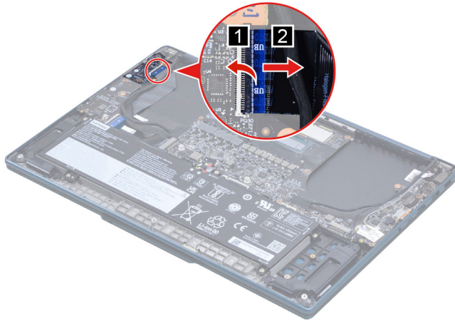
Figure 15. Disconnect the I/O board cable
