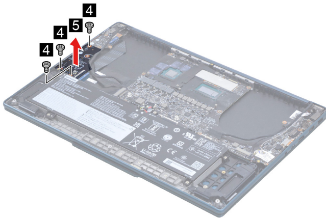
Figure 14. Remove three screws and remove the power board
