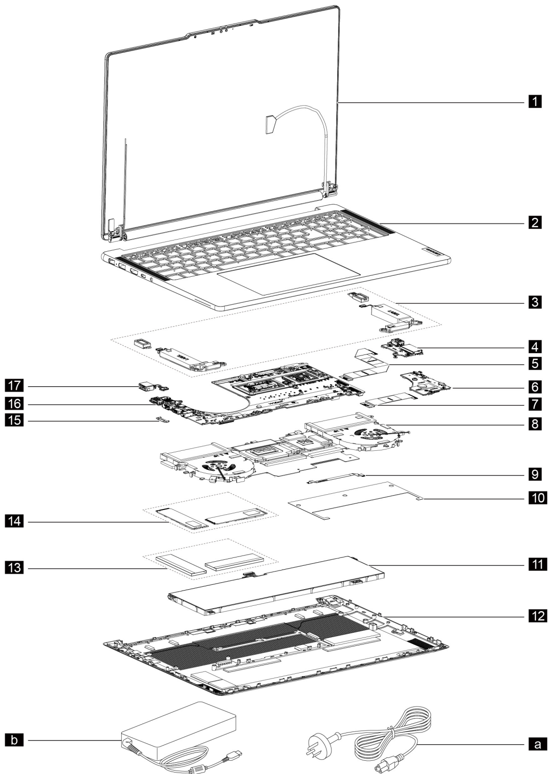
Figure 1. exploded view
