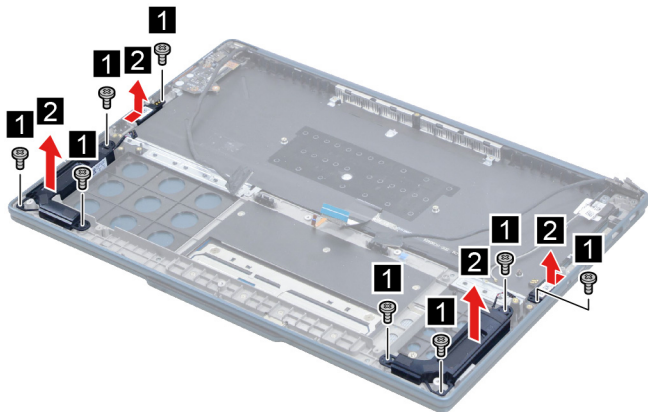
Figure 23. Remove the speakers
