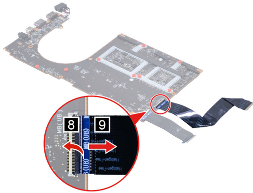
Figure 20. Remove the I/O board cable
