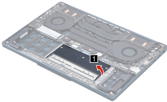
Figure 9. Remove the touchpad board mylar
