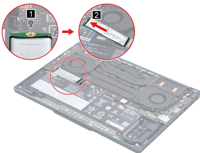
Figure 6. Remove the SSD
