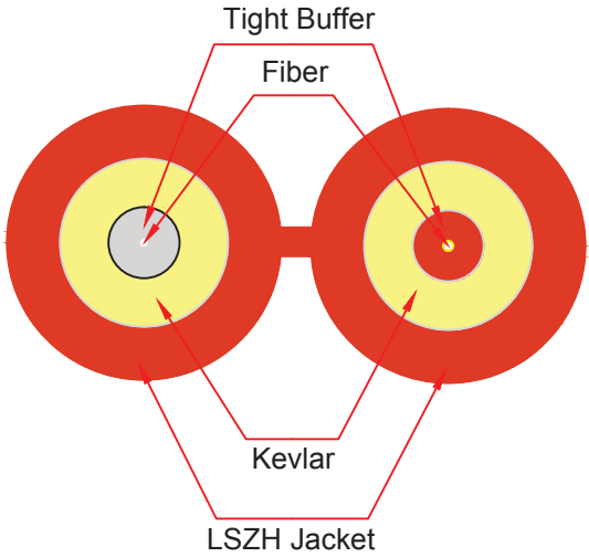
Cable Profile View
