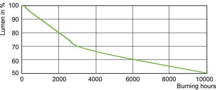
Lumen Maintenance Diagram - MH 175W/640 E40 CL U 1SL/12
