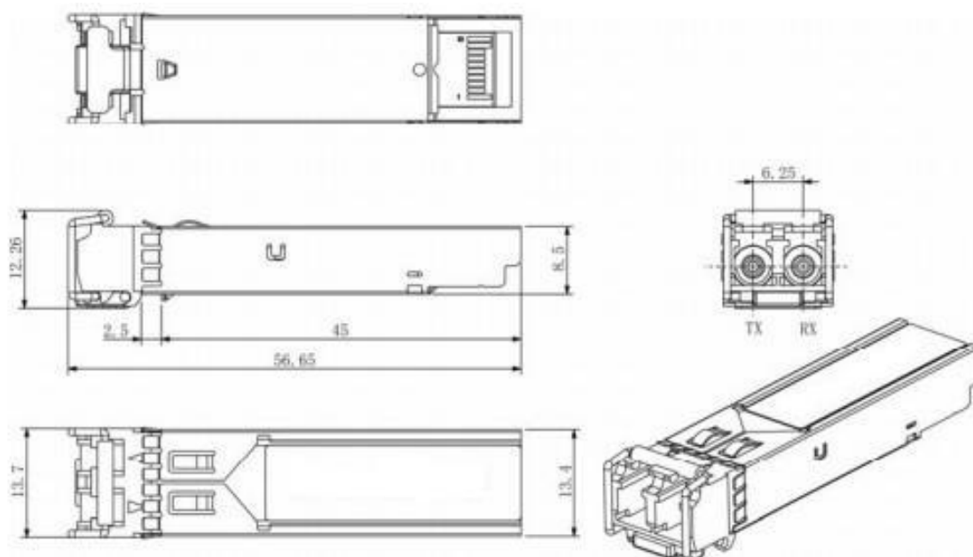
Mechanical Drawing
