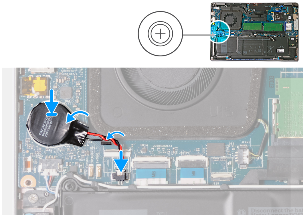
Figure 29. Installation de la pile bouton
