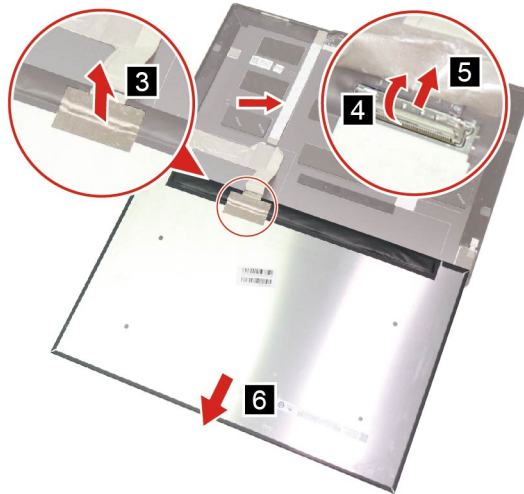
Figure 49. Disconnect the EDP cable and remove the LCD panel
