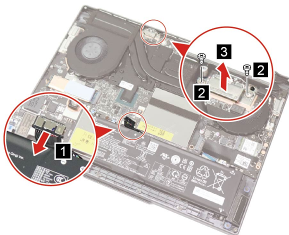
Figure 25. Disconnect the battery pack cable, remove two screws, and remove the HDMI bracket
