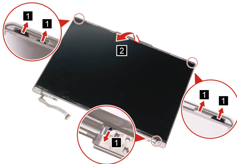
Figure 48. Pull out five pieces of removable tape
