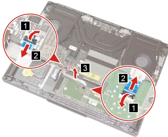
Figure 16. Disconnect and remove the touchpad cable
