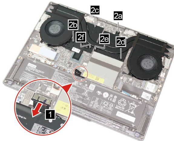
Figure 27. Disconnect the battery pack cable and loosen six screws
