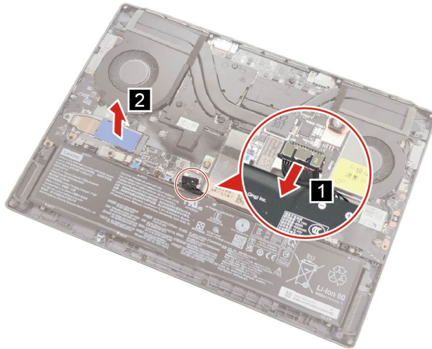
Figure 12. Disconnect the battery pack cable and remove the 2242 SSD thermal pad
