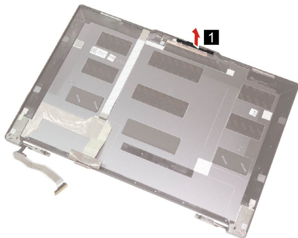
Figure 51. Remove the camera shutter
