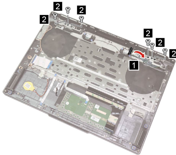
Figure 44. Remove six screws and lift the EDP cable
