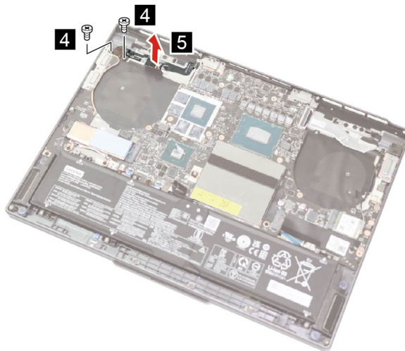
Figure 30. Remove two screws and the fingerprint sensor module
