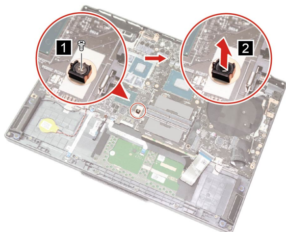
Figure 37. Remove one screw and the system board hook
