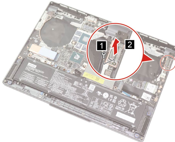
Figure 36. Remove one screw and the USB-A bracket
