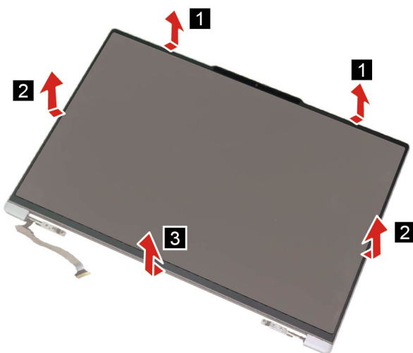
Figure 46. Lift and remove the LCD bezel
