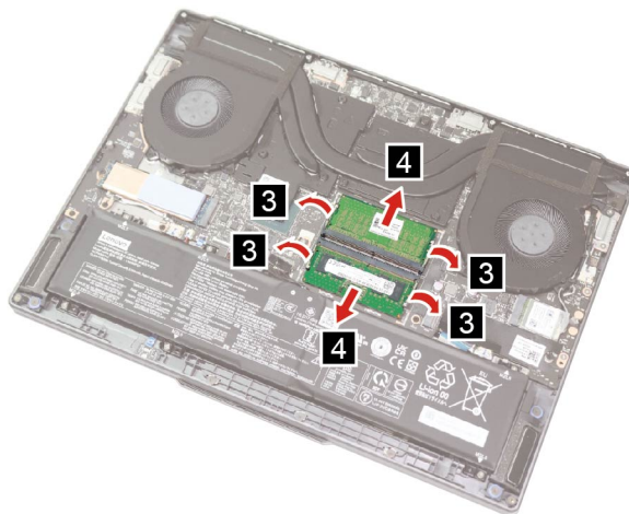
Figure 8. Remove the memory modules
