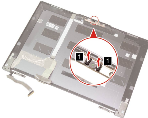
Figure 53. Remove the IR sponges
