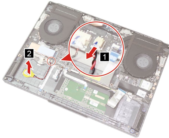
Figure 19. Remove the coin-cell battery
