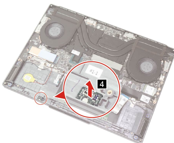
Figure 18. Remove the Hall sensor board
