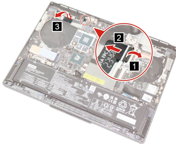
Figure 29. Disconnect the fingerprint sensor connector and lift the mylar
