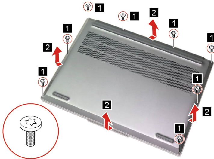
Figure 5. Remove eight screws and the lower case
