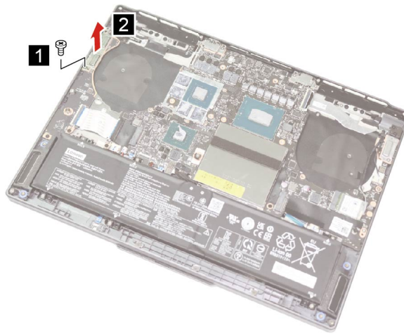
Figure 33. Remove one screw and the I/O board bracket
