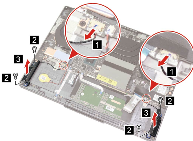
Figure 20. Disconnect the woofer cables and remove the woofers
