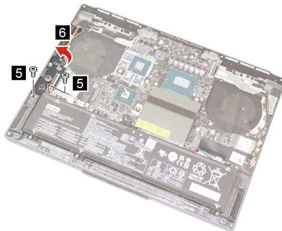
Figure 35. Remove two screws and the I/O board
