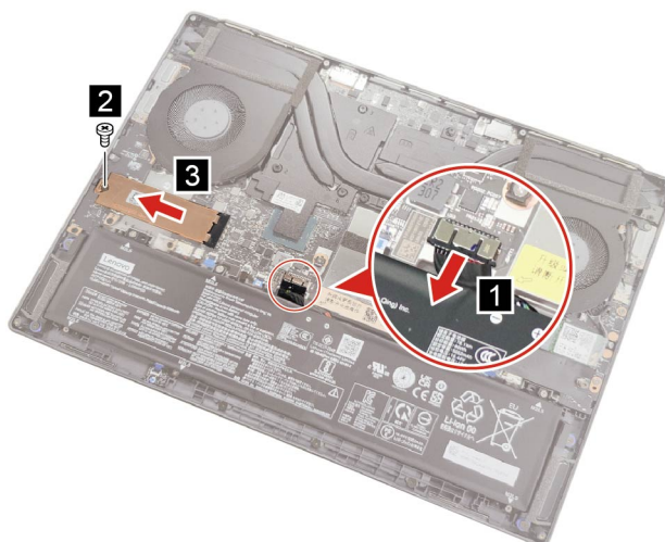
Figure 9. Disconnect the battery pack cable and remove one screw and the 2280 SSD module
