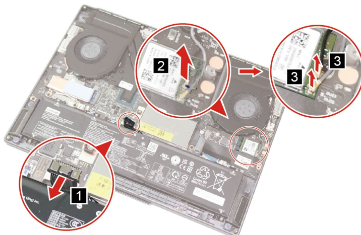
Figure 23. Disconnect the battery pack cable, peel off the Wi-Fi card mylar and disconnect the Wi-Fi antennas
