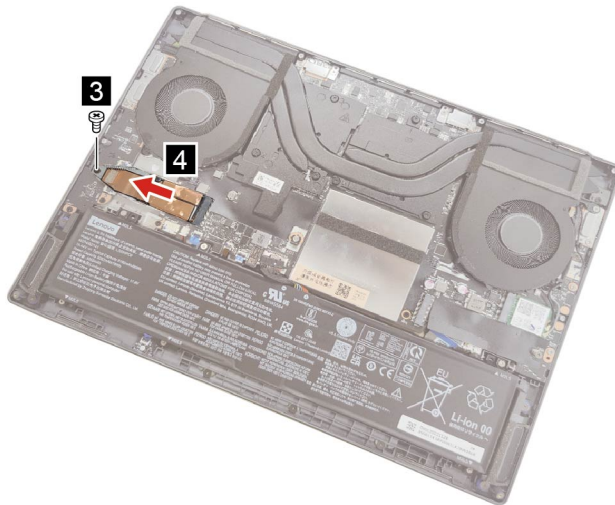
Figure 13. Remove one screw and the 2242 SSD module
