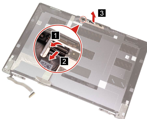
Figure 54. Disconnect the camera cable and remove the camera board
