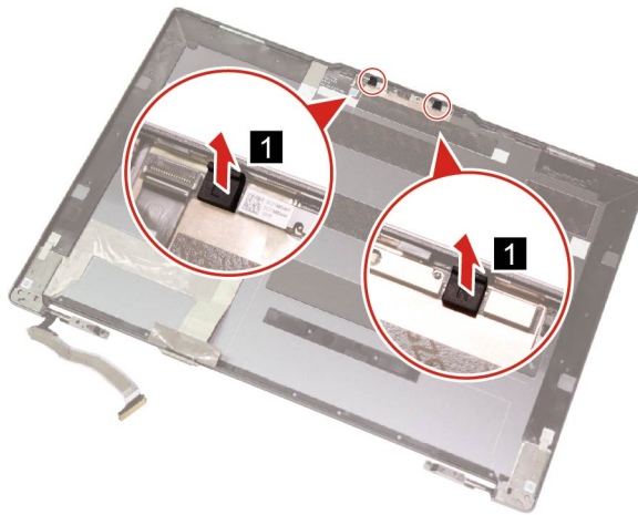
Figure 52. Remove the microphone rubbers
