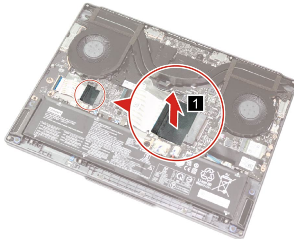
Figure 31. Peel off the I/O board connector mylar
