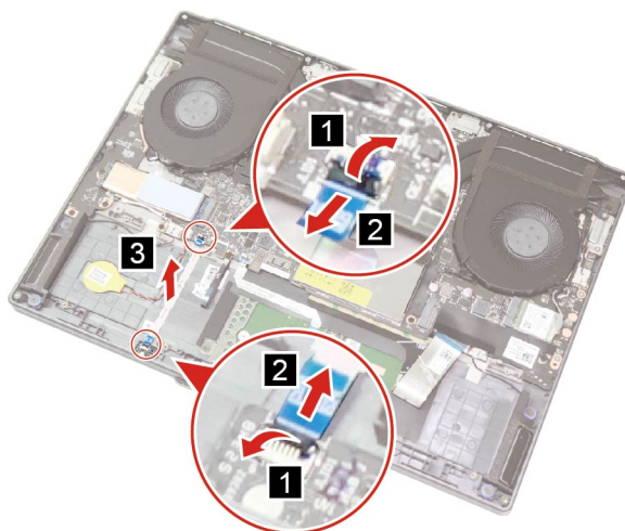
Figure 17. Remove the Hall sensor board cable
