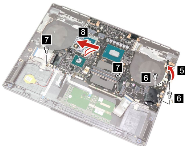
Figure 39. Release the antennas and cable, remove four screws and remove the system board
