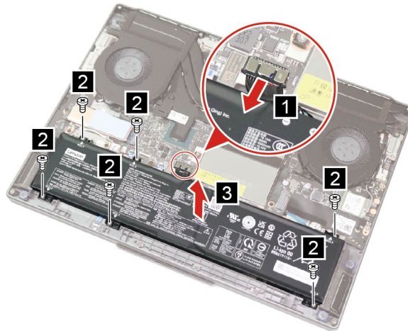
Figure 6. Remove six screws and the battery pack
