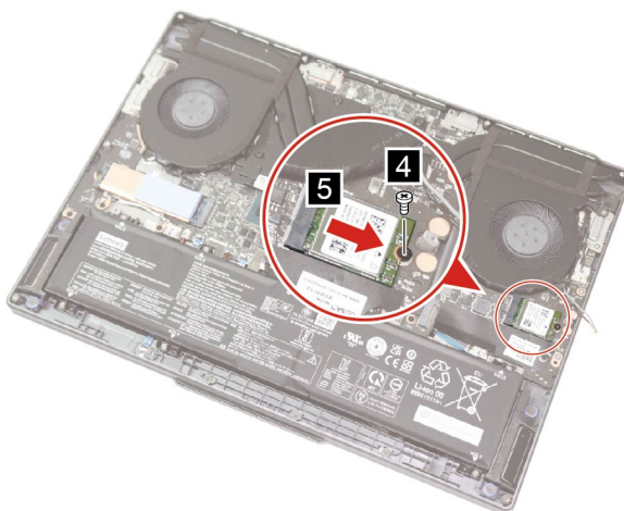
Figure 24. Remove one screw and the Wi-Fi card
