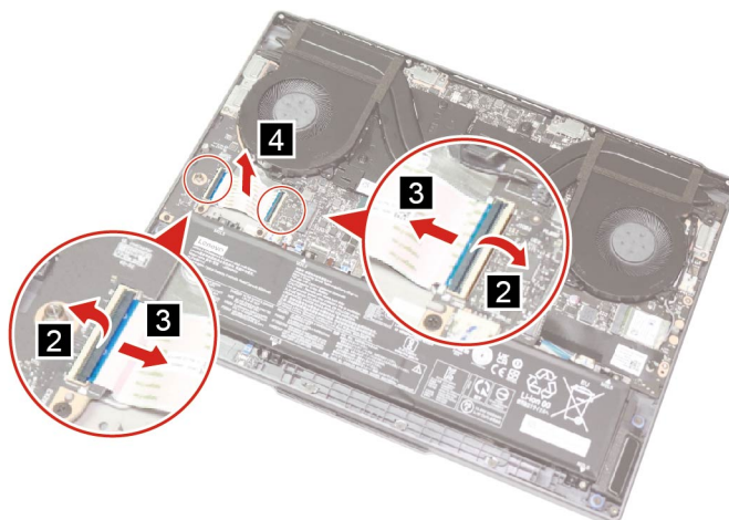
Figure 32. Disconnect and remove the I/O board cable
