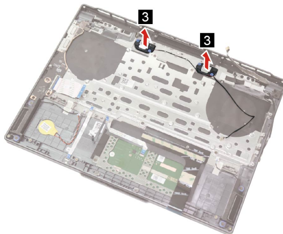
Figure 22. Remove the tweeters
