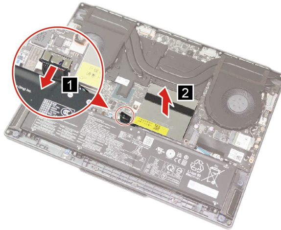
Figure 7. Remove the memory shielding
