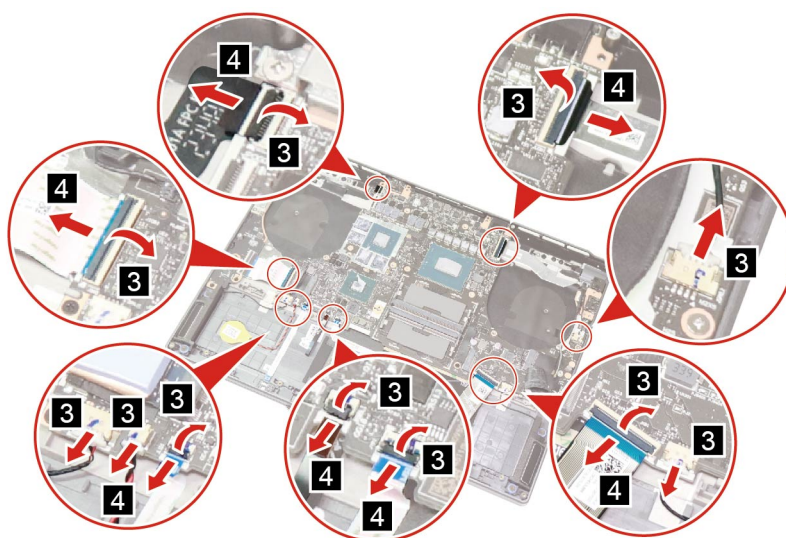
Figure 38. Disconnect all the cables from the system board
