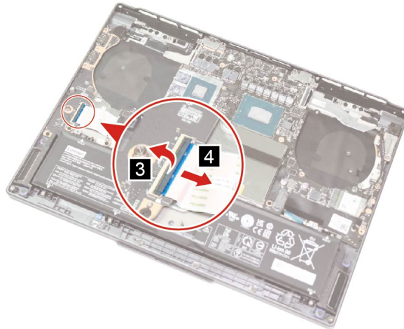
Figure 34. Disconnect the I/O board cable
