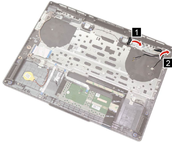
Figure 21. Lift the EDP cable and release the tweeters cable
