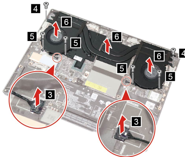
Figure 28. Disconnect the fan cables, remove six screws and remove the thermal module
