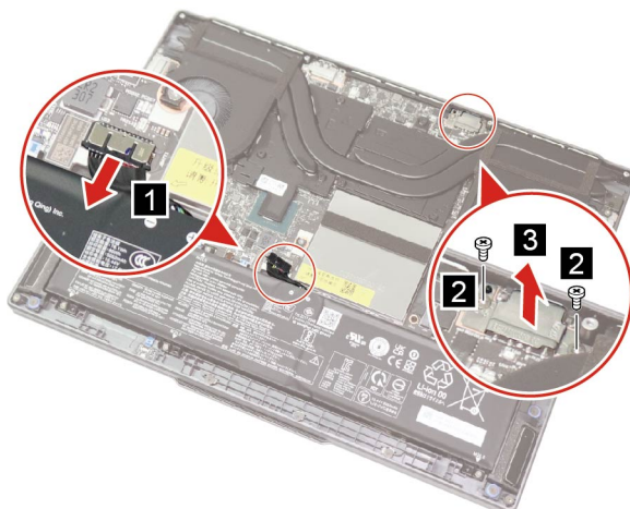
Figure 26. Disconnect the battery pack cable, remove two screws and remove the DC-in bracket
