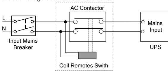
Fig. 1: Typical external isolating device installation
