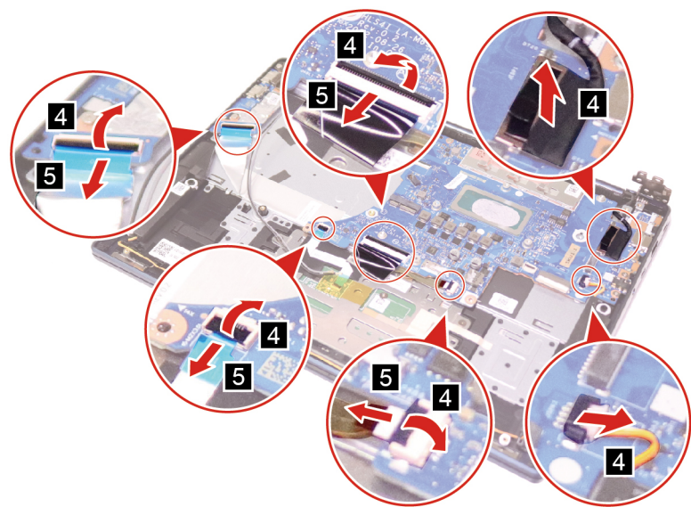
Figure 37. Disconnect cables
