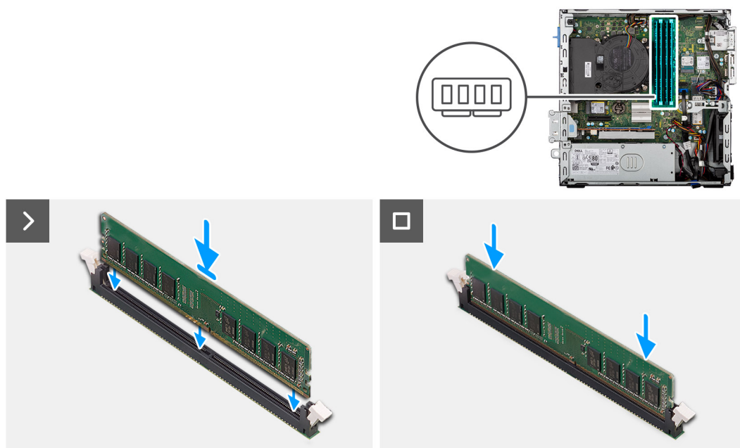
Figure 16. Installation de la mémoire
