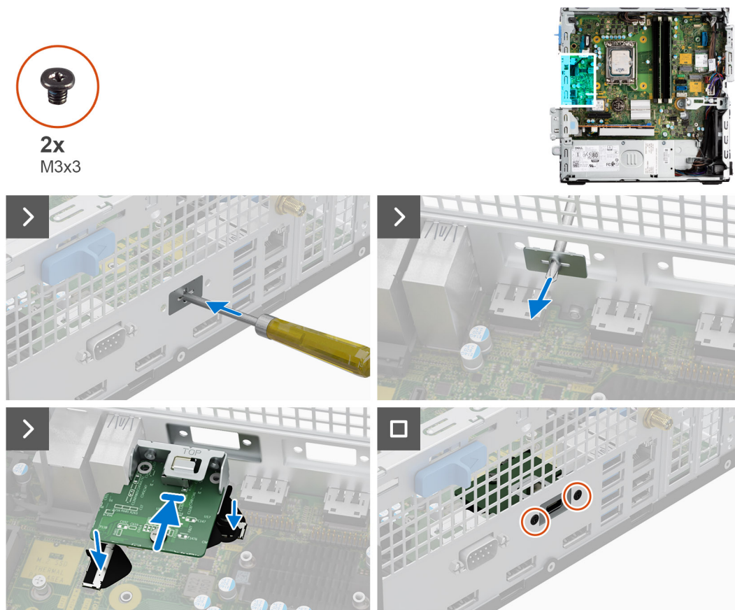
Figure 63. Installation du module USB-C
