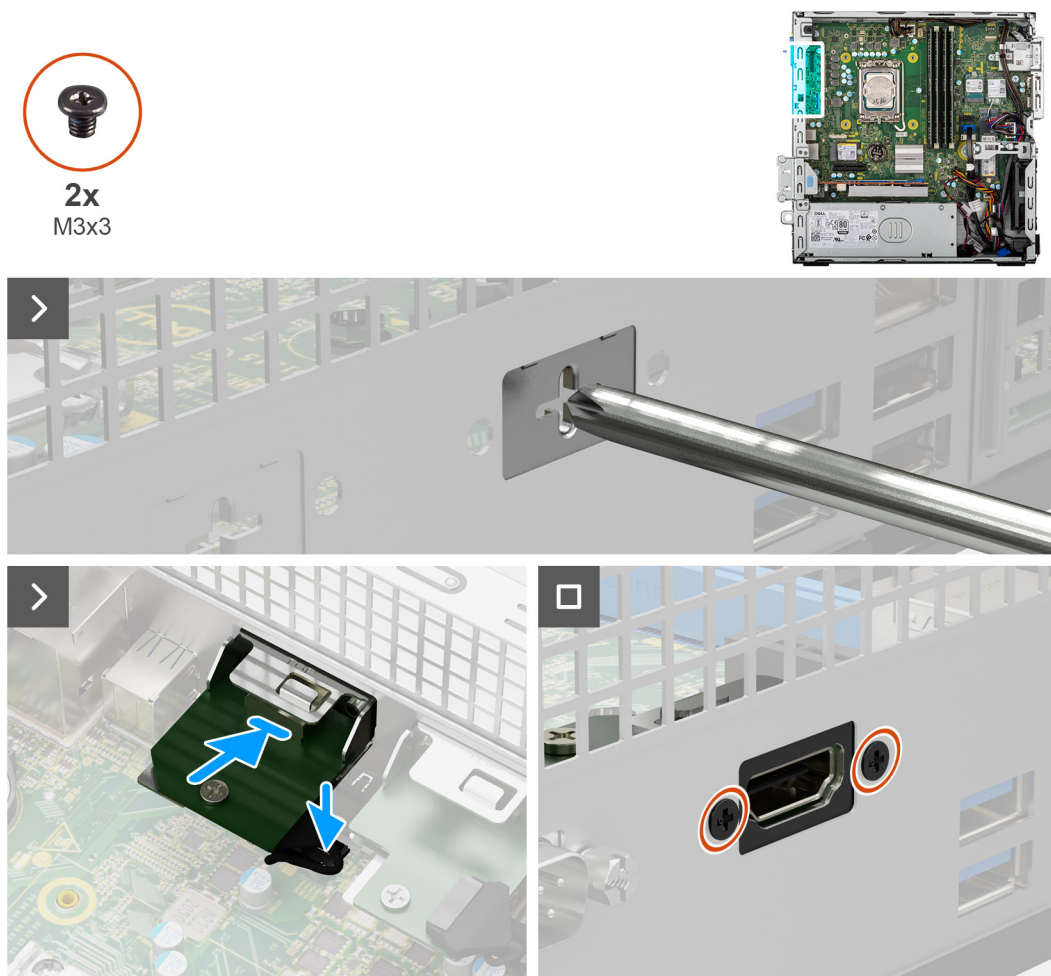
Figure 59. Installation du module HDMI
