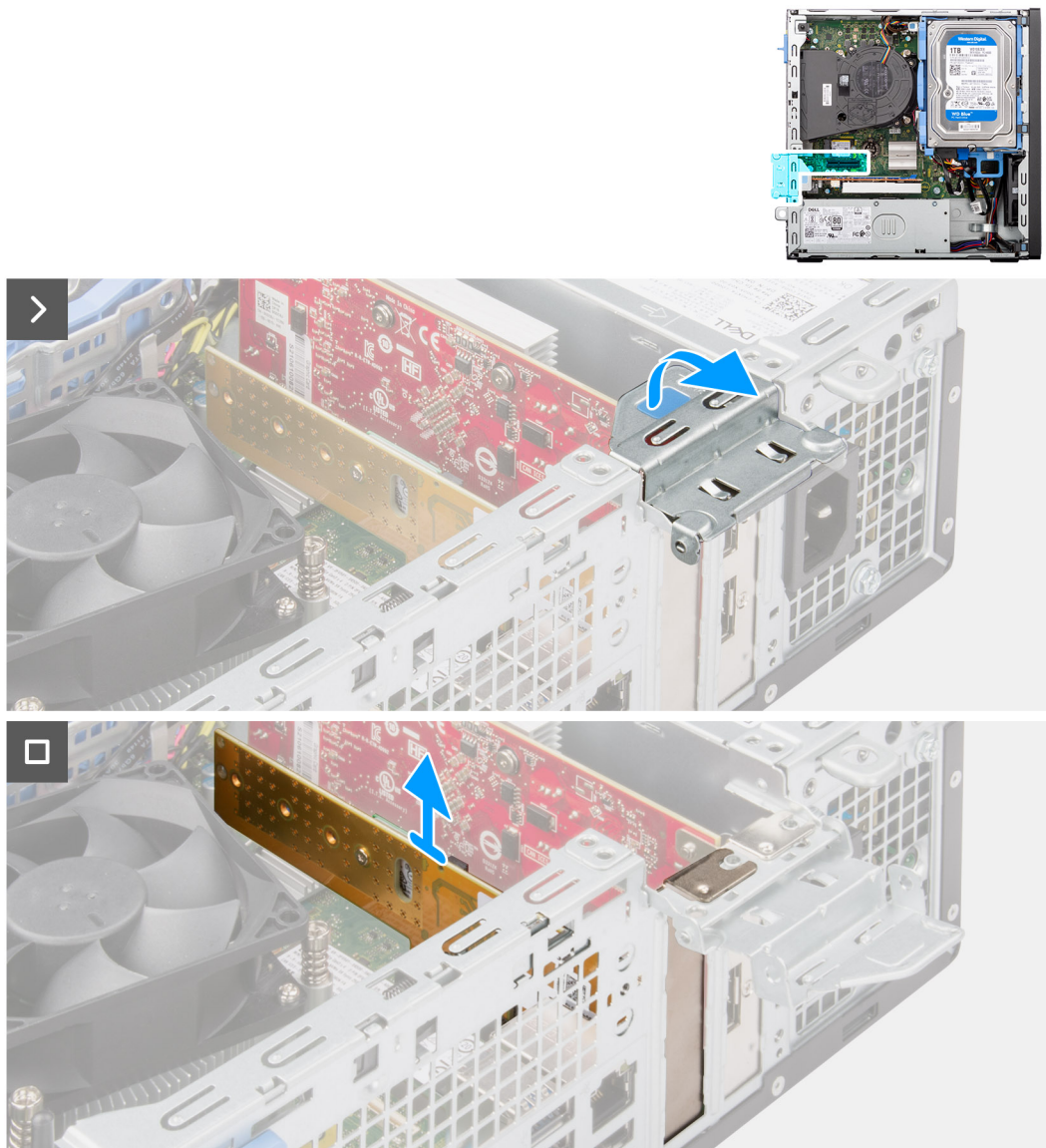
Figure 23. Retrait de la carte Dell Ultra Speed Drive Gen 3
