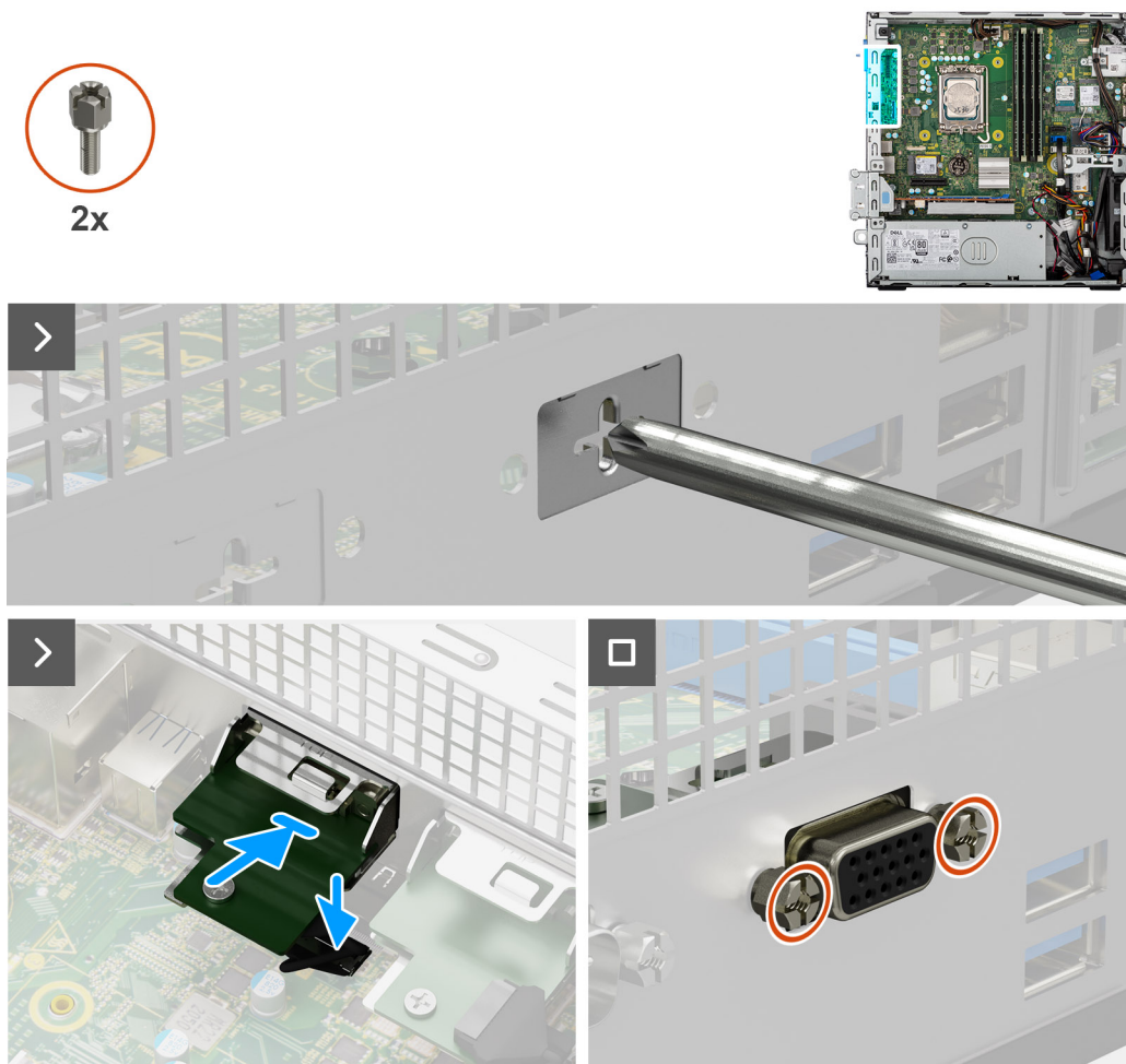
Figure 61. Installation du module VGA
