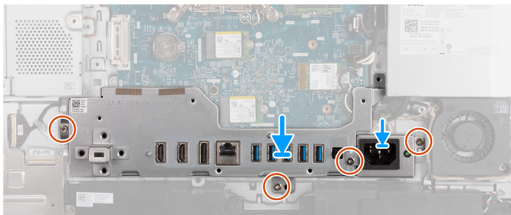
Figure 58. Installation du support d'E/S
