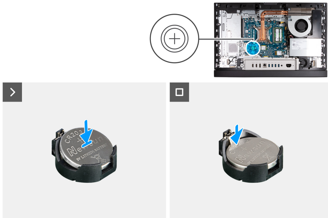
Figure 40. Installation de la pile bouton
