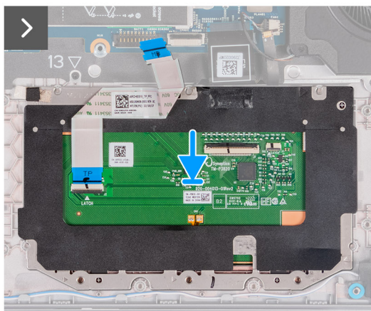
Figura42. Instalar o touchpad
