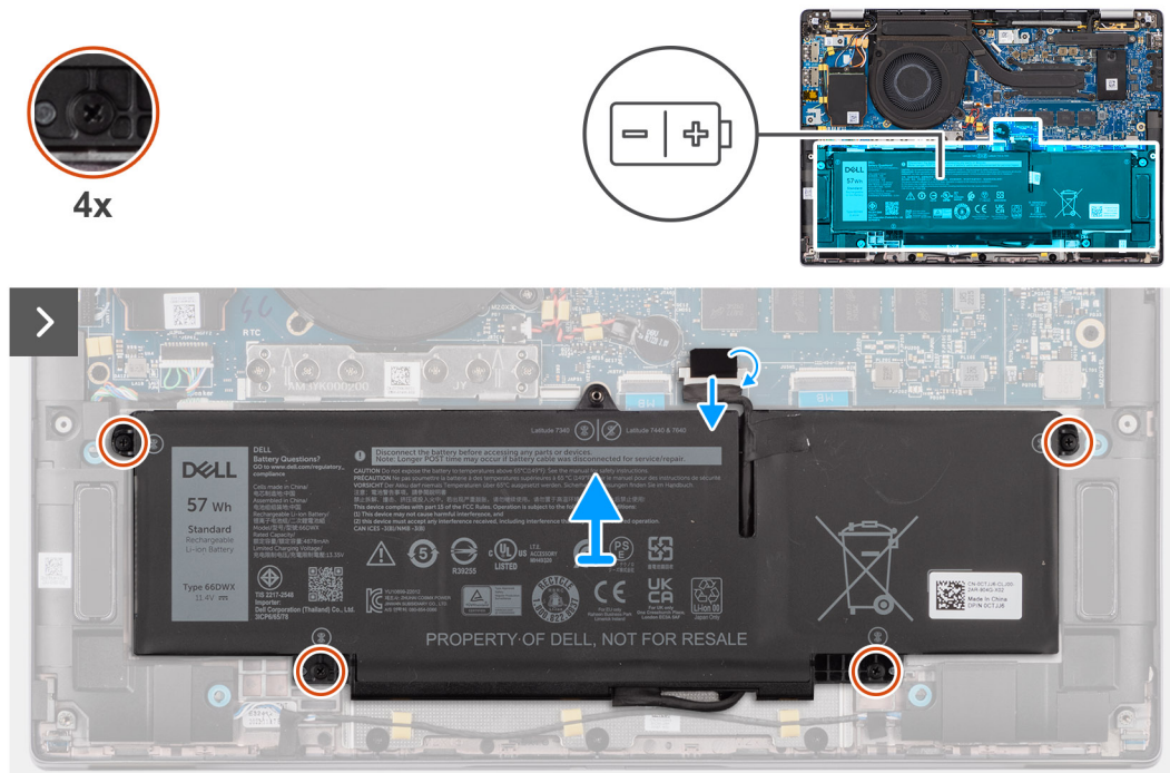
Figur 40. Ta bort 3-cellsbatteriet
