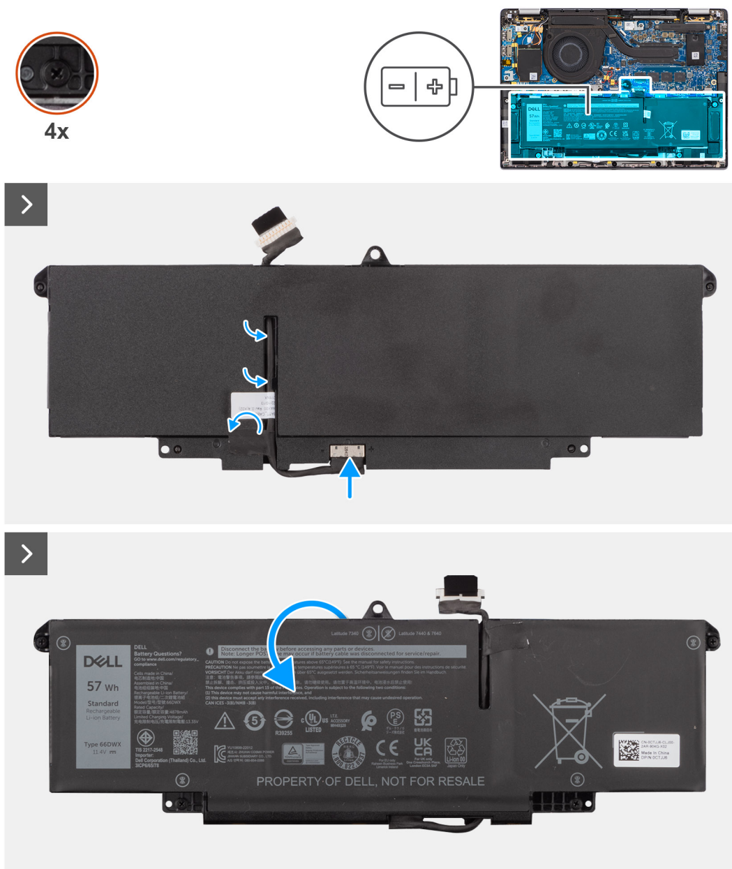
Figur 42. Installera 3-cellsbatteriet
