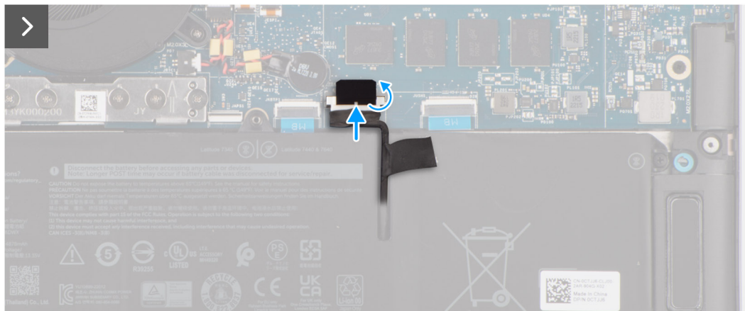
Figur 19. Installera kåpan
